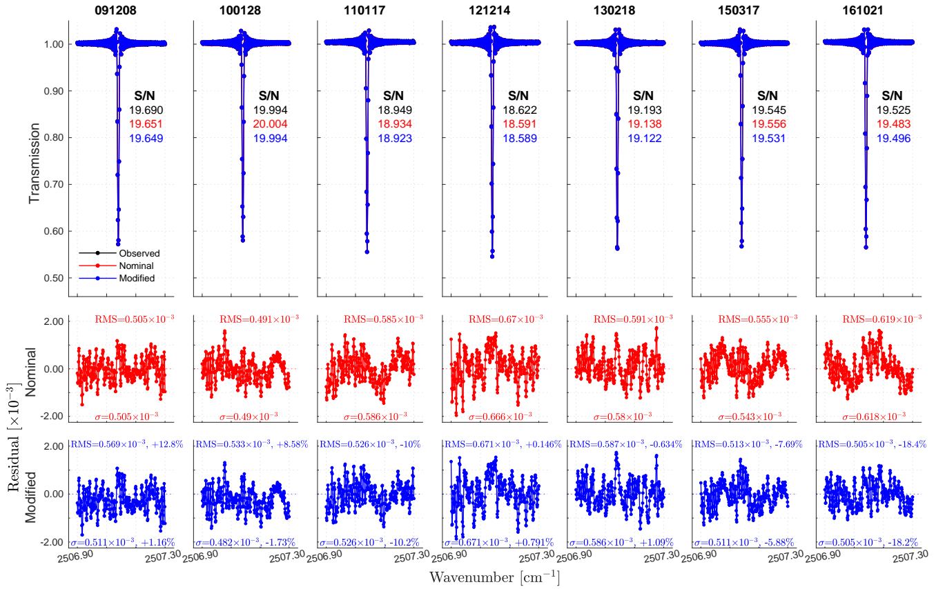
Figure 14. The top row shows the P(2) iside lobe line of the HBr transmission spectrum, showcasing observed , fitted, and reconstructed spectra across different dates. The middle and bottom rows show residual plots comparing the deviations before and after fitting, respectively.
