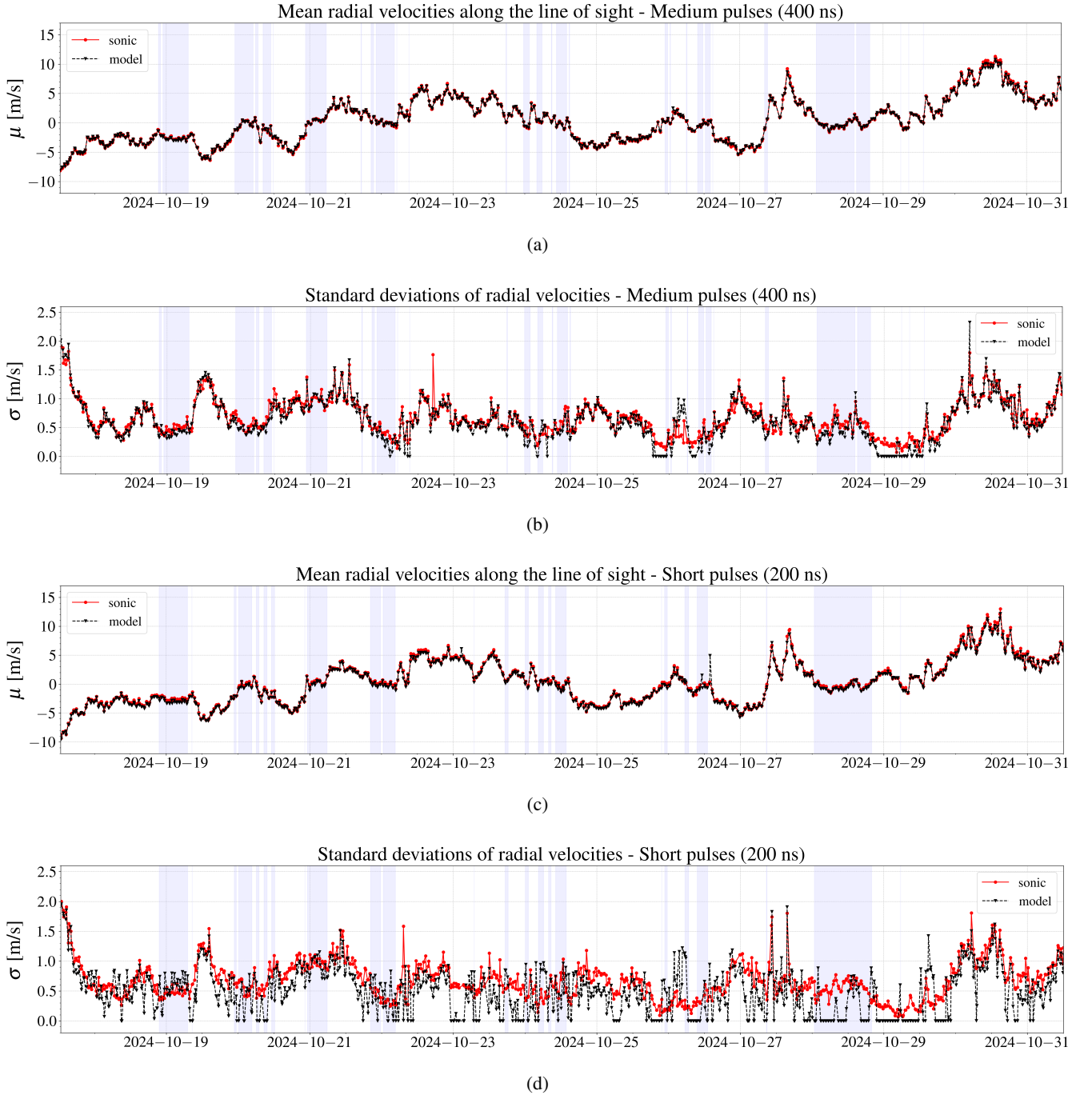
Figure 6. The time series for the 10-minute average radial wind velocities (a) and standard deviations (b), obtained from the model (black triangles), are based on power spectral density from the instrument’s 400 ns pulses. Similar plots for the 10-minute average radial wind velocities (c) and standard deviations (d) are derived using 200 ns pulses. Each of these quantities is compared to the corresponding values from the projected velocity of the sonic anemometer along the lidar beam direction (red circles). The wake sector is shown as a shaded area.
