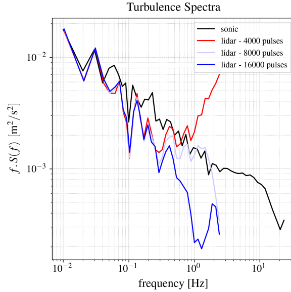
Figure 1. Turbulence spectra derived from the 10-minute radial velocity time series using pulsed lidar without additional averaging (red curve) and a sonic anemometer (black curve). The light and dark blue curves illustrate turbulence spectra obtained from moving averages of the Doppler spectra calculated over two and four times the original number of pulses.
