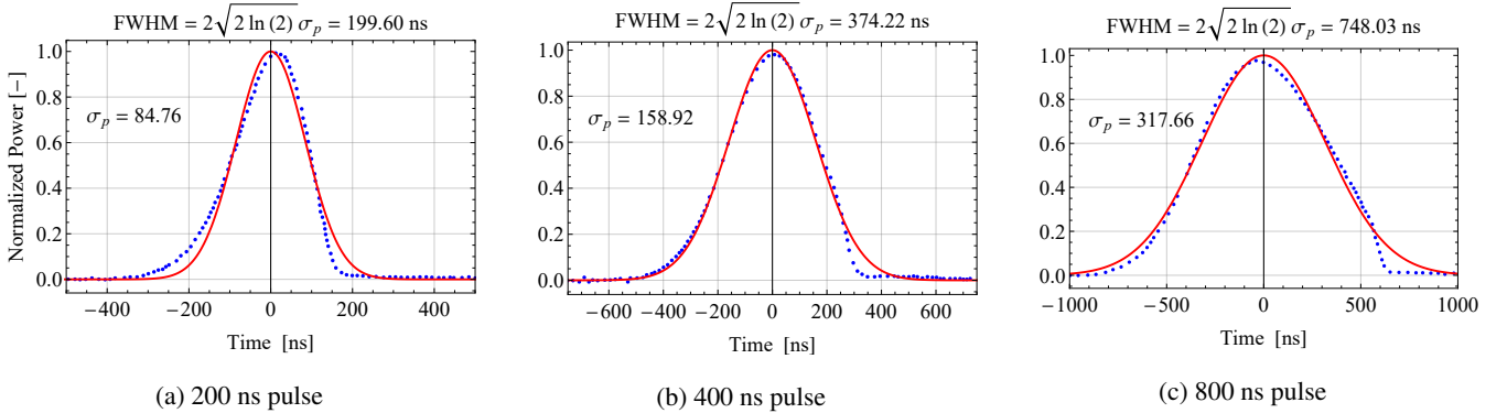
Figure 2. Measured laser power over time (blue points) with Gaussian fits (red curves) approximating the pulse shapes. Each pulse is normalized to its peak power.
