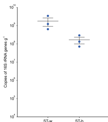
Figure 6: Quantification of the prokaryotic cell biomass present in ST-w and ST-b through qPCR targeting the 16S rRNA gene. The abundance is expressed as number of copies of 16S rRNA per gram of sample.
