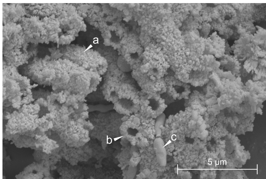
Figure 2: SEM/FESEM image of a sample collected from the white paste of a silica stromatolite-like formation in Imawarí Yeutá. Arrows indicate a) botryoidal masses of precipitated amorphous silica, b) the section of a tubular cast, c) a bacterium-like structure
