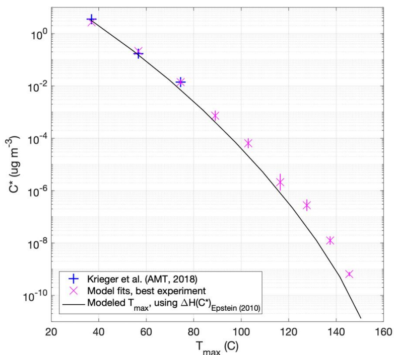
Figure S3: Markers present saturation vapour concentrations C^* for PEGs, at 298 K, using datasets and colour coding as described in Figs. S1 and S2, versus the T_{\max} as obtained during the best-fitting experiment
