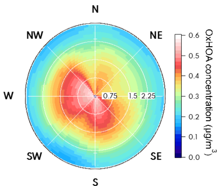
Figure S15. Non-parametric wind regression plot of OxHOA factor (zoomed), x-axis indicates wind intensity in m/s.
