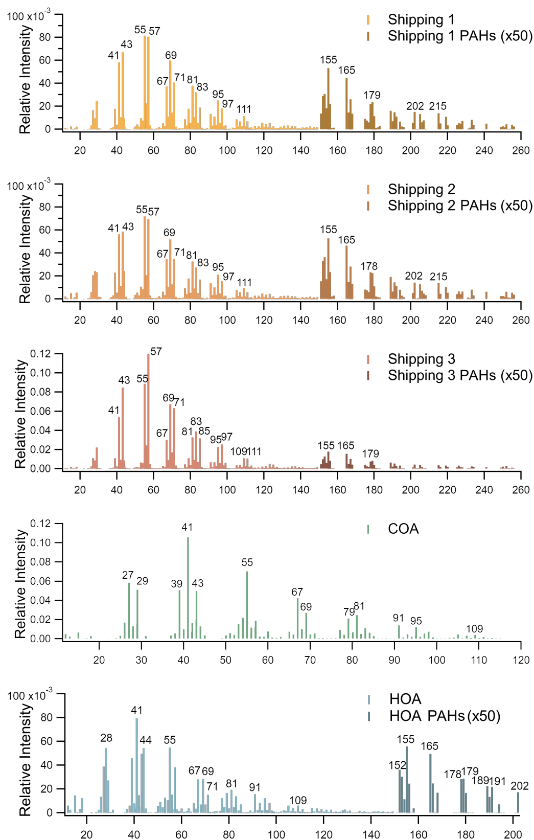
Figure S6. Reference mass spectra used as constraints for PMF analysis. Ions with m/z ratio superior to 150 have their relative intensity multiplied per 50 to enhance readability. X-axis represents m/z ratios.
