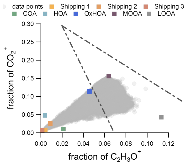
Figure S14. Fraction of \text{CO}_2^+ vs. fraction of \text{C}_2\text{H}_3\text{O}^+ . Dashed lines represent the limits of Ng et al. (2010)'s triangle. Factors are subtracted from total contribution.
