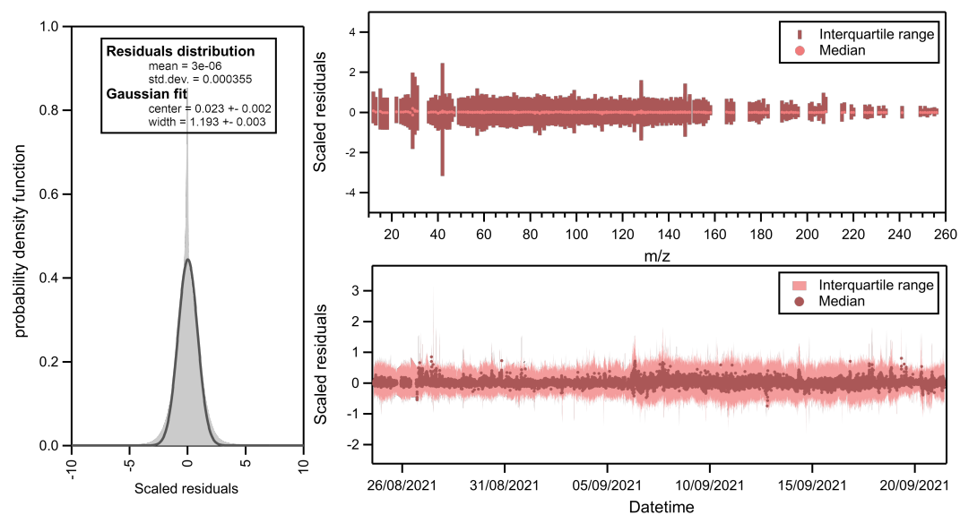
Figure S7. Scaled residuals distribution fitted by a Gaussian curve (a). Median scaled and interquartile range for the solution over m/z profile (a) and time (b).
