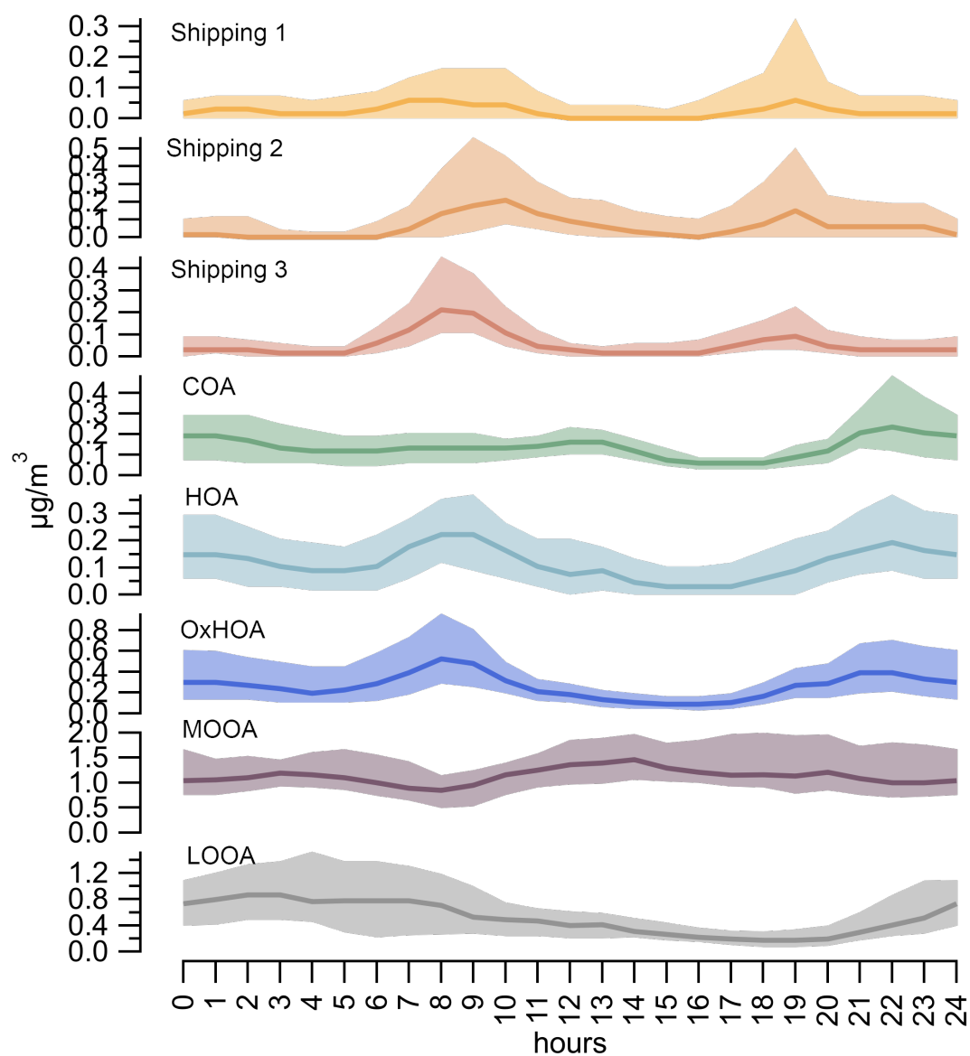
Figure S11. Diurnal variation of the PMF factors.
