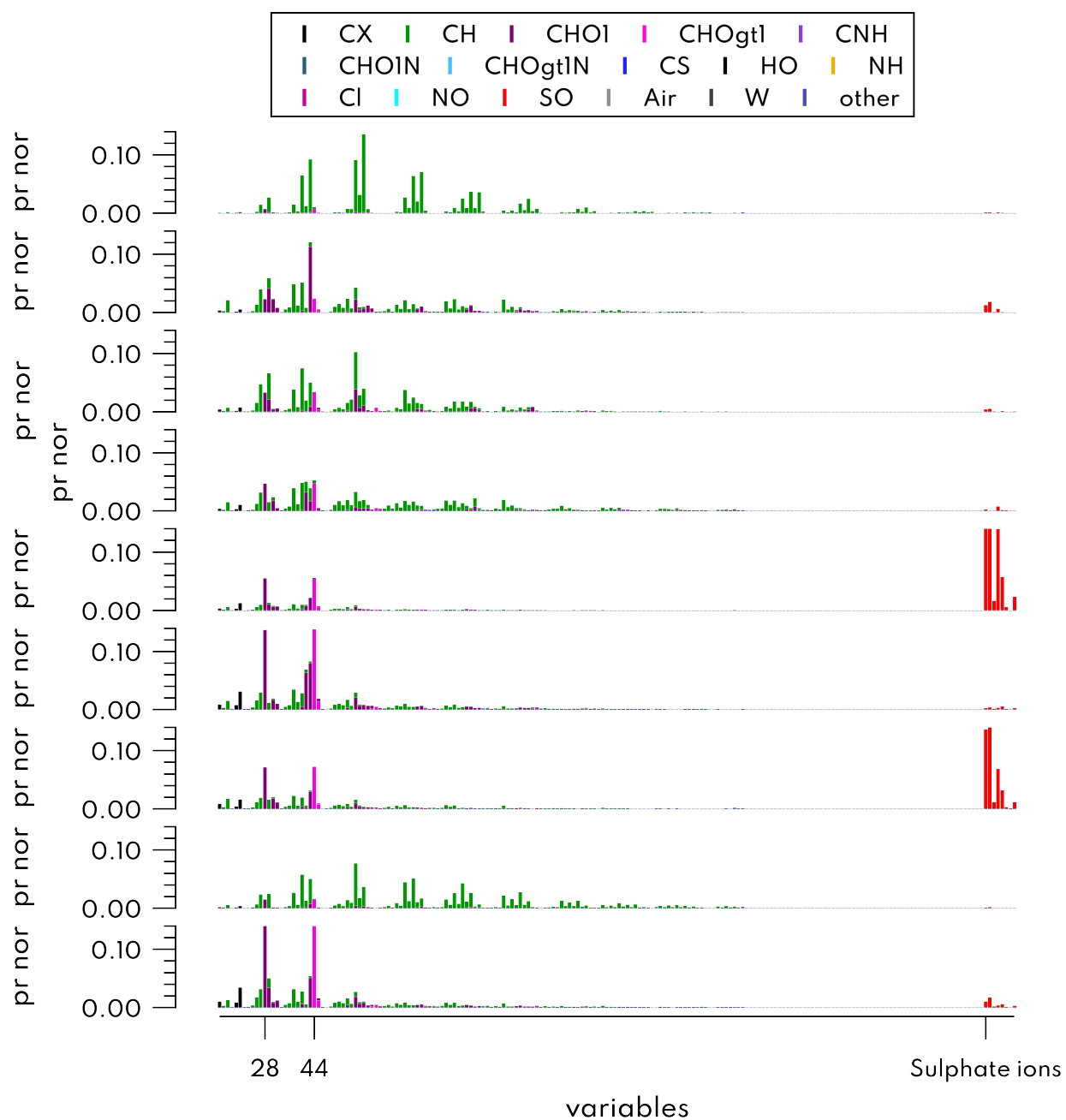
Figure S5. Mass spectra of the 9-factors PMF solution with sulfate ions added.
