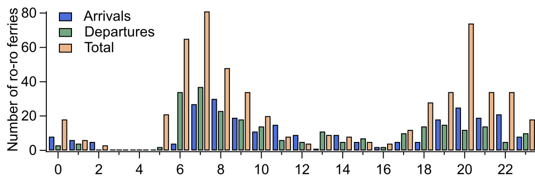
Figure S3. Hourly distribution of arrivals and departures of ro-ro ferries recorded by the harbor authority.
