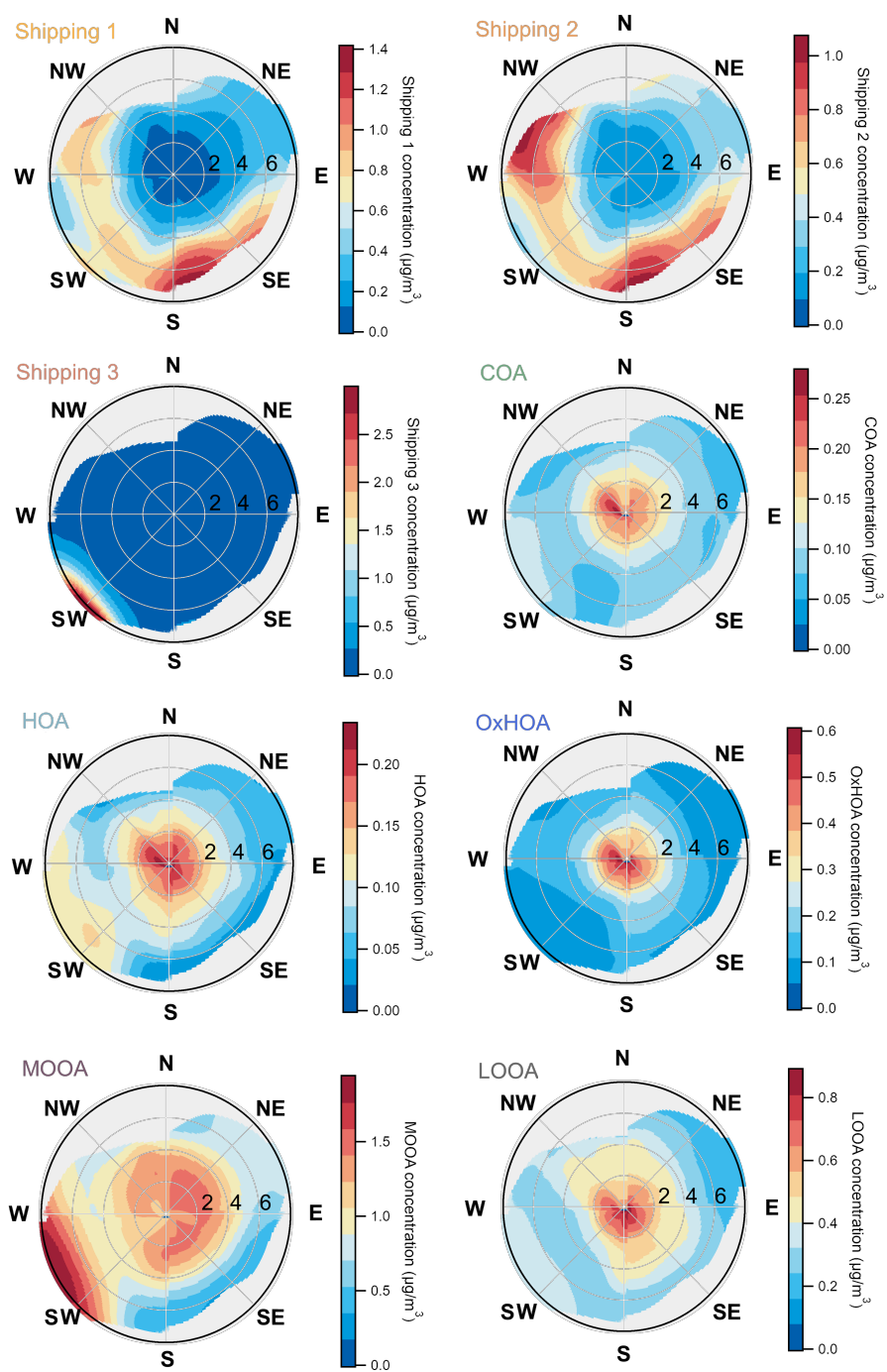
Figure S10. Non-parametric wind regression (NWR) plot of PMF factors, x-axis indicates wind intensity in m/s.
