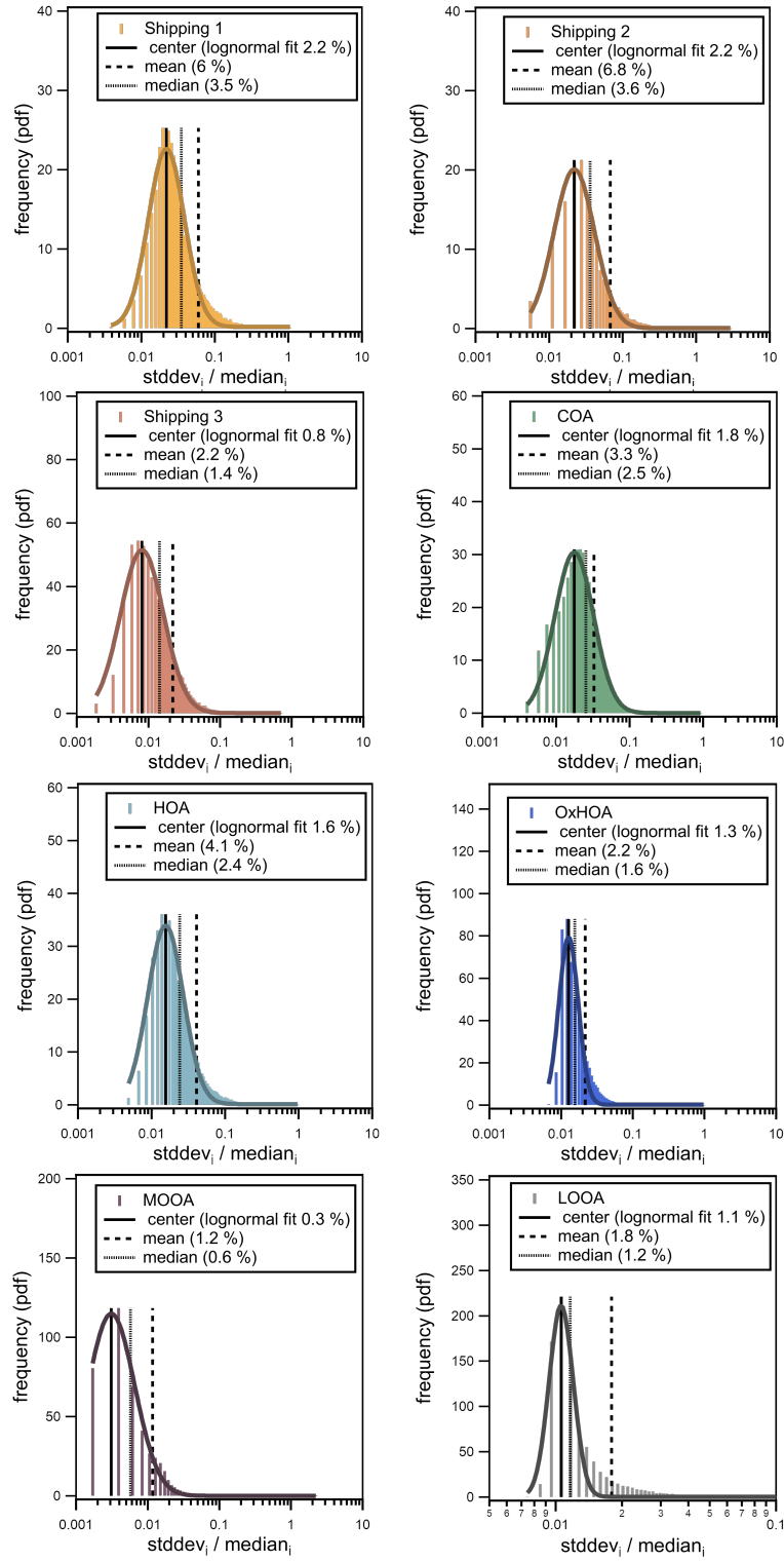
Figure S8. PMF error estimation for each factor, the center of the lognormal fit corresponds to the uncertainties of the factor.
