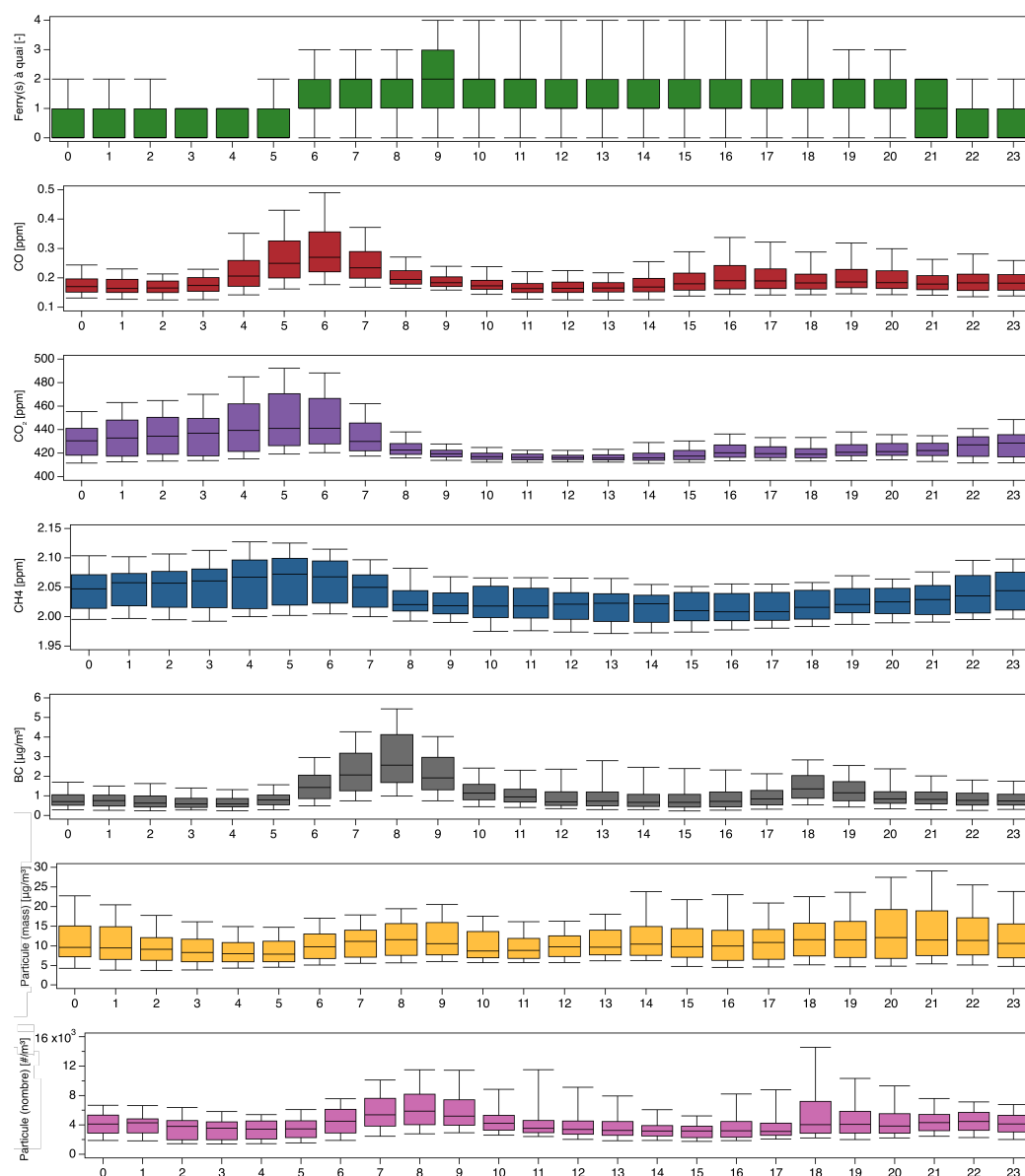
Figure S4. Diurnal distribution of CO, CO 2 , CH 4 , BC, PM and PN during the campaign.
