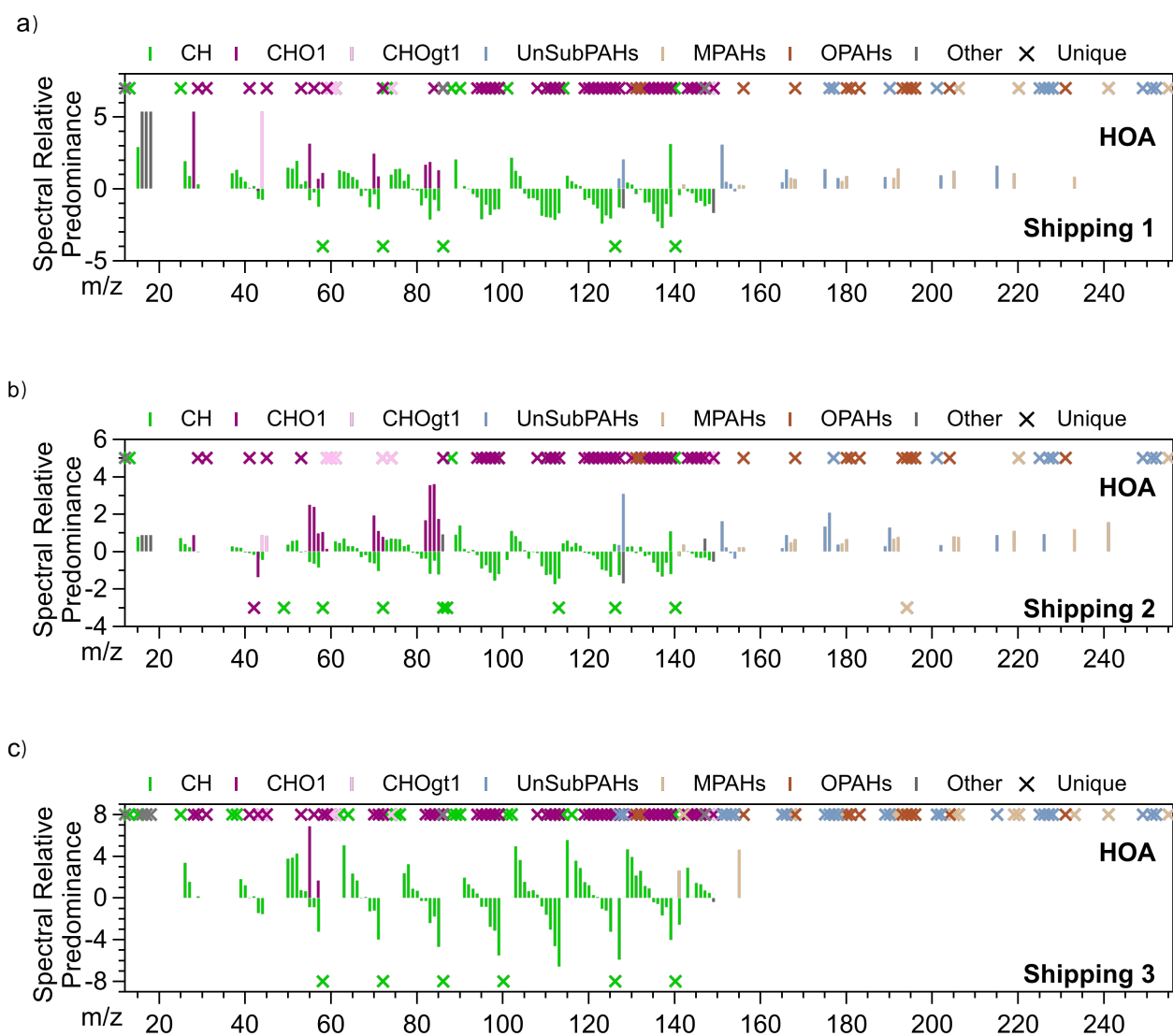
Figure S12. Spectral Relative Predominance (SRP) of HOA factor (positives SRP) with shipping factors 1 (a), 2 (b) and 3 (c) (negatives SRP). Ions whose intensity are below their median error are considered zero. Cross markers represents ions that are null intensity in the other factor. Ions are family-colored.
