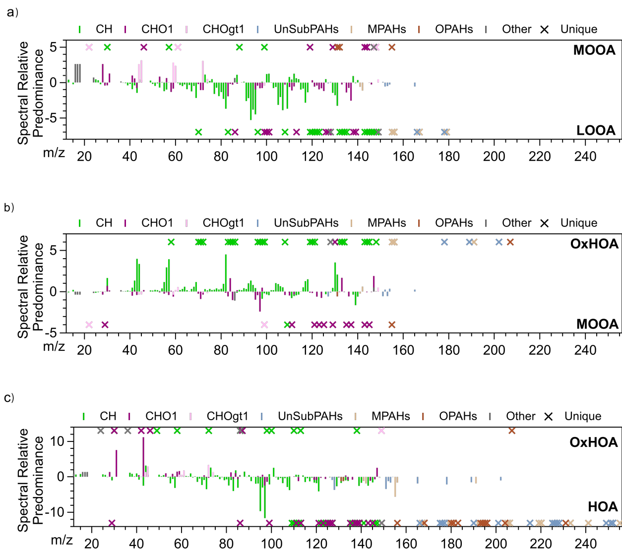
Figure S13. Spectral Relative Predominance (SRP) of MOOA factor (positives SRP) with LOOA factor (negatives SRP) (a)) and OxHOA factor (positives SRP) with MOOA (b)) and HOA factors (c))(negatives SRP). Ions whose intensity are below their median error are considered zero. Cross markers represents ions that are null intensity in the other factor. Ions are family-colored.
