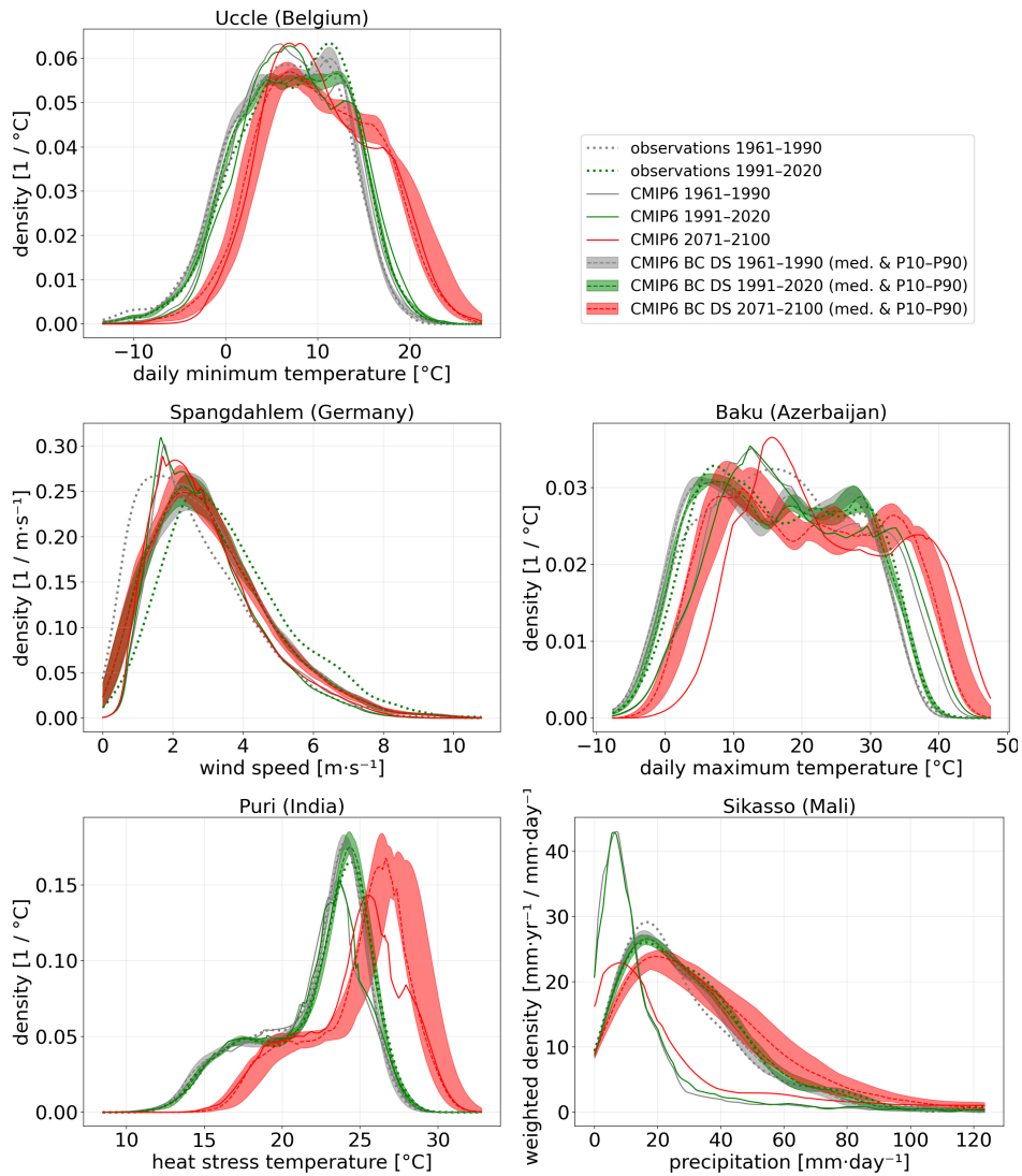
Figure 6. Idem as Fig. 4, but showing results for original CMIP6 climate projections (SSP585) including models listed in Tab. 1, bias-corrected and downsampled CMIP6 models (CMIP6_BC_DS). Observations are also included as comparison. Results are shown for two historical time frames 1961–1990 (in grey) and 1991–2020 (green), and for one future timeframe 2071–2100 (in red). For CMIP6_BS_DS, we show the 10-to-90 percentile spread over the different models.
