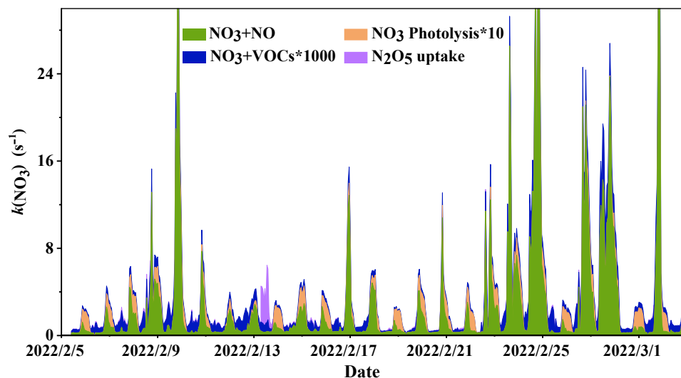
Figure 5. Time series variation of k_{\text{NO}_3} (reactions with NO and VOCs, heterogeneous uptake of N 2 O 5 and photolysis of NO 3 ).
