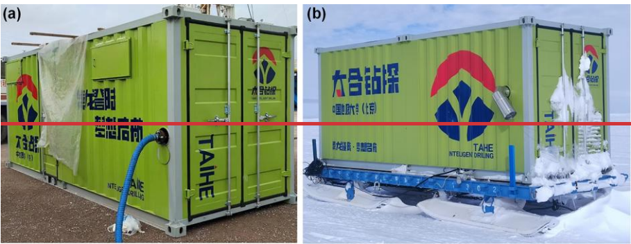
Figure 6: (a) Domestic test and (b) field test of the air system
