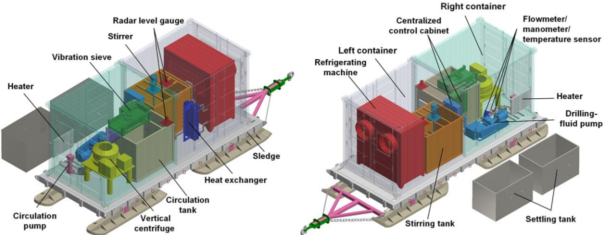
Figure 147: Structure of the DFCS
