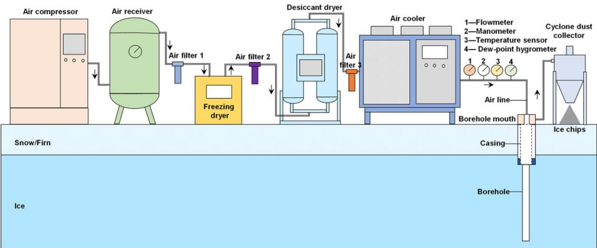
170 Figure 2: Air-system-pPrinciple of the air system
