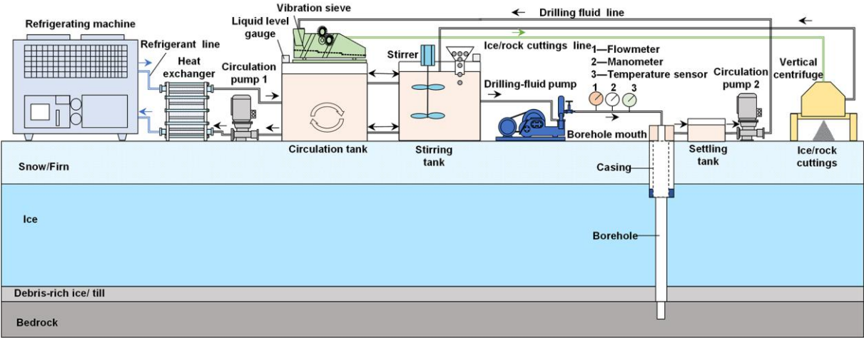
Figure 95: Principle of the DFCS
