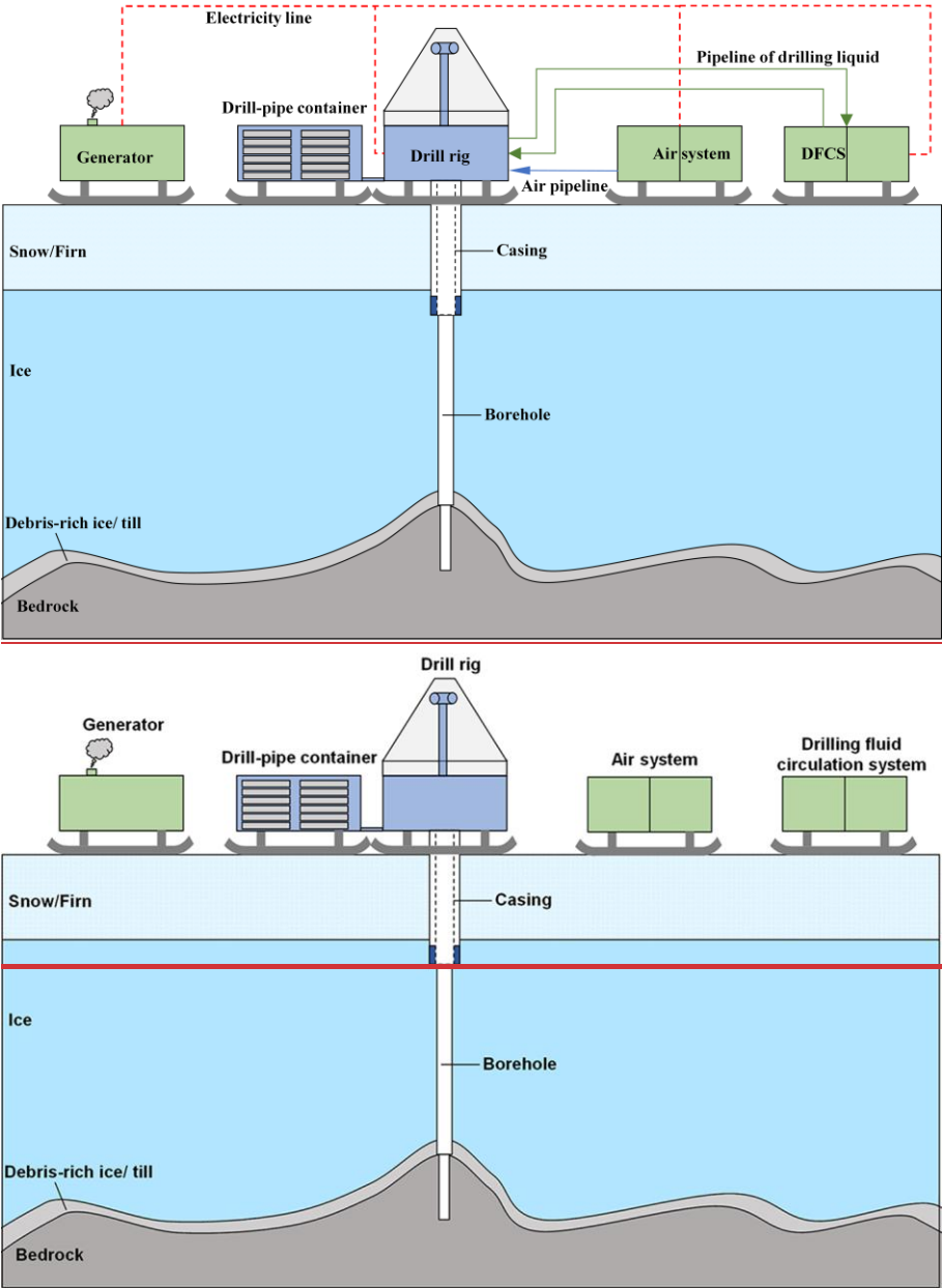
Figure 1: Schematic diagram of the MPDS for subglacial bedrock sampling in Antarcticapolar regions
