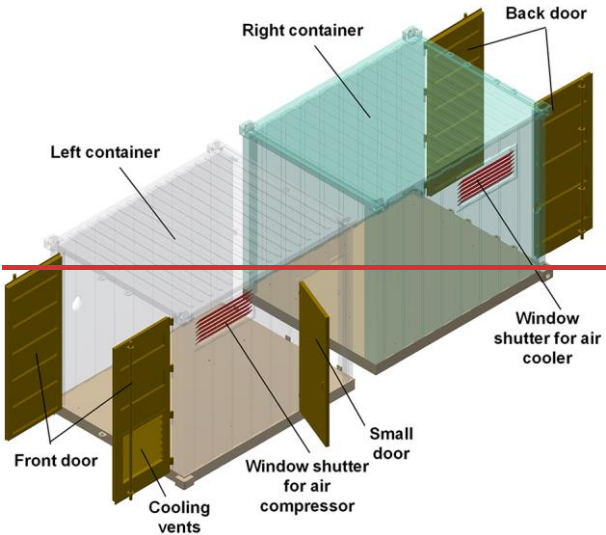
Figure 5: Modified container of the air system
