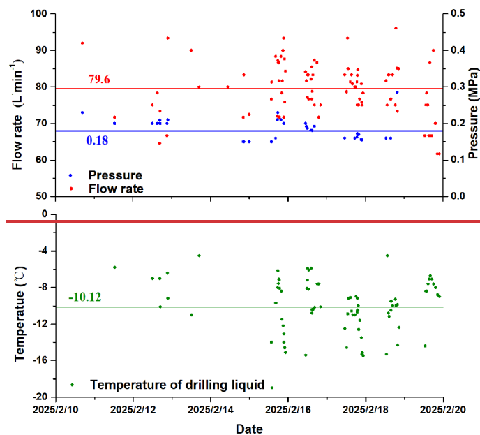
Figure 1410: Test results of the DFCS in Antarctica
