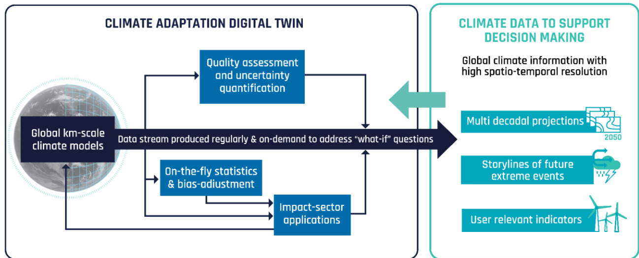
Figure 1: Conceptual diagram illustrating the main Climate DT components. The Climate DT uses data streams from the global high-resolution climate models to feed a range satisfy the requirements of a number of data consumers embedded in the workflow . The data consumers include climate-sensitive applications and a comprehensive monitoring and quality assessment procedure. User feedbacks are regularly incorporated in the Climate DT design (hence the thick arrows pointing in both directions) so that the global information with local granularity produced adequately supports climate adaptation decision-making.
