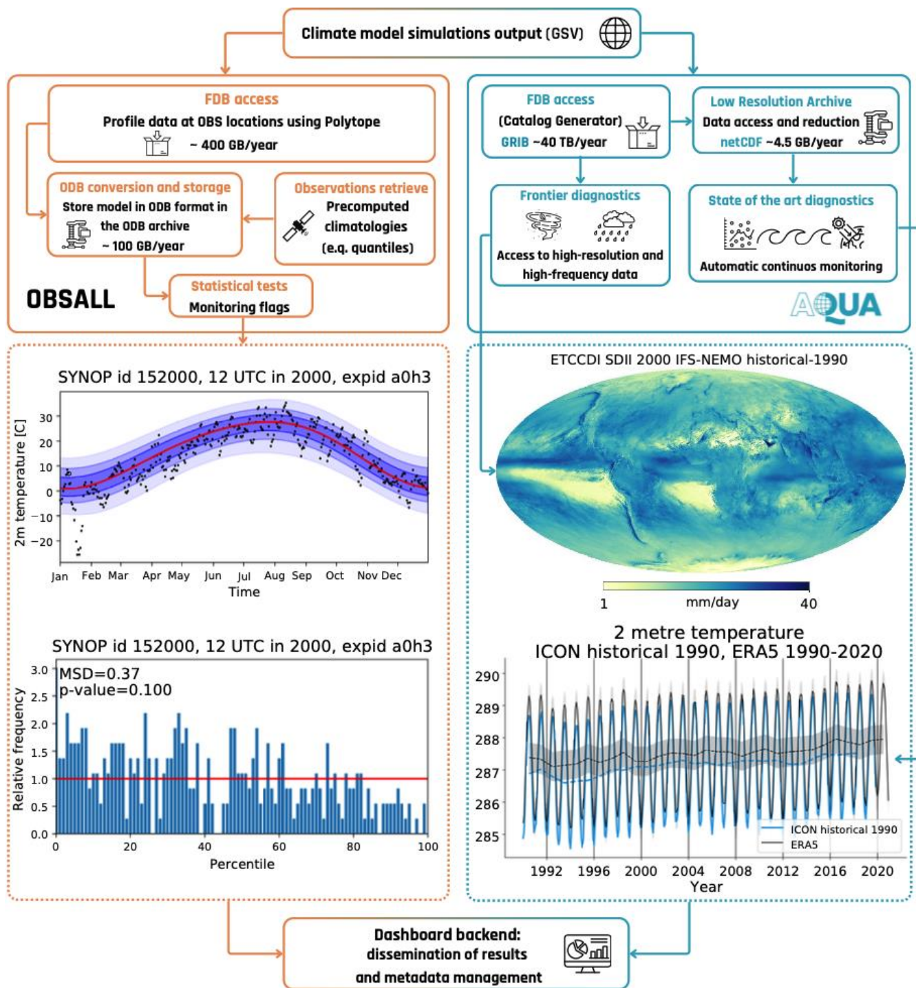
Figure 6: Scientific model evaluation strategy of the Climate DT. The AQUA processing (blue boxes) enables two-way model evaluation through automatically-generated catalogue entries. High-resolution data supports high-granularity frontier diagnostics,
