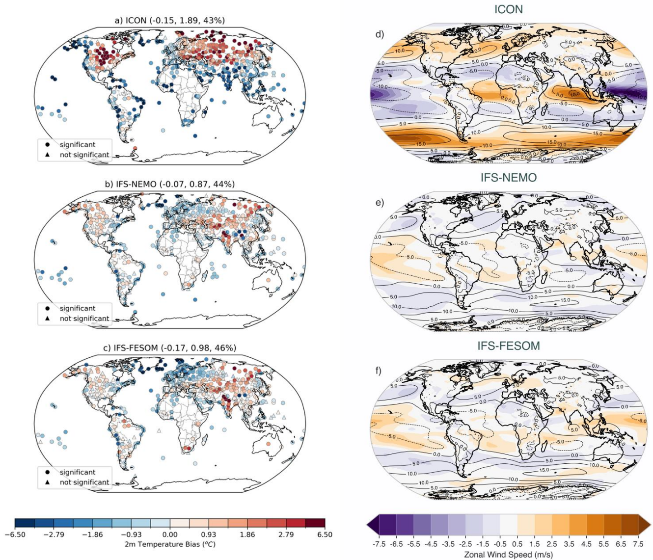
Figure 4: Example of AQUA-OBSALL diagnostics output. (Left column) Bias of annual mean 2-metre temperature (°C) at synoptic surface stations in (a) ICON, (b) IFS-NEMO and (c) IFS-FESOM. Stations where the simulated values differ at the 5% significance level from the observations are represented with closed circles and the rest of the stations with triangles. Values in the headings stand for average bias, average absolute bias, and the fraction of stations with positive bias, respectively. (Right column) 850 hPa zonal mean wind (contour, m/s) and bias against ERA5 (shading, m/s) in (d) ICON, (e) IFS-NEMO and (f) IFS-FESOM. For the three models, climate simulations considered are operational/historical simulations (O25.1). For both simulations and references, the period considered
