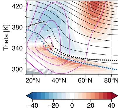
Figure 10. Vertical clear-sky eddy ozone flux in EMAC (winter-mean climatology, DJF 2000–2019), \overline{\hat{Q}_{cs}\rho_{\theta}\hat{\chi}}/\overline{\rho_{\theta}} in units of % K day -1 , approximated by the Newtonian damping approach from Eq. (3) with \alpha = 7 days. Other details as in Fig. 8.
