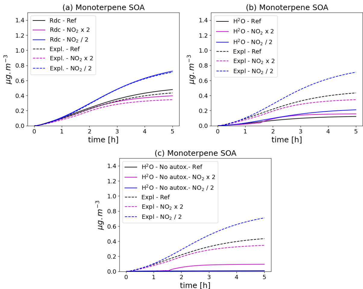
Figure 5. Time evolution of monoterpene SOA mass with different chemical schemes and for different \text{NO}_2 initial concentrations (Ref. denotes the reference \text{NO}_2 levels, \text{NO}_2 \times 2 the simulation with doubled \text{NO}_2 , and \text{NO}_2 / 2 the simulation with halved \text{NO}_2 ). In the upper left panel (a), the near-explicit chemical scheme (Expl.) of MCM and PRAM is compared to the reduced scheme (Rdc.) of Wang et al. (2023b). The near-explicit scheme is compared to the \text{H}^2\text{O} mechanism in the upper right panel (b) and to the \text{H}^2\text{O} mechanism without autoxidation in the lower panel (c).
