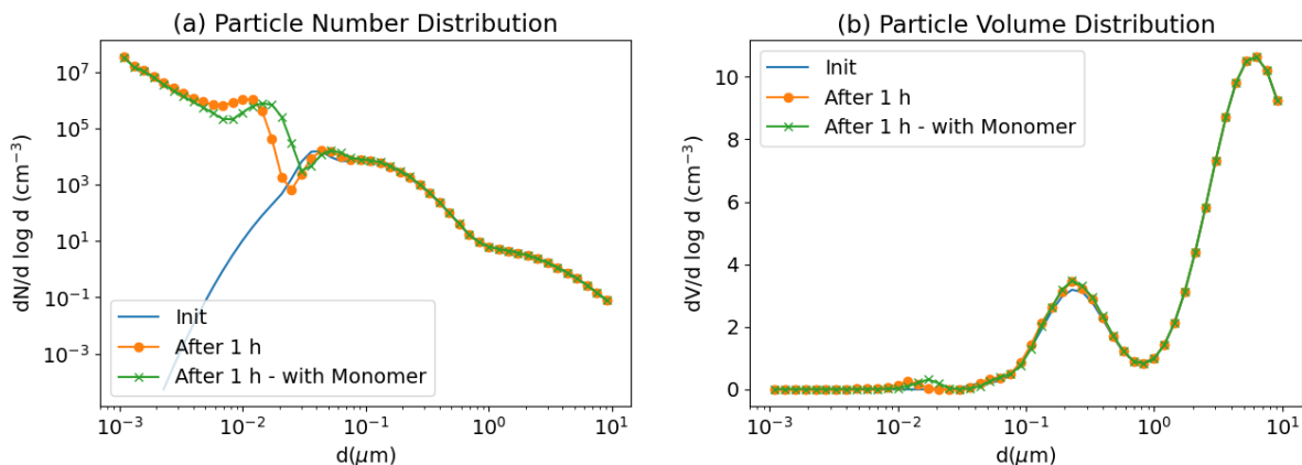
Figure 16. Size distribution of particles in the nucleation test case. Under hazy conditions, nanoparticles nucleated from water, sulfuric acid and ammonia grow to larger size. A simulation adding ELVOCs (Monomer) to the initial conditions is performed to illustrate their effect on the growth of ultrafine particles. Number (left panel, a) and volume (right panel, b) concentrations.
