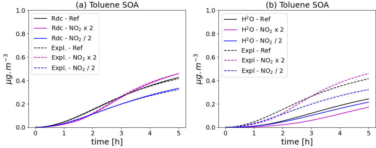
Figure 4. Time evolution of toluene SOA mass with different chemical schemes and for different \text{NO}_2 initial concentrations (Ref. denotes the reference \text{NO}_2 levels, \text{NO}_2 \times 2 the simulation with doubled \text{NO}_2 , and \text{NO}_2 / 2 the simulation with halved \text{NO}_2 ). In the right panel (a), the near-explicit chemical scheme of Lannuque et al. (2023) supplemented by molecular rearrangement with ring opening of a bicyclic peroxy radical with an O-O bridge Iyer et al. (2023); Sartelet et al. (2024) is compared to the \text{H}_2\text{O} mechanism. In the left panel (b), the near-explicit scheme (Expl.) is compared to the reduced scheme (Rdc.) of Sartelet et al. (2024).
