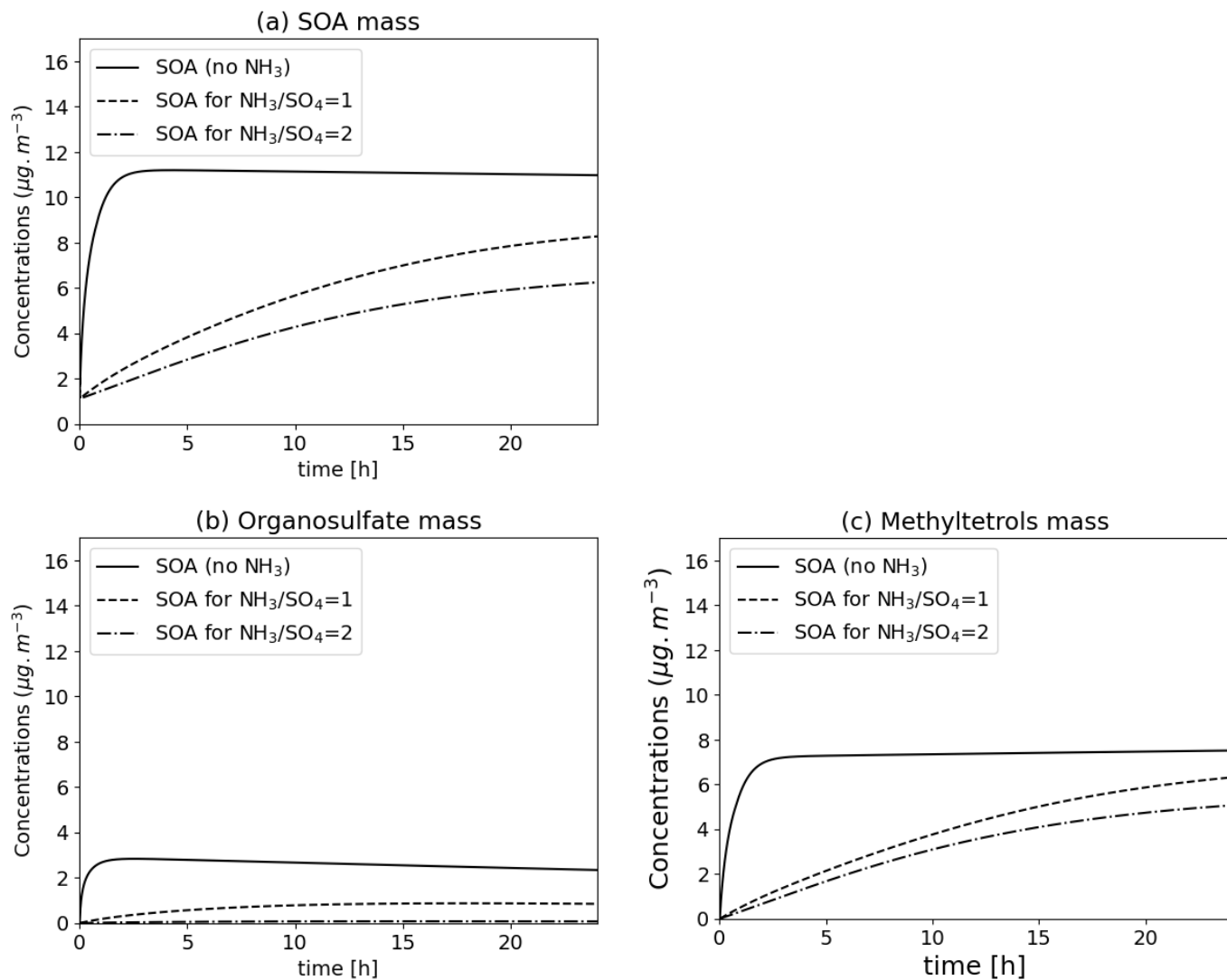
Figure 14. Formation of SOA (top, panel a), organosulfate (bottom left, panel b) and methyltetrols (bottom right, panel c) due to the reaction of 10 μg/m 3 IEPOX in the particle phase (in the presence of 10 μg/m 3 of HNO 3 at the beginning of the reaction and 3 μg/m 3 of sulfate) for a different ratio of ammonia to sulfate.
