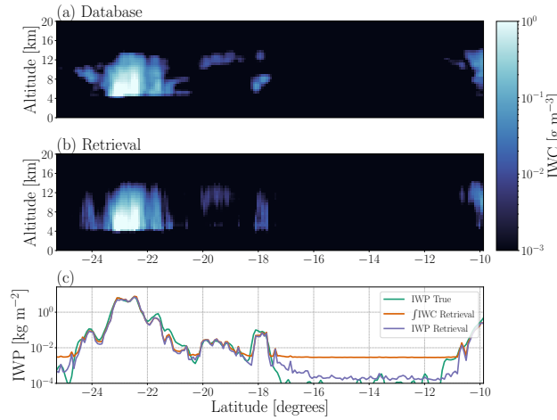
Figure 7. A comparison of IWC profiles, with database IWC shown in (a), and the corresponding retrieved IWC shown in (b). Panel (c) shows IWP across the scene. ‘IWP True’ is the IWP in the retrieval database, ‘IWP Retrieval’ is the retrieved IWP, and ‘ \int IWC’ is the integral of IWC, i.e. IWP, calculated for retrieved IWC cases in a given profile. The retrieved IWC is plotted using the retrieval mean as the single estimate for each case. The scene corresponds to a CloudSat overpass on 22 January 2009 at approximately 04:15.
