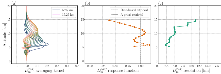
Figure 13. Averaging kernels for retrieved D_m^{IWC} are shown in panel (a). In panel (b), the corresponding measurement response function is given as a function of altitude. The estimated retrieval resolution, estimated from the FWHM of the averaging kernels, is shown in panel (c).
