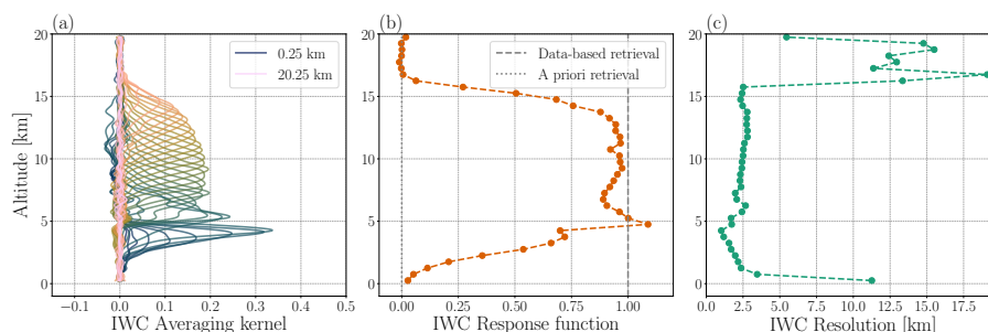
Figure 12. Averaging kernels for retrieved IWC are shown in panel (a). In panel (b), the corresponding measurement response function is given as a function of altitude. The estimated retrieval resolution, estimated from the FWHM of the averaging kernels, is shown in panel (c).
