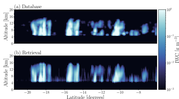
Figure 3. A comparison of IWC profiles, with database IWC shown in (a), and the corresponding retrieved IWC shown in (b). The retrieved IWC is plotted using the retrieval mean as the single estimate for each case. The scene corresponds to a CloudSat overpass on 28 January 2009 at approximately 17:30.
