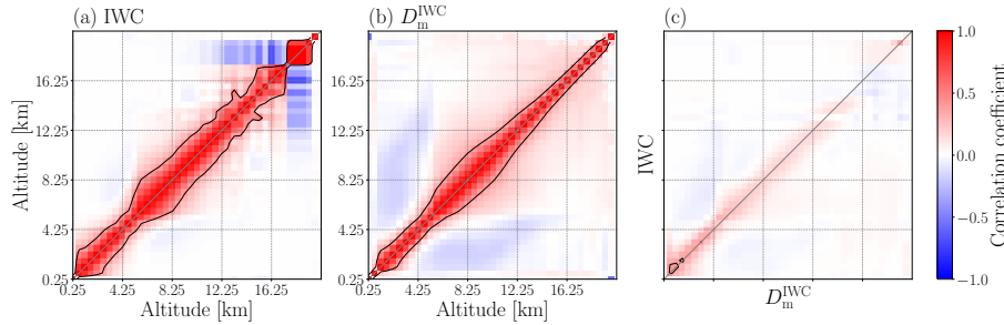
Figure 11. Error correlation matrix for retrievals of IWC, in panel (a), and retrievals of D_m^{\text{IWC}} , in panel (b). The error cross-correlation matrix between IWC and D_m^{\text{IWC}} is shown in panel (c). The errors are calculated as the difference between the retrieved value and the database value. The correlation matrices are computed over all IWC and D_m^{\text{IWC}} data that correspond to a database IWP > 0.1 \text{ kg m}^{-2} , i.e. the same threshold used for the averaging kernel calculations in Sect. 5.4. The black contour line indicates the approximate altitude below which the correlation coefficient falls below e^{-1} , or \sim 37\% . Each grid cell, or matrix element, is 500 m in width and height.
