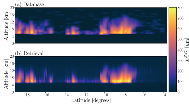
Figure 10. A comparison of D_m^{\text{IWC}} profiles, with database D_m^{\text{IWC}} shown in (a), and the corresponding retrieved D_m^{\text{IWC}} shown in (b). The retrieved D_m^{\text{IWC}} is plotted using the retrieval mean as the single estimate for each case. The scene corresponds to a CloudSat overpass on 1 February 2009, at approximately 13:00.
