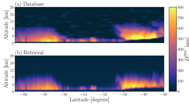
Figure 9. A comparison of D_m^{\text{IWC}} profiles, with database D_m^{\text{IWC}} shown in (a), and the corresponding retrieved D_m^{\text{IWC}} shown in (b). The retrieved D_m^{\text{IWC}} is plotted using the retrieval mean as the single estimate for each case. The scene corresponds to a CloudSat overpass on 22 January 2009 at approximately 19:15.
