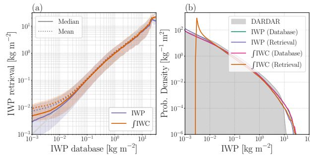
Figure 6. Comparison of IWP calculated from retrieved IWC to database IWP. In panel (a), the mean, median, 16th and 84th percentiles are shown. Panel (b) shows the overall distribution of IWP obtained in four different ways: Database IWP, retrieved IWP, the column integral of database IWC, and the column integral of retrieved IWC. The distribution of IWC from the DARDAR 3.1 product is also shown in panel (b).
