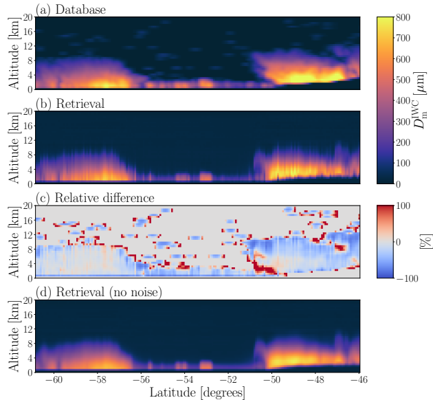
Figure 9. A comparison of D_m^{\text{IWC}} profiles, with database D_m^{\text{IWC}} shown in (a), and the corresponding retrieved D_m^{\text{IWC}} shown in (b). The retrieved D_m^{\text{IWC}} is plotted using the retrieval mean as the single estimate for each case. Panel (c) shows the difference between the retrieval and the database, relative to the database value. Only data points with either database or with retrieved IWC \geq 1 \text{ mg m}^{-3} are shown. Panel (d) shows the retrieval performed on noise-free input data. The scene corresponds to a CloudSat overpass on 22 January 2009 at approximately 19:15.
