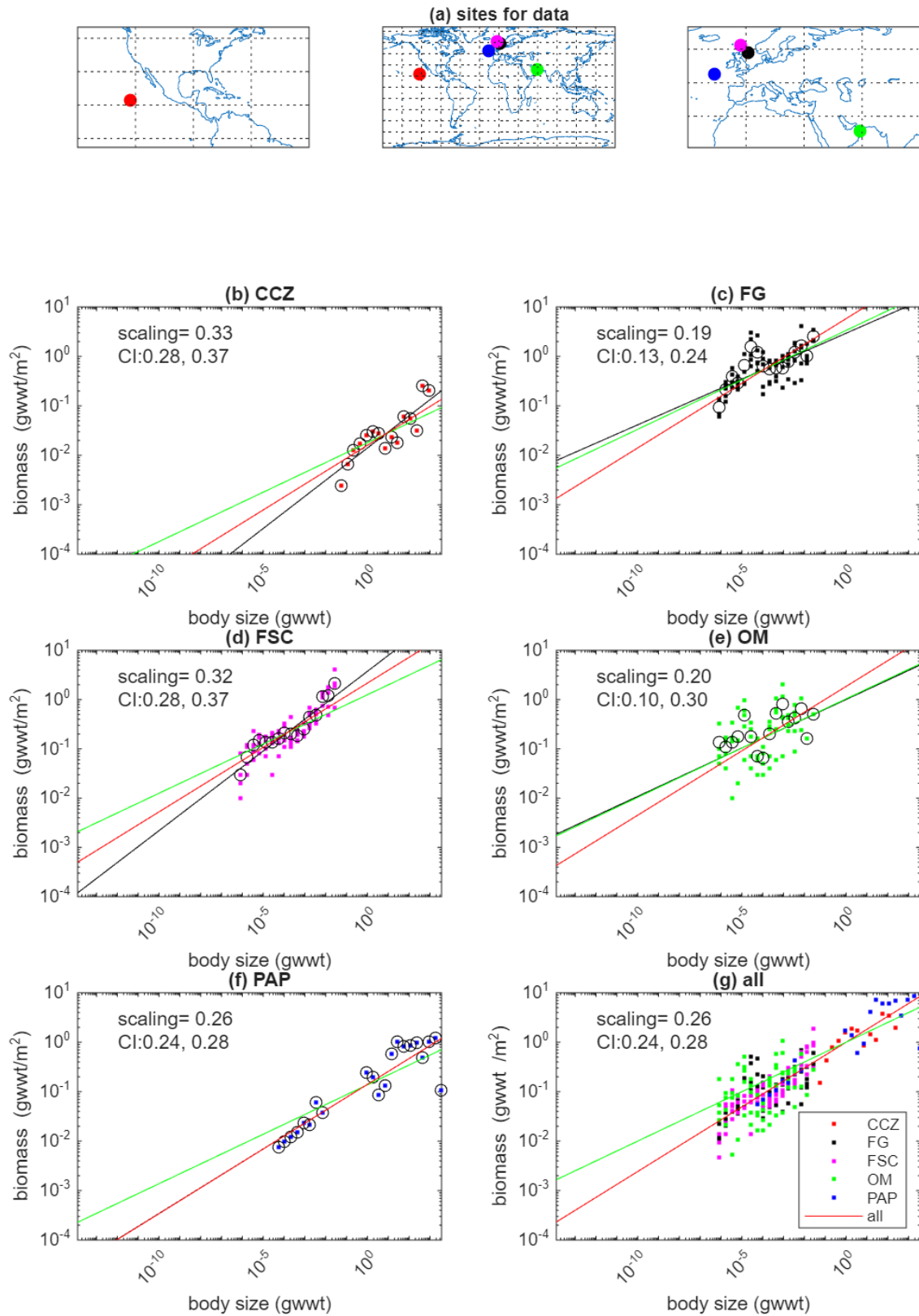
1003 Figure 3 Locations (top) and observations of biomass as a function of body size for the five sites listed in Table 2. For each of the 1004 sites the dots show observations, circles indicate means within size classes and the black line is a power-law fit to the observations. 1005 The fitted values for the scaling exponent together with 95% confidence intervals are also shown. The bottom right panel shows the 1006 fit to all sites simultaneously, assuming a common scaling exponent (fitted value shown with 95% CI) but allowing the pre-factor to 1007 vary across sites. The dots show data from the sites with colours matching those used in the panels for individual sites. Note that in 1008 the bottom right panel the data from each site has been normalised by dividing by the fitted pre-factor to allow the visual comparison. 1009 The red line in all panels is the simultaneous fit to all sites. The green line in all plots is the relationship used in the model by fitting 1010 a power-law with an imposed scaling of 0.2 to the same observations.
