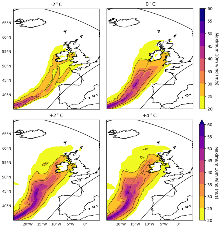
Figure 9. 10m wind footprint for Ophelia in the -2^{\circ}\text{C} , 0^{\circ}\text{C} , +2^{\circ}\text{C} , and +4^{\circ}\text{C} alternate climate scenarios, with their respective tracks. Contour lines at storm-force (10 Bft, 24.7 m/s) and hurricane-force (12 Bft, 32.8 m/s). RACMO domain bounds are also shown.
