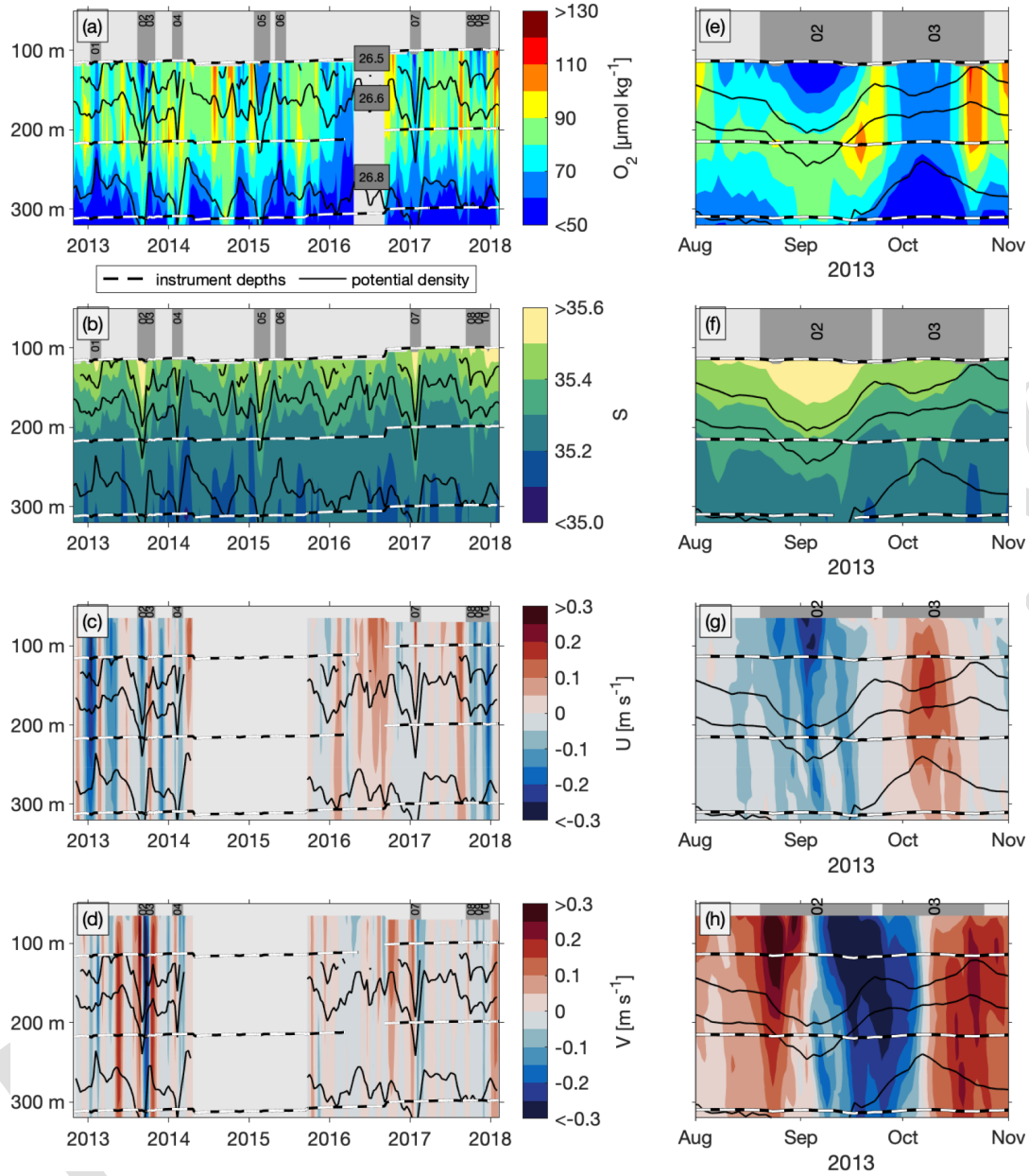
Figure 5. Time series of observed (a) DO, (b) salinity, (c) eastward and (d) northward velocity from moored observations at 11^{\circ}\text{N}/21^{\circ}\text{W} in the upper 300 m as a 10 d average (color shading). Black lines denote depth of potential density surfaces 26.5 , 26.6 and 26.8\text{ kg m}^{-3} . Black-white dashed lines denote depths of DO sensors – in (a), (c) and (d) – and salinity sensors (in b). Gray bars with numbers 01–10 in the top of these panels denote time periods of low-DO events (#01 to #10). Note, that no velocity observations are available for low-DO events #05 and #06. Panels (e)–(h) show corresponding 2 d averaged time series for the 90 d time period around low-DO events #02 and #03.
