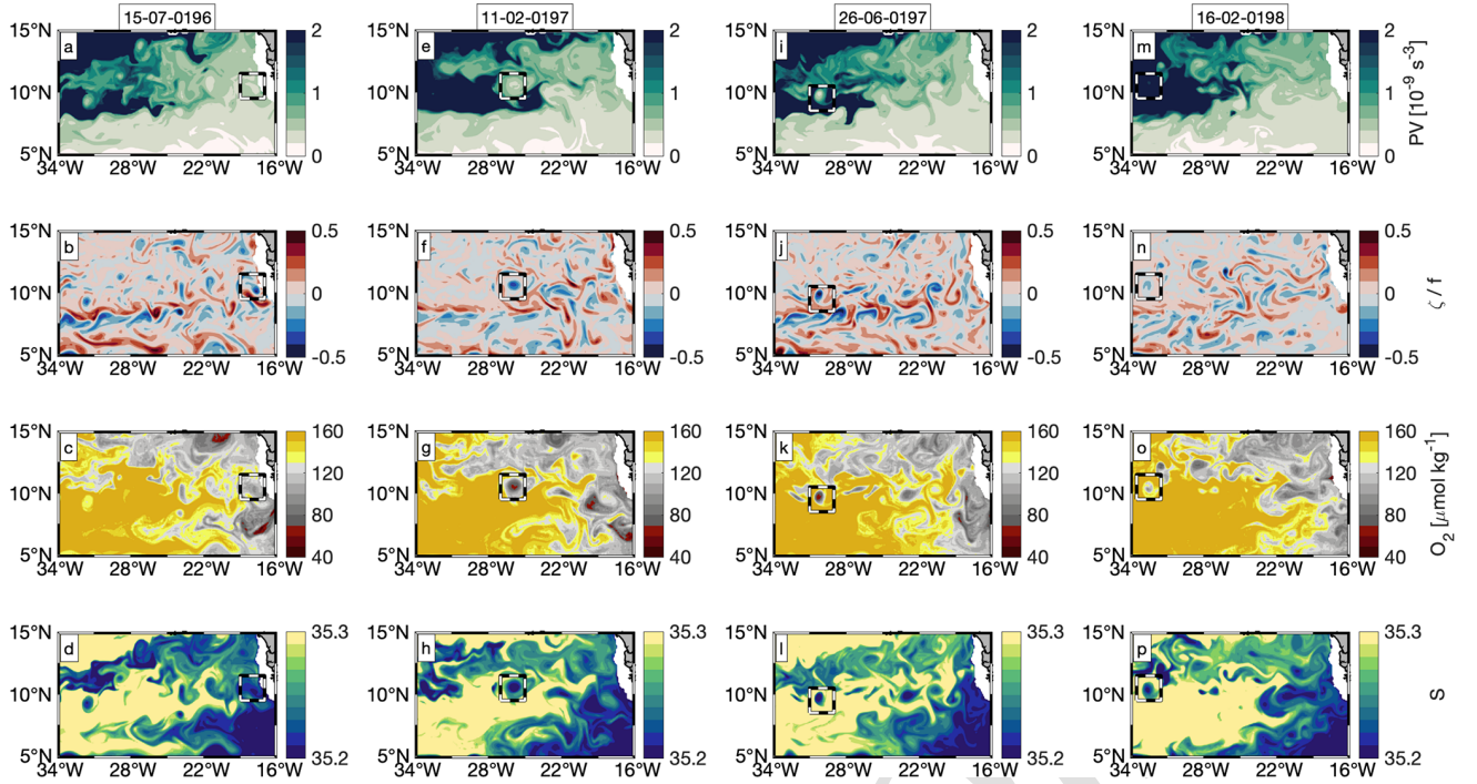
Figure 9. Model snapshots of PV on isopycnal surface 26.6 \text{ kg m}^{-3} (a, e, i, m), relative vorticity over f , DO and salinity on isopycnal surface 26.5 \text{ kg m}^{-3} (b, c, d, f, g, h, j, k, l, n, o, p) for different phases (different columns) of an anticyclonic HBV (respective time indicated above each column with T = 0/211/346/580 \text{ d} : formation/strongest peculiarity/weakening/decay). Black-white dashed box in each sub panel denotes HBV position.
