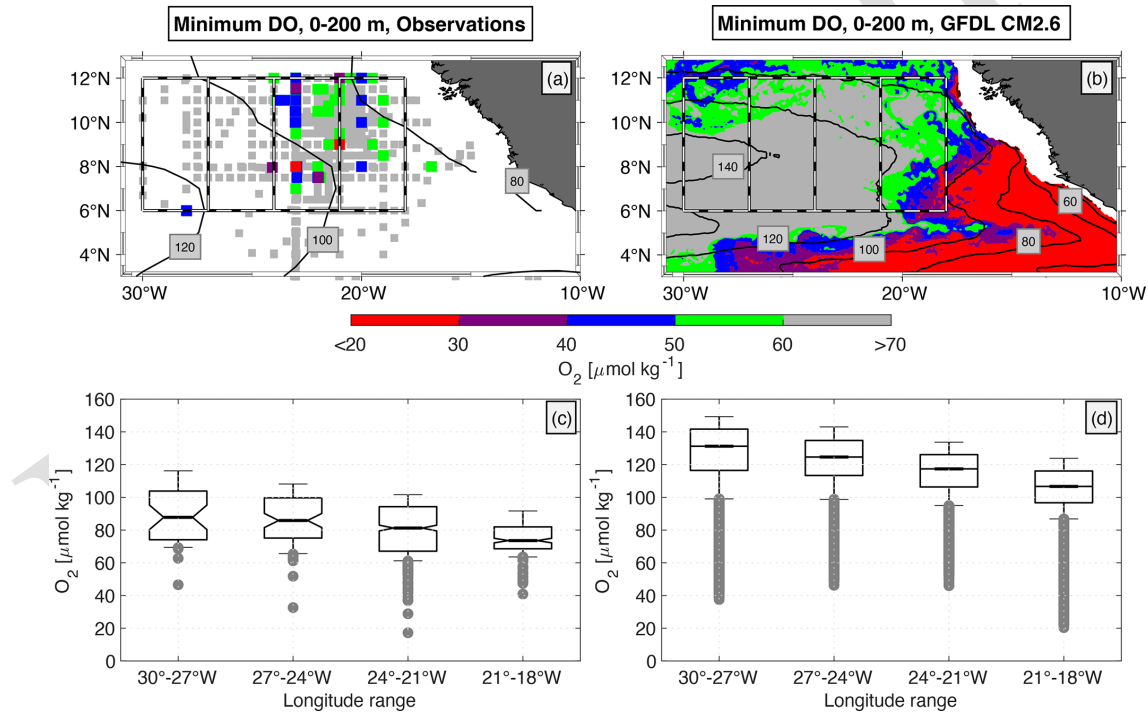
Figure 4. (a) Spatial distribution of DO profiles acquired from shipboard CTD-O observations in the tropical North Atlantic. Colored/gray dots denote DO profiles with a minimum DO concentration of lower/higher than 60 \mu\text{mol kg}^{-1} in the depth range 0–200 m (red: < 30 \mu\text{mol kg}^{-1} , violet: 30\text{--}40 \mu\text{mol kg}^{-1} , blue: < 40\text{--}50 \mu\text{mol kg}^{-1} , green: < 50\text{--}60 \mu\text{mol kg}^{-1} ). (b) Horizontal distribution of DO minimum obtained in the depth range 0–200 m and from the last 20 years of GFDL CM2.6 model run. Black contour lines in (a) and (b) show 0–200 m minimum of mean DO distribution (similar to filled contours in Fig. 2a and b). Dashed boxes denote different regions of interest for boxplots shown in (c) and (d). (c) Boxplots for 0–200 m minimum of DO profiles, that are shown for four different regions by the dashed boxes in (a). Thick line in each boxplot denotes median and notches show 95 % confidence interval. Upper and lower whiskers denote 10 % and 90 % quantiles. Grey dots below the lower whiskers show 10 % lowest DO events. (d) Similar to (c), but boxplots shown for 0–200 m minimum of DO profiles that were taken from the last 20 years of GFDL CM2.6 model run.
