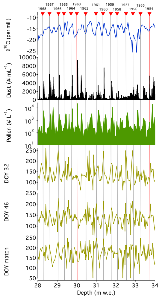
Figure 4: Annual layers between 28 and 34 m w.e. in core #1 shown in \delta^{18}\text{O} , dust and pollen concentrations, Day-Of-the-Year (DOY) 32 and 46 and DOY depth-to-day match variations (see text). Red vertical lines indicate time markers from the ^3\text{H} and beta activity peaks (Gabielli et al., 2016). See also Figs. S5 and S6 in the Supplementary Information which display annual layers in previous periods of the 20 th century.
