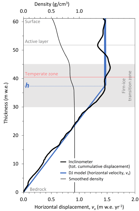
Figure 9: Vertical profiles of density and horizontal displacement (i.e., v_x ) for the Alto dell'Ortles drilling site. Also indicated is the elevation above bedrock defined as shear zone thickness h in the (DJ model (parameter h ), which was here derived determined empirically from based on the displacement measurements (see main text). The firn-ice transition zone, typically with density of 0.830 - 0.917 g cm -3 , (Cuffey and Paterson, 2006) is indicated by the grey shading while the grey and red lines mark the bottom of the active layer and temperate zone, respectively (see main text). The core #2 reference depth (sect. 2) is here expressed as thickness, with the surface of depth zero corresponding to the total of 61.15 m w.e. (74.88 m).
