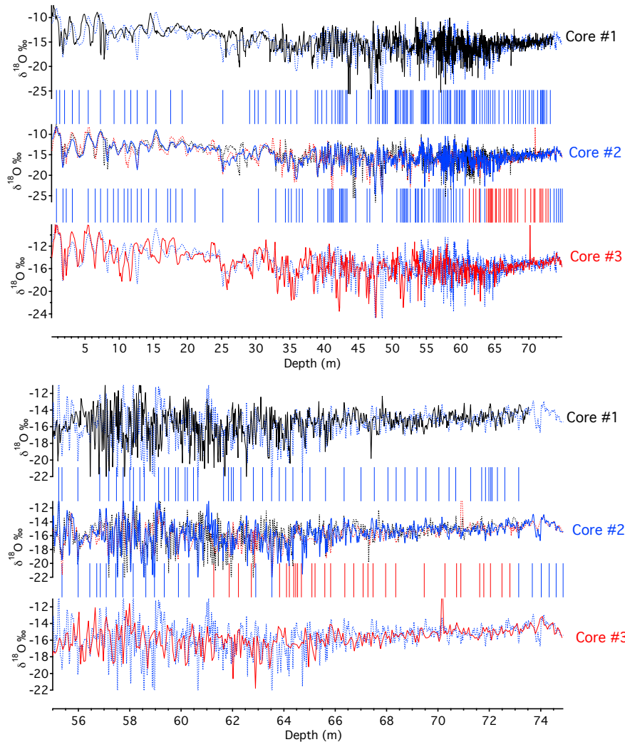
Figure 1: Revised depth alignments using the \delta^{18}\text{O} records from the Alto dell'Ortles cores #1 (in black, continuous and dotted lines ), #2 (in blue, continuous and dotted lines ) and #3 (in red, continuous and dotted lines ) over the entire lengths (upper panel) and the bottom portions (lower panel) of the cores. A common core #2 depth (X axis) is used in the mid panel for displaying of the three matched records, while the \delta^{18}\text{O} records in the top and bottom panels are shown on their original depth scales. Blue vertical lines indicate the \delta^{18}\text{O} tie points while red lines indicate tie points obtained through the Pb records of cores #1 and #3 (see Fig. 2). Adapted from Fig. 10 in Gabrielli et al., (2016).
