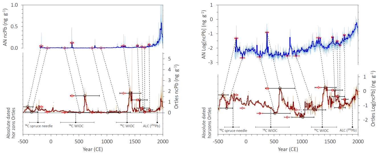
Figure 6: Synchronization of non-crustal lead (the Pb record of ncPb; dark red record) non-crustal concentrations from the Alto dell'Ortles core #3 (in dark red) (dark red record) on the CP2025/1 timescale with the corresponding record from Akademii Nauk (AN; in blue record ) on its well-dated ( \leq \pm 5 years) chronology used as reference (McConnell et al., 2019).
