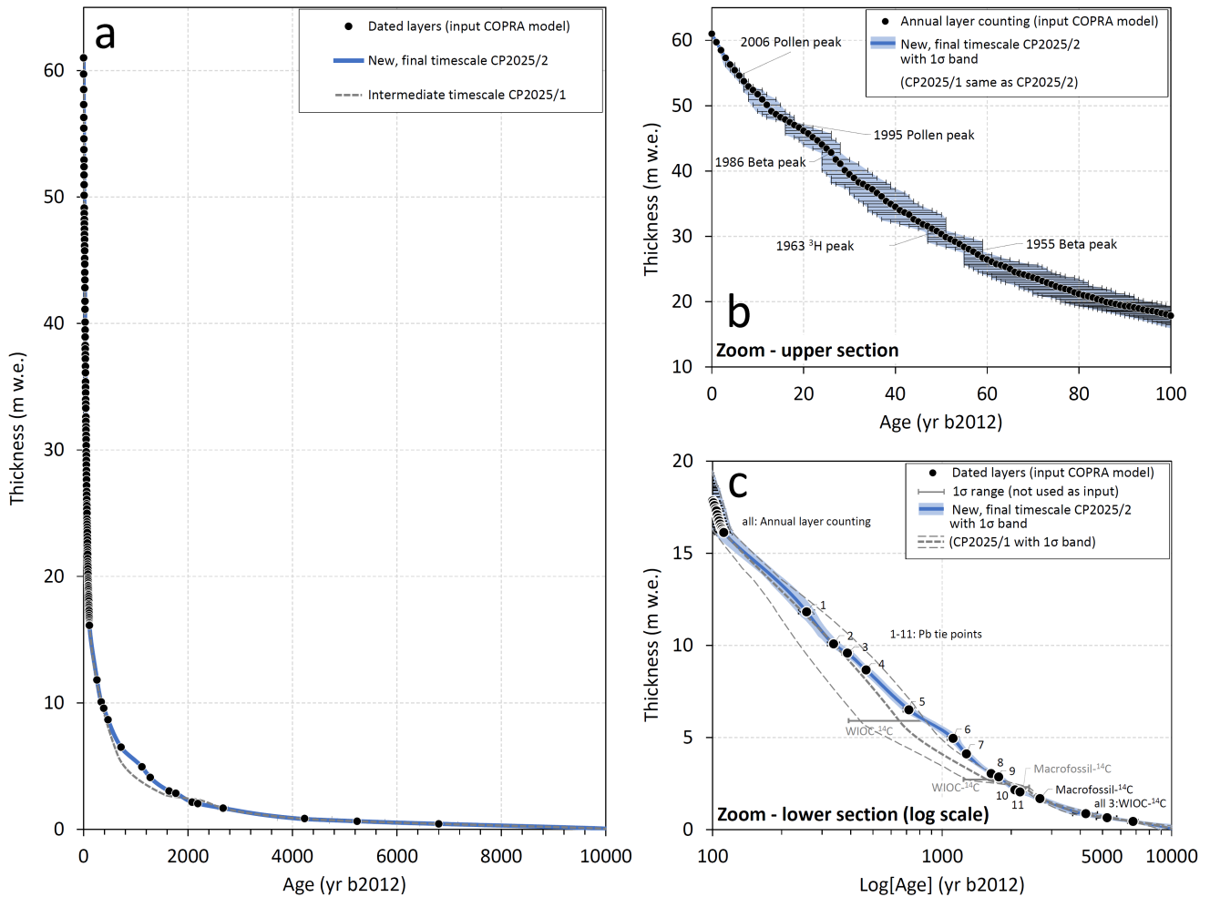
Figure 7: Comparison of the intermediate (CP2025/1, before synchronisation) and the final Alto dell'Ortles (CP2025/2) timescales. The different time markers used for construction (see listed in Supplementary Table S2) are indicated by symbols with error bars illustrating their uncertainty by the linked dating methods (1σ range for 14 C cal ages; see text for others). The two-three 14 C data points that were not used for model input are indicated just by their 1σ range (grey bars). Shown in panel (a) for the entire length of the ice core from surface, indicated by the uppermost point, to bedrock covering the entire time period of the Alto dell'Ortles ice archive, in (b) for the last 100 years, and in (c) for the older part of the record (>100 years) on a logarithmic age scale. The core #2 reference depth (sect. 2) is here expressed as thickness, with the surface of depth zero corresponding to the total of 61.15 m w.e. (74.88 m).
