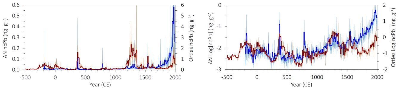
Figure 8: Comparison of the ncPb non-crustal Pb concentrations from Alto dell'Ortles #3 (Ortles; dark red) after synchronization with Akademii Nauk (AN) used for age reference ( McConnell et al., 2019 ) between 175 BCE and 1750 CE. Thin and thick lines show annual and 10-year averages, respectively. Same for both panels, except for Pb concentrations being plotted on a logarithmic scale on the right panel.
