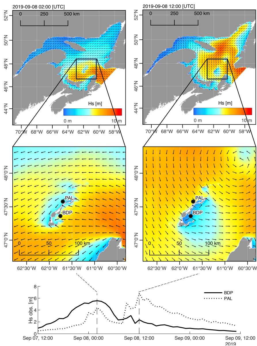
Figure 10. Top and middle panels show maps of the significant wave height H_s and wave direction predicted at the peak of the storm. The lower panel shows the evolution of H_s observed during the storm Dorian at Pointe aux Loups (PAL) and Baie de Plaisance (BDP).
