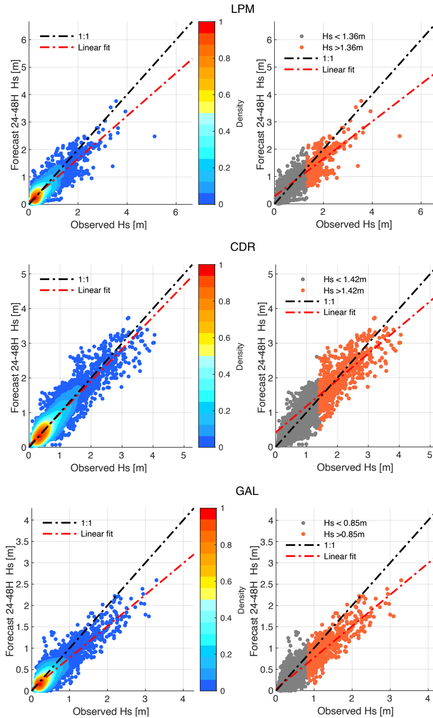
Figure 7. Scatter plot between observed and predicted significant wave height at the horizon 24-48h for AWAC stations CDR, GAL and LPM during the ice-free period (31 March to 15 January). The linear regression (orange dotted line) is applied to all waves on the left and to the highest 10% waves on the right.
