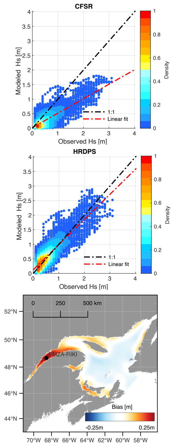
Figure 3. Comparison between observed and modelled significant wave height H_s at station PMZA-RIKI when forced by CFSR (top) and HRDPS winds (middle). The mean difference (HRDPS - CFSR) is shown in the bottom panel.
