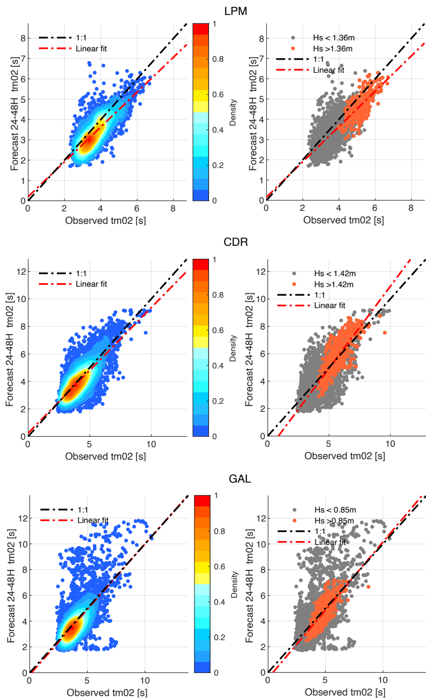
Figure B2. Scatter plot comparing observed and predicted mean wave period at the horizon 24-48h for AWAC stations CDR, GAL and LPM during the ice-free period (31 March to 15 January). The linear regression (orange dotted line) is applied to all waves on the left and to the highest 10% waves on the right.
