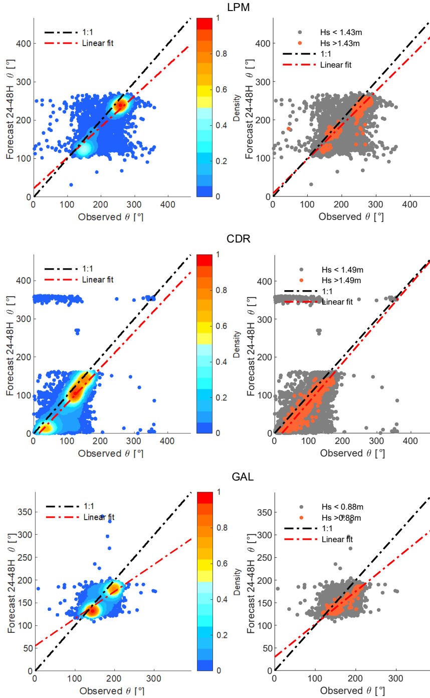
Figure B3. Scatter plot comparing observed and predicted mean wave direction at the horizon 24-48h for AWAC stations CDR, GAL and LPM during the ice-free period (31 March to 15 January). The linear regression (orange dotted line) is applied to all waves on the left and to the highest 10% waves on the right.
