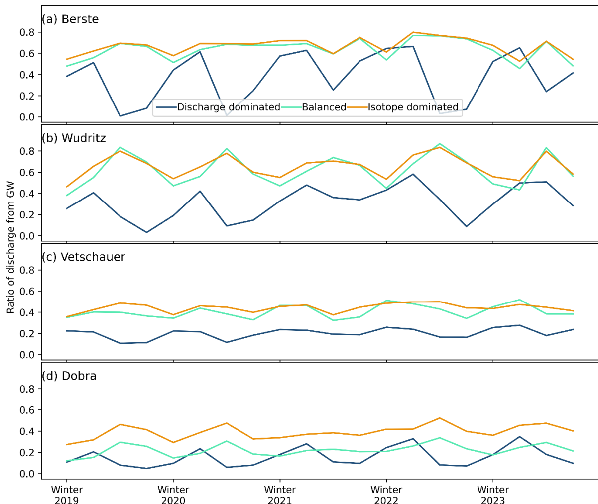
Figure 6. The mean ratio of seasonal runoff from groundwater storage at each catchment (winter, spring, summer, fall of each year along the X-axis). The results were calculated from the discharge dominated, balanced and isotope dominated solutions in schemes 2-5.
