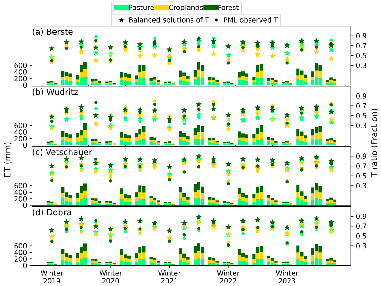
Figure 7. Seasonal total ET and transpiration ratio ( T/ET ) from the balanced solutions at (a) Berste in scheme 2; (b) Wudritz in scheme 3; (c) Vetschauer in scheme 4; (d) Dobra in scheme 5, and RS products. Bars and scatters indicate ET and T ratios, respectively. Each season contains three bars, ordered from left to right as follows: balanced solutions, MODIS and PML ET products.
