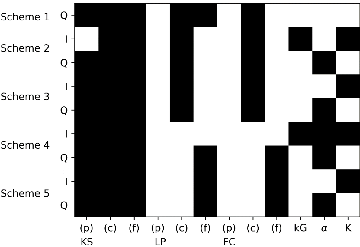
404 Figure 5. Sensitive parameters in each calibration scheme (The top six sensitive parameters 405 are shown shaded). I and Q in the y-axis represent isotopes and discharge; (p), (c), (f) represent 406 pasture, croplands, forest, respectively. kS, kG LP, \alpha , K control processes of runoff from soil, 407 runoff from groundwater, Actual ET, interception and ET partitioning, respectively; and FC is 408 the soil water storage capacity.
