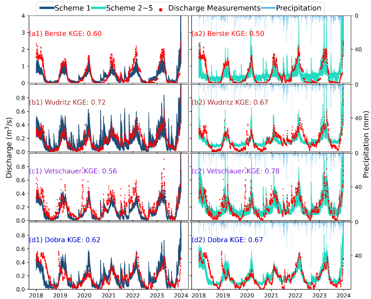
Figure 2. Discharge simulations at the outlet of each catchment based on the balanced solutions in the calibration scheme 1 (first panel (a1, b1, c1, d1)) and schemes 2-5 (second panel (a2, b2, c2, d2)). (a) Berste; (b) Wudritz; (c) Vetschauer; (d) Dobra.
