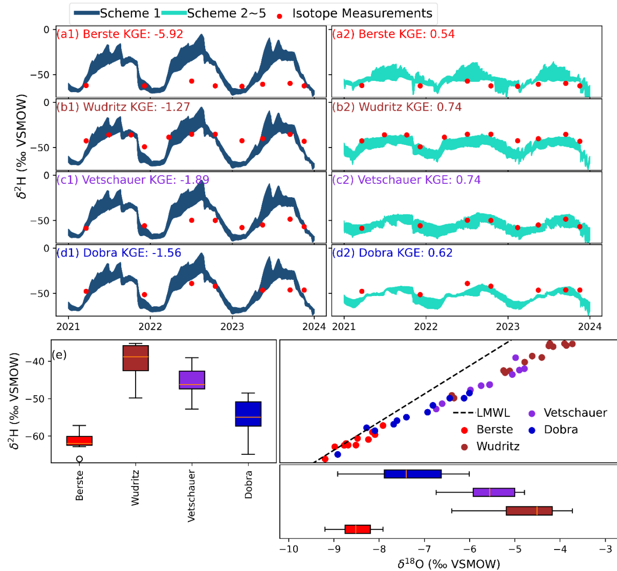
Figure 3. Stream water isotope simulations at the outlet of each catchment based on the balanced solutions in the calibration scheme 1 (first panel (a1, b1, c1, d1)) and schemes 2-5 (second panel (a2, b2, c2, d2)). (a) Berste; (b) Wudritz; (c) Vetschauer; (d) Dobra; and (e) Dual isotope from Jan 2021 to Dec 2023 in each catchment.
