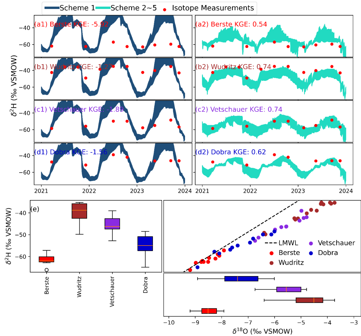
Figure 3. Stream water isotope simulations at the outlet of each catchment based on the balanced solutions in the calibration scheme 1(first panel (a1, b1, c1, d1)) and schemes 2-5(second panel (a2, b2, c2 d2)). (a) Berste; (b) Wudritz; (c) Vetschauer; (d) Dobra; and (e) Dual isotope from Jan 2021 to Dec 2023 in each catchment.
