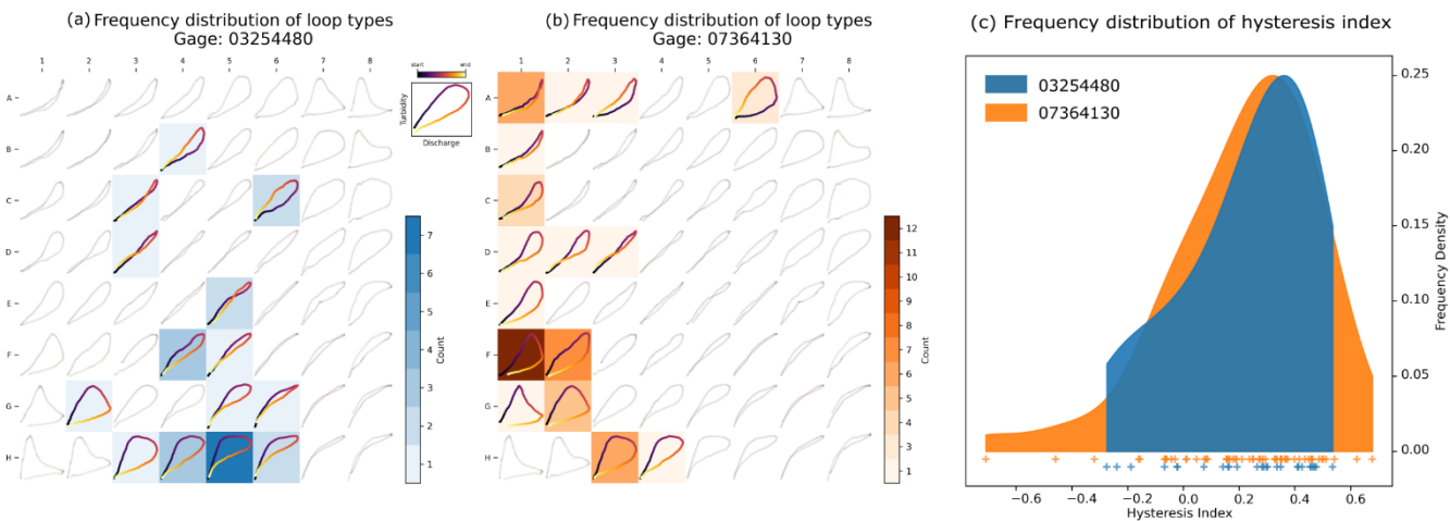
Figure 12. Frequency distribution of loop types for watersheds 03254480 (a) and 07364130 (b) mapped onto the General T-Q SOM and the hysteresis index (c). The frequency distributions mapped onto the General T-Q SOM reveal distinctions in loop types that are not captured by the hysteresis index.
