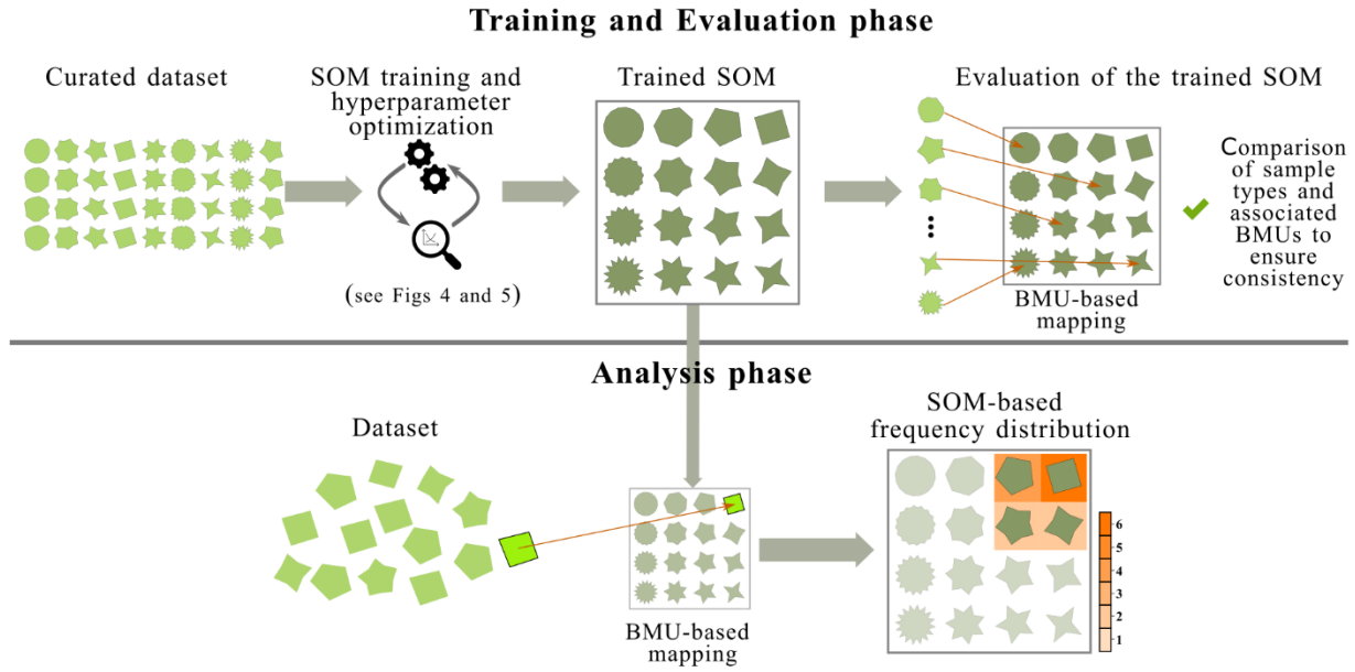
Figure 3. Workflow to generate an SOM for C-Q hysteresis loops ( Training and evaluation phase ) and apply the SOM for C-Q hysteresis analyses in watersheds ( Analysis phase ). Here, we illustrate the generation of the SOM using different shapes, which are analogous to the hysteresis loop types that might be found for a dissolved or particulate constituent in a watershed. In the bottom panel ( Analysis phase ), we demonstrate how hysteresis loops from a new dataset get mapped to the trained SOM, where the shade of orange represents the frequency with which the shape occurs in the dataset. The HySOM python package (see section 7) allows users to implement both phases of this workflow.
