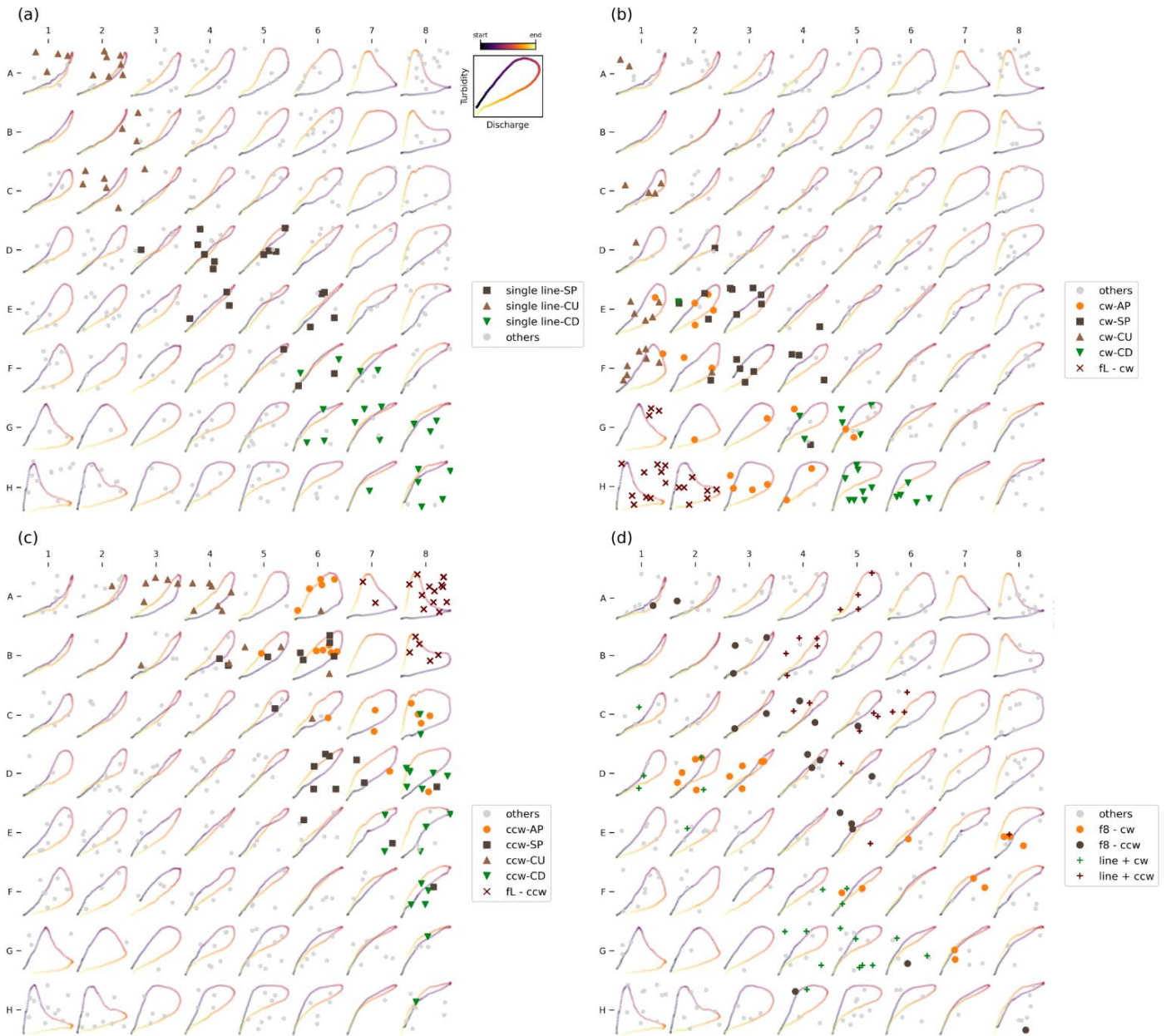
500 Figure 10. Mapping of all samples from the curated loop dataset to their respective BMUs on the trained SOM. For visual clarity, loop types and their mappings are organized into four distinct panels: (a) single-line loops; (b) clockwise loops including Async , Sync , Concave , and Figure-L ; (c) counterclockwise loops including Async , Sync , Concave , and Figure-L ; and (d) Figure-eight and Line+loops . Acronyms used in the figure include: SP – Sync-Peak , AP – Async-Peak , CU – Concave-Up , CD – Concave-Down , ccw – Counterclockwise , cw – Clockwise , fl – Figure-L , f8 – Figure-eight .
