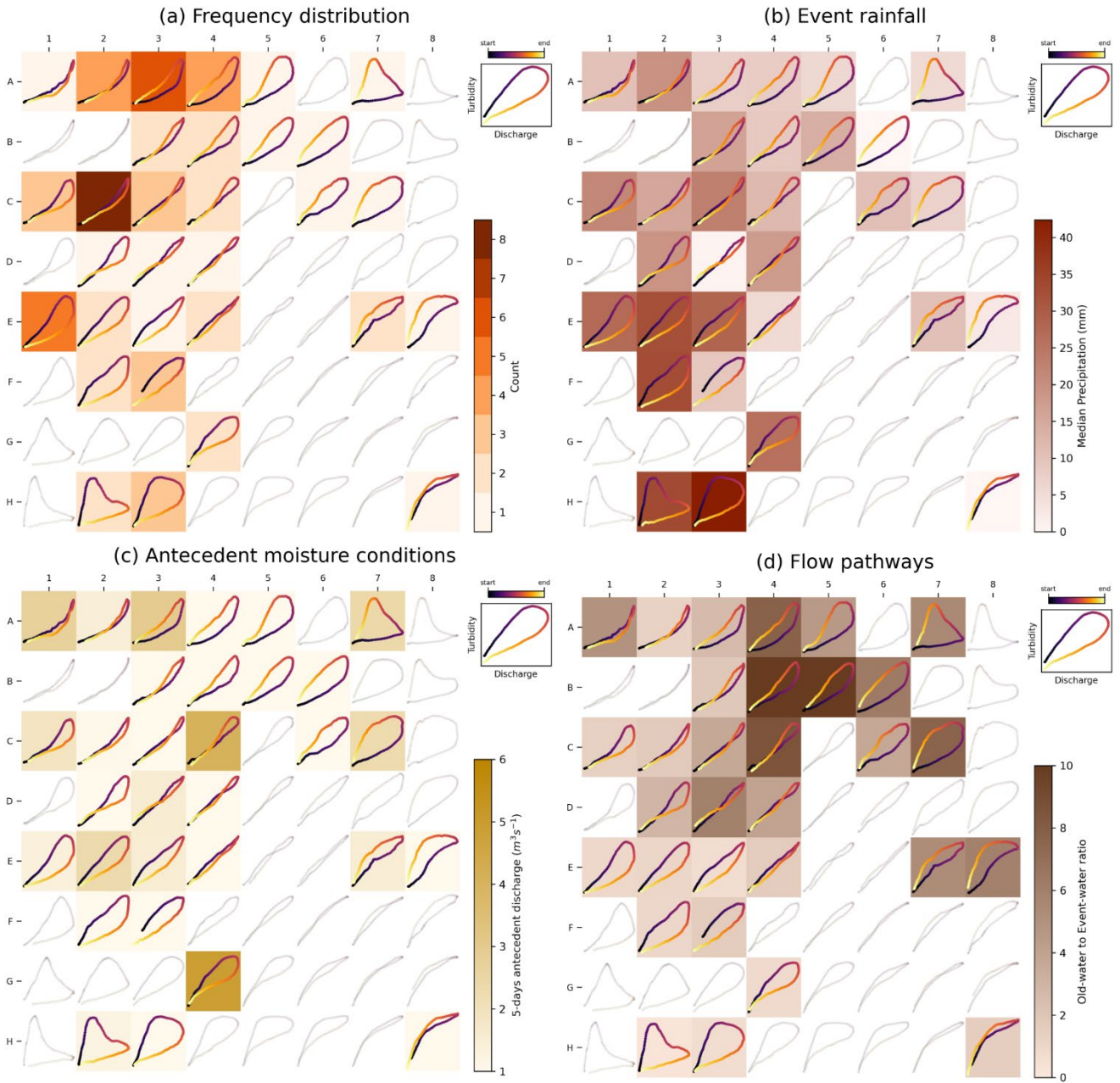
Figure 14. Heatmaps for watershed 03289000 of a) loop types, b) precipitation, c) antecedent discharge, and d) old-water to event-water ratio. The figure illustrates a visual approach for analyzing associations between hydrologic variables and loop types using the General T-Q SOM . In panels b and c, the color intensity represents the median values of the variable calculated for loop samples mapped to each prototype. Consistent patterns are evident for precipitation (higher precipitation for clockwise loops) and the old-water to event-water ratio (higher ratios for counterclockwise loops), whereas no discernible pattern can be seen for the 5-day antecedent discharge.
