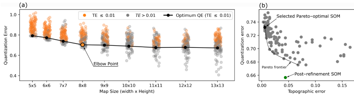
Figure 8. a) Quantization Error (QE) across varying map sizes, illustrating the expected decrease in QE as map size increases. While larger maps continue to lower the minimum QE, this reduction stabilizes when considering maps with low Topographic Error ( TE \leq 0.01 ). Similar stabilization patterns are observed across other TE thresholds (0.05 and 0.1). b) Scatterplot displaying QE and TE for 8 \times 8 maps. The map selected after visual inspection is highlighted, alongside the final QE and TE following map refinement training, which corresponds to the General T-Q SOM .
