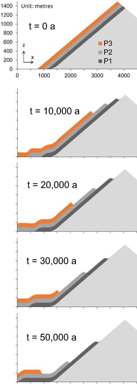
Fig. 6: Flow height evolution for the experiment SD1 along a longitudinal profile in down-slope (x) direction, assuming an extremely slow movement.
