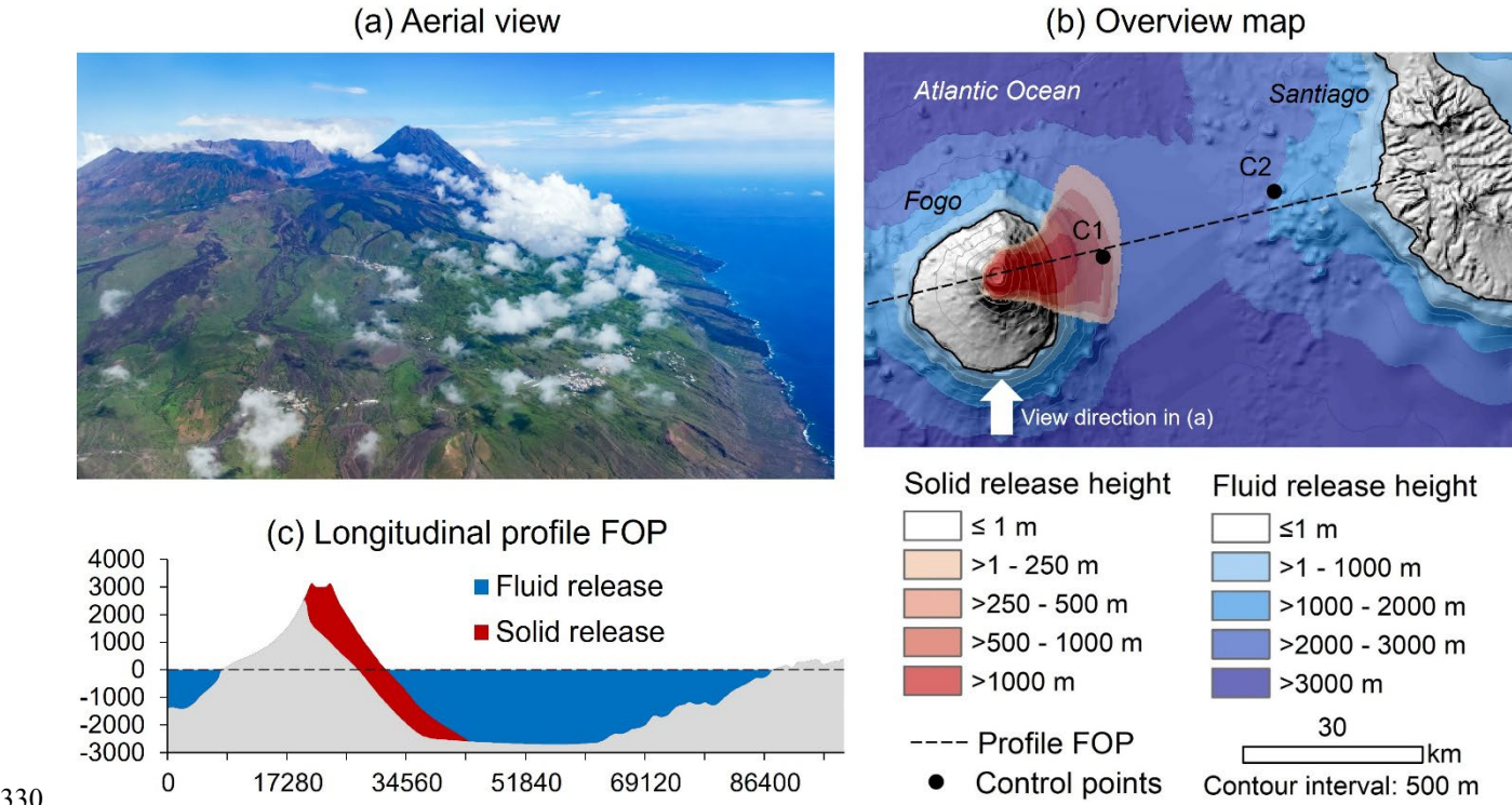
Fig. 4: Prehistoric East Fogo event. (a) Aerial view of today's situation with Pico do Fogo – author: M. Mergili, 10 September 2022; (b) Overview map with reconstructed release height distribution; (c) profile along the dashed line in (b).
