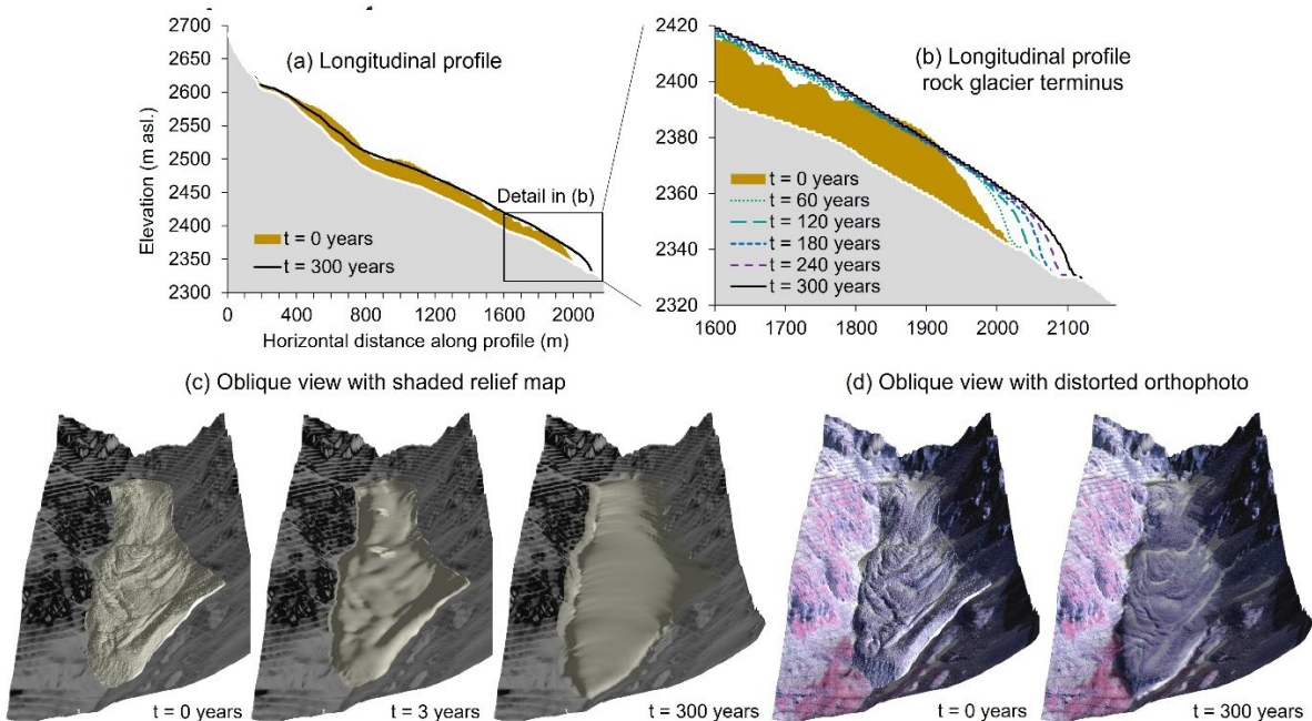
460 Fig. 12: Simulation results for the semi-generic Dösen rock glacier case. (a) Longitudinal profile along the main flow line for t = 0 and t = 300 years. (b) Longitudinal profile, detail of the rock glacier terminus for six selected time steps. (c) Oblique view against the flow direction, shaded relief map for t = 0 , t = 3 years, and t = 300 years. (d) Oblique view with distorted orthophoto for t = 0 and t = 300 years.
