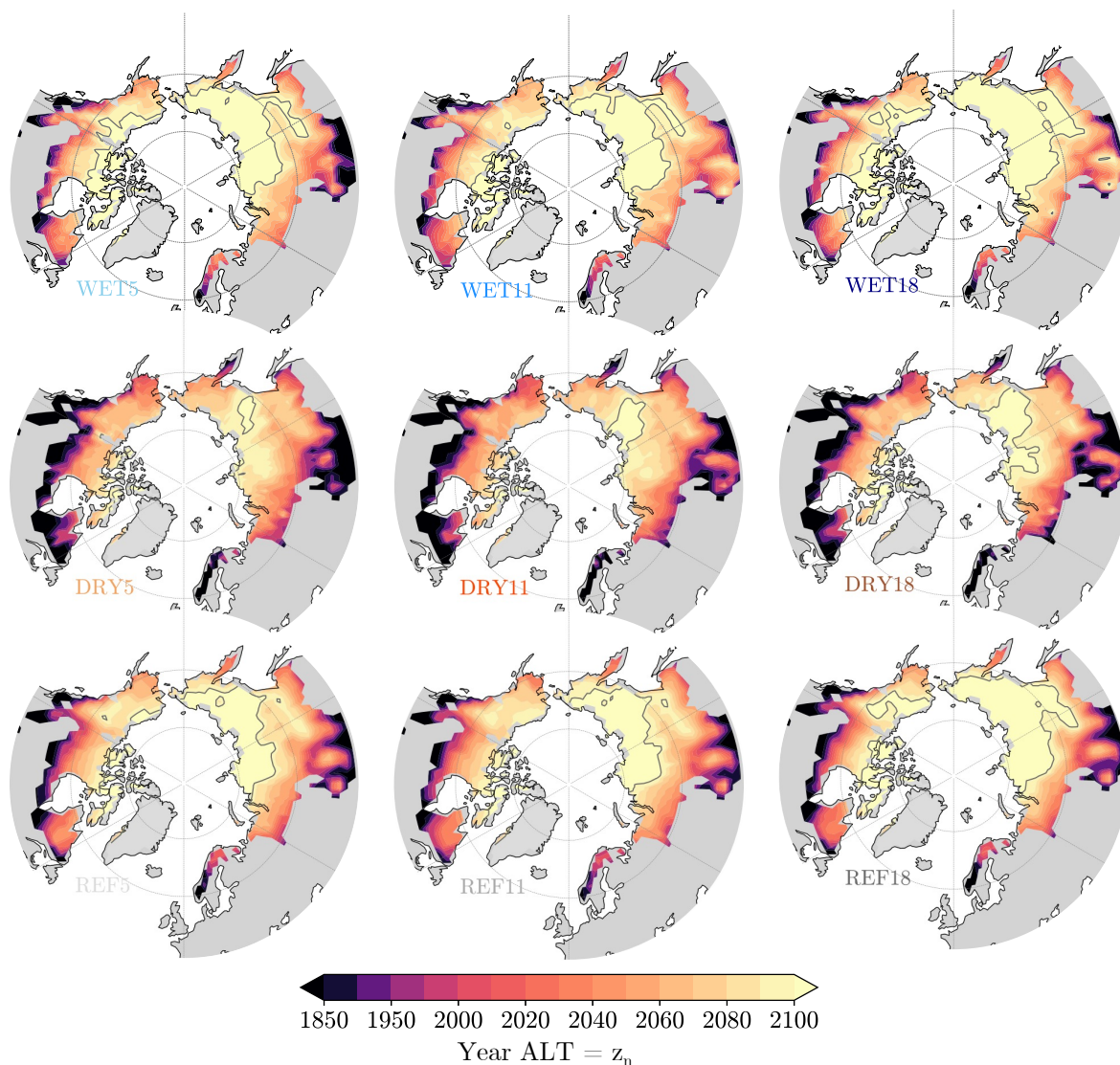
Figure 9. Deep permafrost presence with time for the combination of the three hydrological configurations (WET, DRY, REF) and vertical discretizations (5L, 11L, 18L). Spatial distribution of the last simulation year (HIS + SSP5-8.5) at which ALT is equal to the mid-layer depth of the bottom layer ( ALT = z_n ) for every simulation of the MPIESM-PePE. For the 18L simulations, 11L JSBACH z_n was taken in order to allow for comparison. Contour lines delimit areas where ALT do not reach z_n within the temporal extent of the simulation. The colored distribution stands over the permafrost domain displayed in Fig. 2a.
