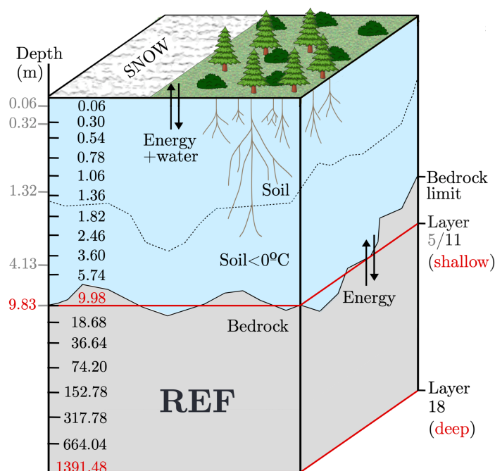
Figure 1. Main hydrological and thermodynamic features of the JSBACH standard version (REF). The mid-layer depth values for the default 5-layer (5L) vertical discretization, with a LSM depth at 9.83 m, are given on the left part of the y-axis. The corresponding values for the two enhanced discretizations of 11 (11L) and 18 (18L) layers introduced by this work are also shown, with LSM depths at 9.98 and 1391.48 m, respectively.
