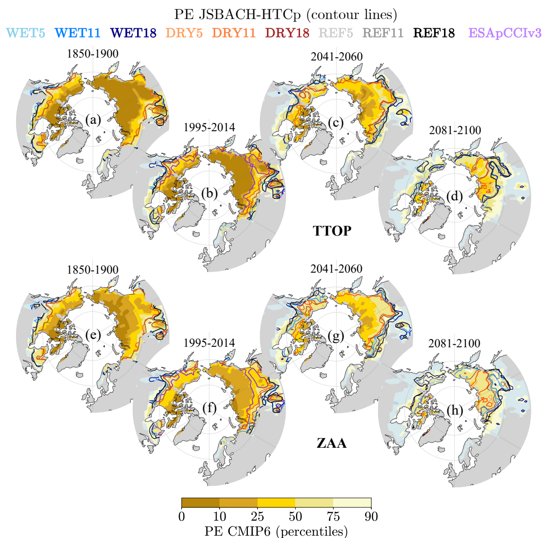
Figure 11. Permafrost extent (PE) for different periods in the MPIESM-PePE and CMIP6 ensembles in the historical and SSP5-8.5 scenario, and observed historical extension. PE CMIP6 10th, 25th, 50th, 75th, and 90th percentiles spatial distribution (shading) for TTOP (a–d) and ZAA (e–h) for 1850–1900, 1995–2014, 2041–2060, and 2081–2100. The extent and distribution of PE for the different MPIESM-PePE experiments in the same periods are depicted with contour lines of different colors (see legend), whilst the observational ESAPCCIv3 historical permafrost distribution in 1997–2019 is shown with a thicker purple contour line.
