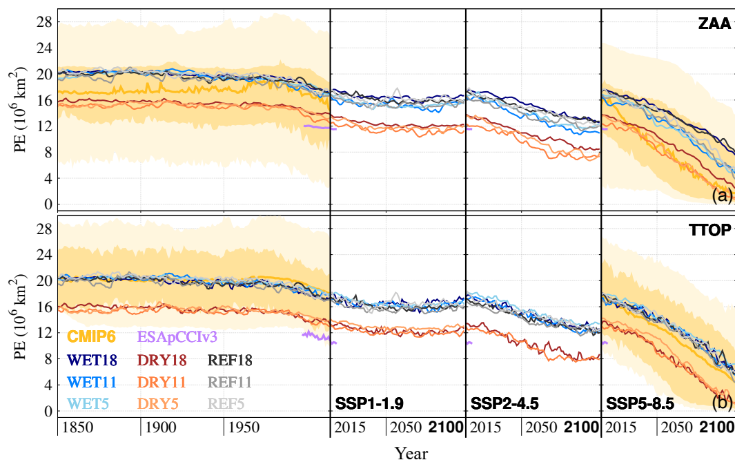
Figure 10. Permafrost extent evolution according to ZAA and TTOP (see Section 2.3.3). (a) PE ( 10^6 \text{ km}^2 ) using the ZAA definition for the different MPIESM-PePE simulations (solid lines, see legend for colors), the CMIP6 ensemble (gold solid line for the median, and dark (light) golden shading for the interquartile (interdecile) range), and the observational product ESApCCIV3 (purple solid line). (b) Same as (a), but for TTOP PE metric. CMIP6 PE data is only available for the historical period and SSP5-8.5 scenario (Steinert et al., 2023).
