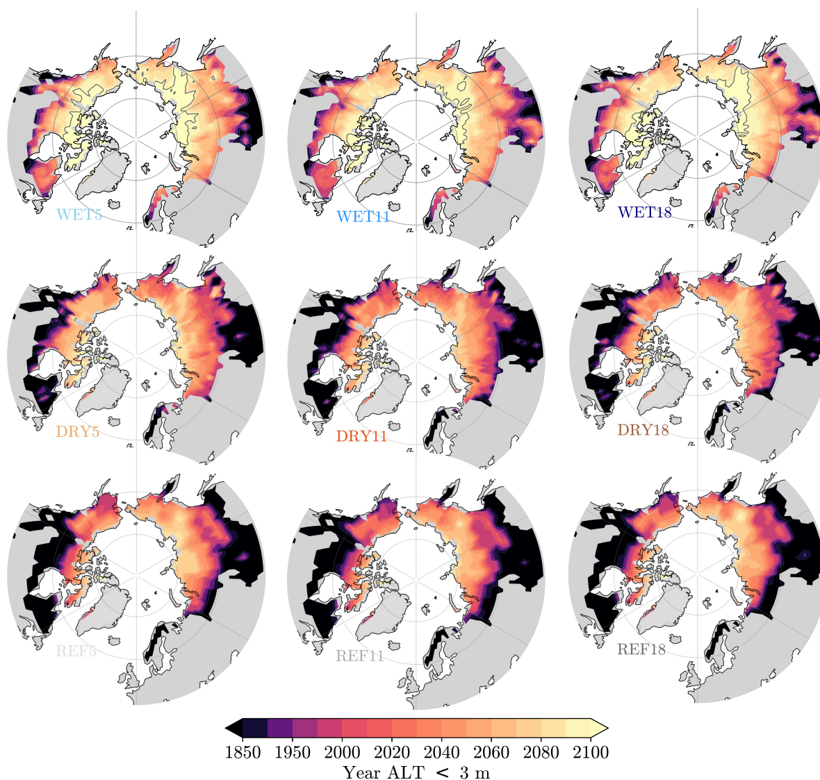
Figure 8. Near-surface permafrost presence with time for the combination of the three hydrological configurations (WET, DRY, REF) and vertical discretizations (5L, 11L, 18L). Spatial distribution of the last simulation year at which ALT is smaller than 3 m for every simulation of the MPIESM-PePE. The time evolution for historical and SSP5-8.5 experiments is shown in every case. Contour lines delimit areas where ALT does not reach 3 m within the temporal extent of the simulation. The colored distribution stands over the permafrost domain displayed in Fig. 2a.
