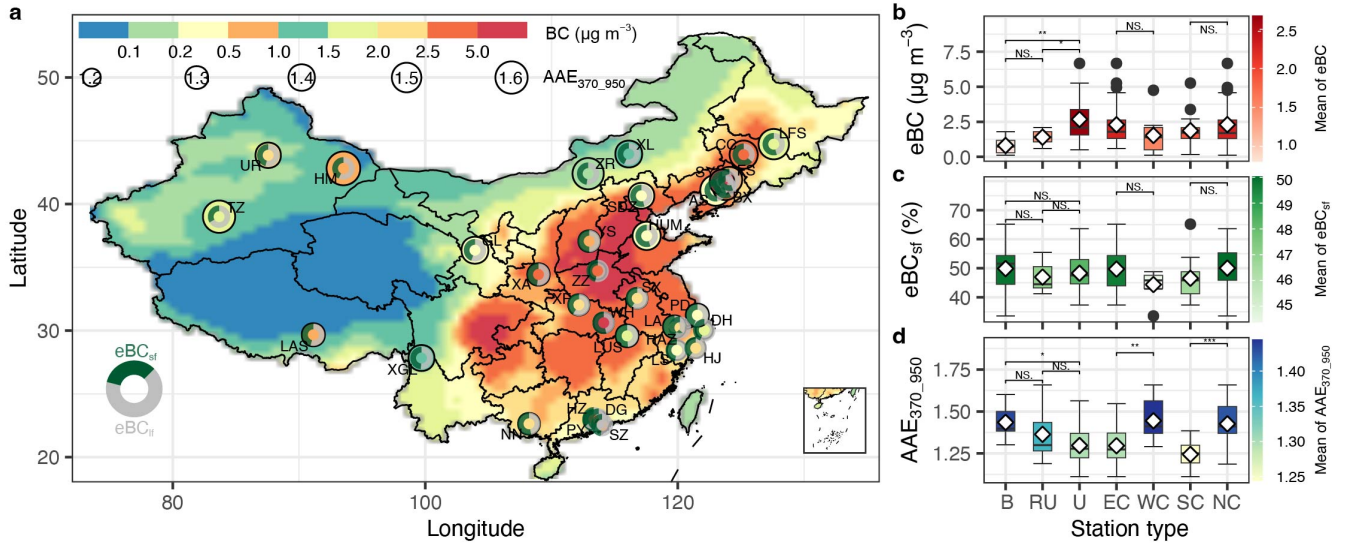
Figure 2. Spatial distributions of mean values of BC concentrations, source apportionment results sources of eBC including solid fuel (eBC sf ) and liquid fuel (eBC lf ) combustion , and absorption Ångström exponent between 2015 and 2017 (a), and their box plots (b–d) showing station-specific values for different types of stations, including baseline (B), rural (RU), and urban (U), as well as different regions in China: eastern China (EC), western China (WC), southern China (SC), and northern China (NC). The sizes and colors of the dots in panel (a) correspond to the mean values of AAE and eBC, respectively. The donuts in panel (a) represent the source apportionment results of eBC in each station. The data in the filled grid in panel (a) is from MERRA-2. NS, *, **, and *** in panels (b)–(d) indicate differences between two paired groups that are not significant ( p > 0.05 ) or significant at the 0.05, 0.01, and 0.001 levels, respectively.
