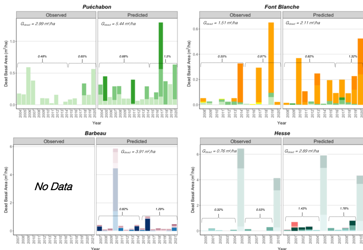
Figure W4 | Predicted versus observed evolution annual stand basal area loss due to mortality. For each simulation site, the bars depict the summed annual total basal area ( \text{m}^2/\text{ha} ) of all dead trees, broken down by species and size class). Observed values are derived from stand inventories, while predicted values are generated by the PHOREAU model. Also shown are the yearly basal area loss rates, calculated relative to the initial basal area for two distinct time periods in each simulation, along with the total basal area dieback per hectare ( G_{dead} ). Transparent bars indicate years with thinnings (see Appendices Q and R for details), which are excluded from the mortality statistics. Refer to Fig. 8 for species and cohort color codes.
