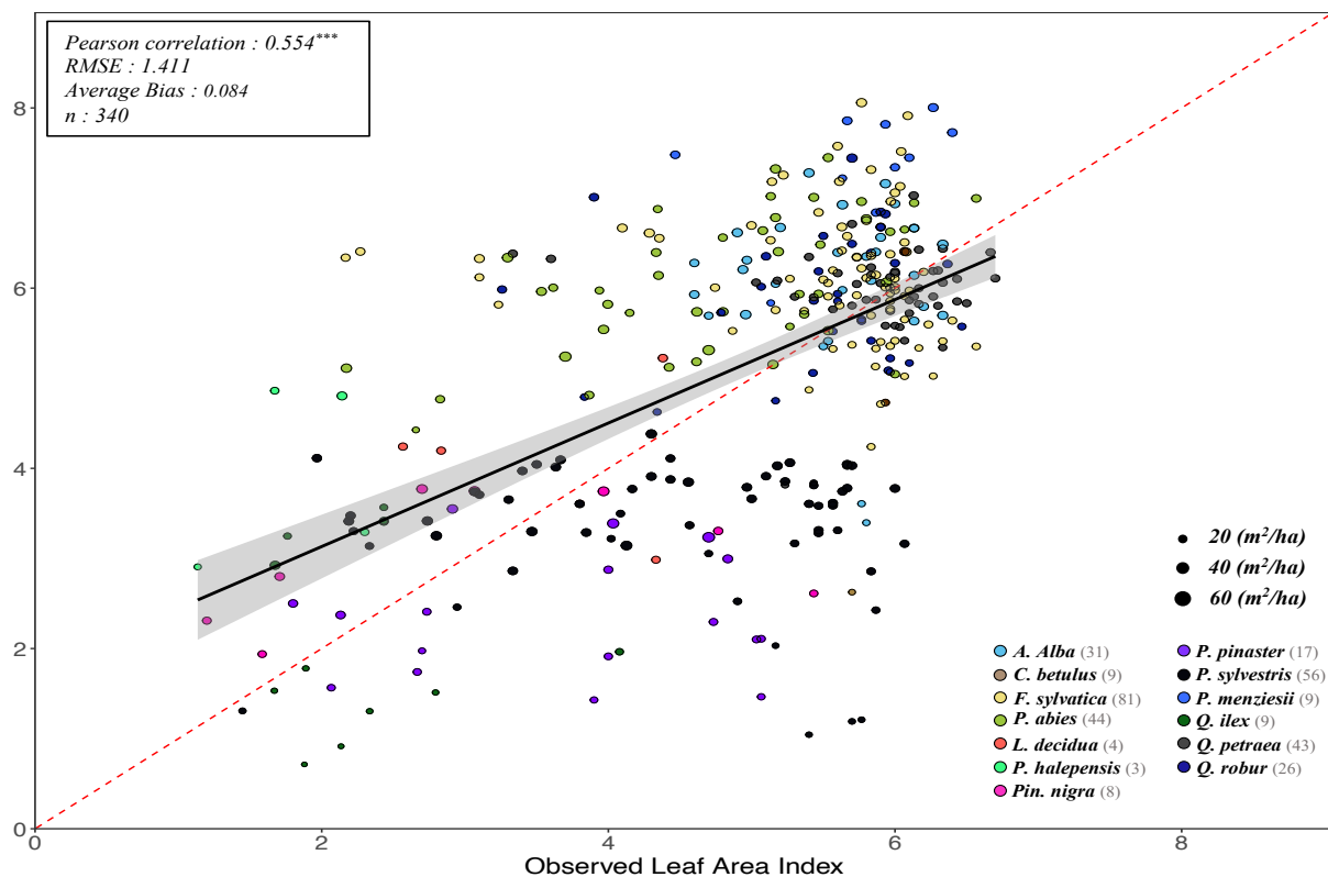
Figure 13 | Projected (by PHOREAU) against observed satellite leaf area index (LAI) for all 340 RENEFOFOR and ICP II validation inventories. The y-axis shows the LAI predicted by the model from the stand inventory at the start of the simulation, while the x-axis represents the PROBA-V LAI value for the matching coordinate and inventory year, averaged between July, August and September. Stand points are color coded by dominant species (see legend in bottom left). The size of points shows inventory basal area. The dashed red-line is the 1:1 line; the black full line represent the regression line of the linear model between observed and predicted LAI, with confidence interval represented by the grey shaded area. Associated statistics in Table S6.
