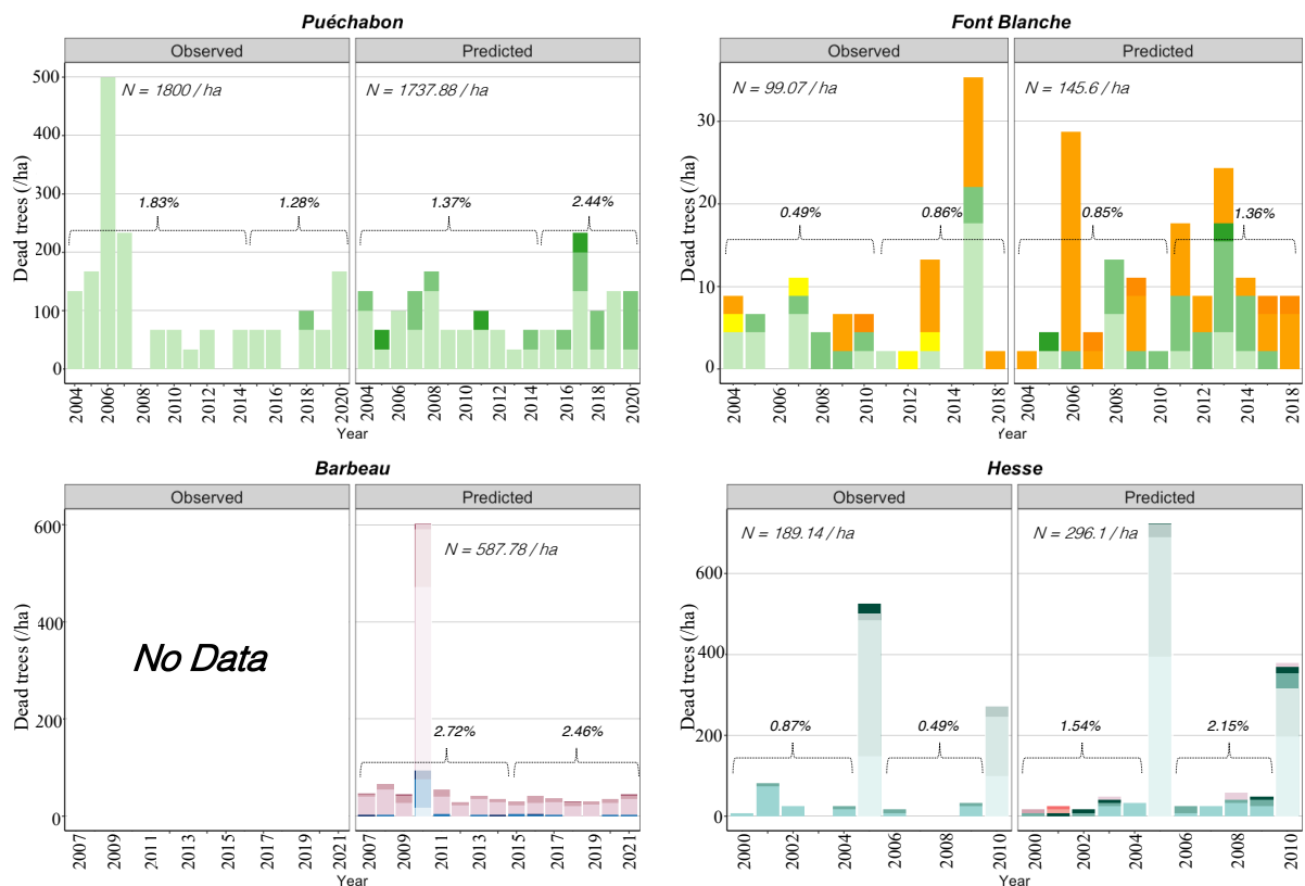
Figure 9 | Predicted versus observed annual tree mortality. For each simulation site, the bars depict the total annual number of dead trees, irrespective of cause, broken down by species and size class contributions. Observed values are derived from stand inventories, while predicted values are generated by the PHOREAU model. Also shown are the annual mortality rates, calculated relative to the initial number of trees for two distinct time periods in each simulation, along with the total number N of dead trees by hectare. Transparent bars indicate years with thinnings (see Table S17 for details), which are excluded from the mortality statistics.
