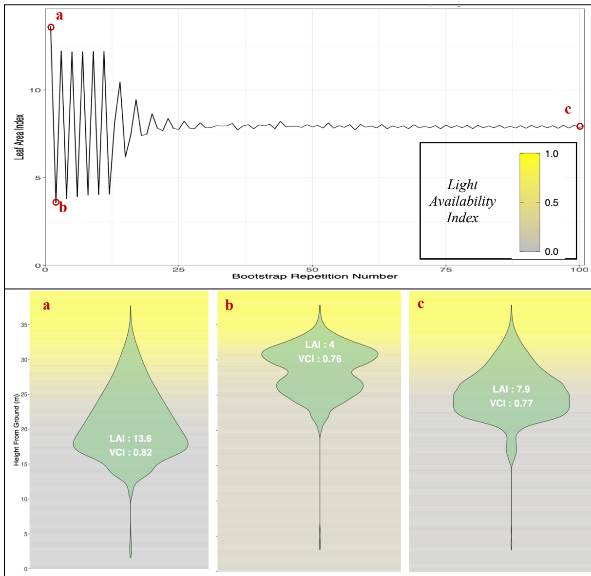
Figure M1 | Illustration of PHOREAU canopy bootstrap algorithm. Top: one-sided leaf area indices predicted by the PHOREAU bootstrap algorithm, initialized with a Picea abies dominated inventory (RENECOFOR EPC 39a, 2003). Bottom: three snapshots of predicted foliage area and light availability vertical stratification at different steps in the algorithm. For details on the calculation of the Vertical Complexity Index (VCI), refer to Appendix F.
