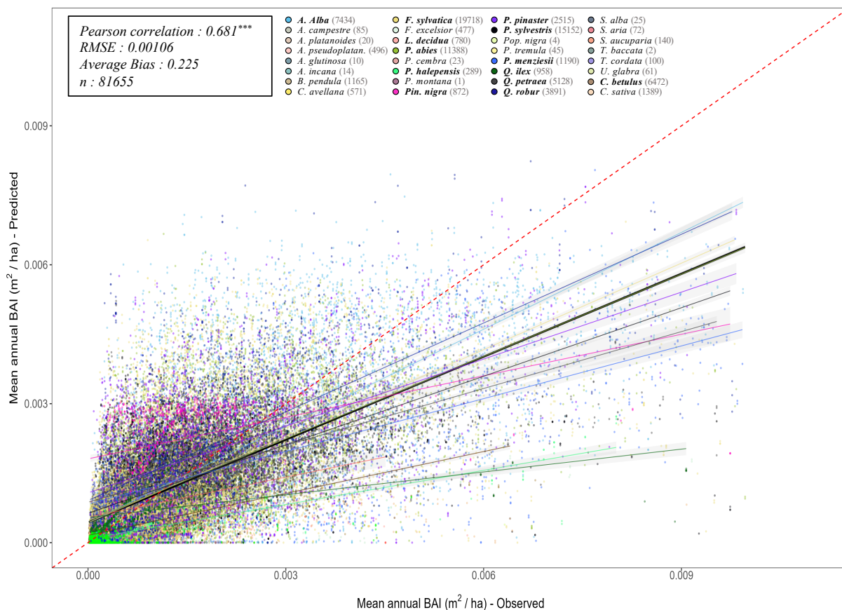
Figure Y1 | Projected (by PHOREAU) against observed mean annual tree basal increments (BAI) for all simulated trees over the 340 RENECOFOR and ICP II validation inventories. Tree points are color coded by species (see legend above). The dashed red-line is the 1:1 line; other full lines represent the regression lines of the linear model between observed and predicted tree productivity, with confidence intervals represented by the grey shaded area (in black the overall regression; coloured lines for species-specific regressions). Species-specific regressions are only shown for stand dominant species (in bold in legend). Associated statistics for the global simulation in top left, while species-specific statistics can be found in Table S1.
