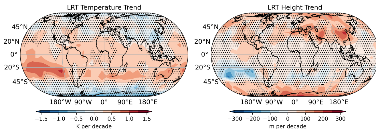
Figure 2. Observed trends in lapse rate temperature (left) and height (right), from 2002 to 2024, in 10^\circ \times 10^\circ horizontal resolution. Stippled areas are regions which are not significant at the 95% level.
