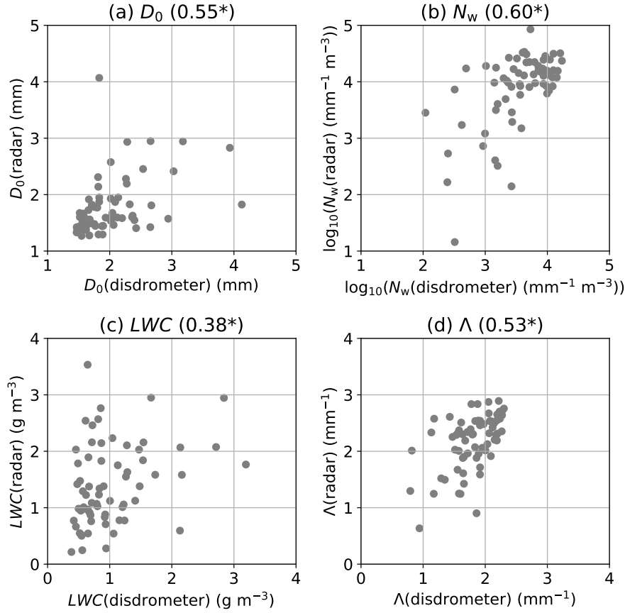
Figure 3. The scatter diagram of the drop size distribution parameters of median volume diameter ( D_0 ; mm), generalised intercept parameter ( N_w ; mm -1 m -3 ), liquid water content ( LWC ; g m -3 ), and slope parameter ( \Lambda ; mm -1 ) retrieved from Tokyo radar data against the disdrometer data at Kumagaya. Correlation coefficient values are displayed each panel and an asterisk * is added if the p -value for the correlation coefficient is less than 0.05.
