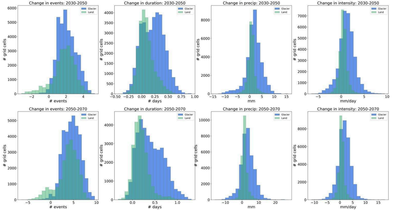
Figure 7: Spatial distribution of change in ROS frequency, duration, total precipitation and mean intensity for 2030-2050 (upper row) and 2050-2070 (lower row) shown for land and glaciers separately.
