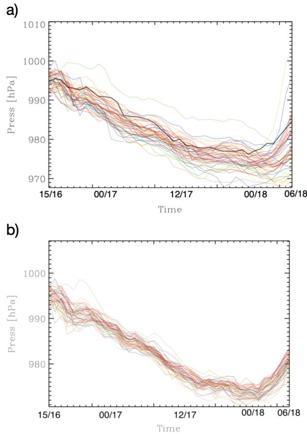
Figure 6. Time variation of minimum sea level pressure for a) the background ensemble; b) the WIV_{3h} experiment. The black line in panel a) is the minimum sea level pressure of member 42.
