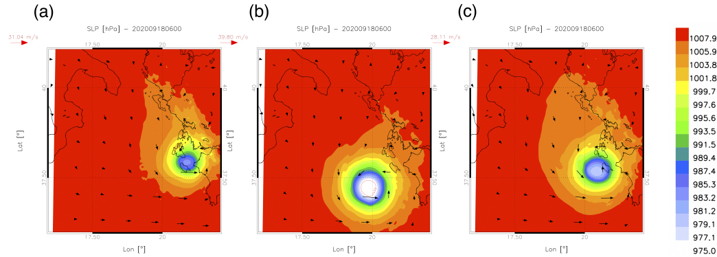
Figure 10. Sea level pressure and surface winds (every 20 grid points) at 06 UTC on 18 September for a) member 42; b) member 10, c) member 10 after the assimilation of WIVERN winds at 12 UTC on 17 September. The panels refer at 06 UTC on 18 September, i.e. 18 h after the assimilation time. The contour inside the Medcane eye in panel b) corresponds to the 975 hPa isobar.
