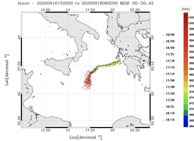
Figure 5. Trajectory followed by the WRF ensemble when WIVERN DA is applied every 3 h. The member in black is the representative member 42.
