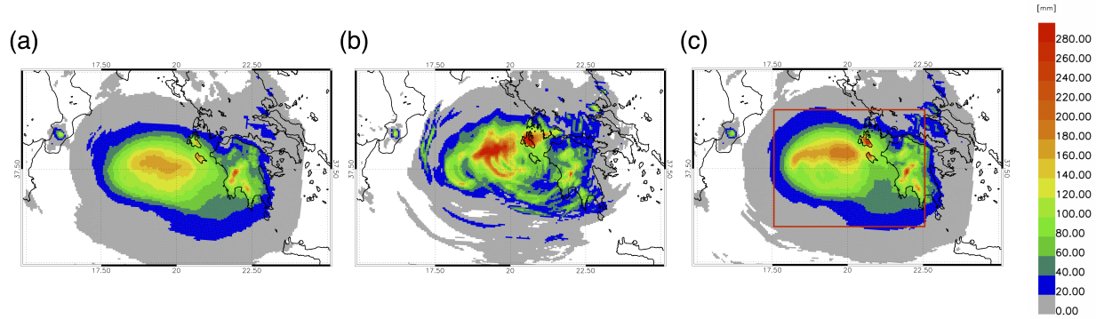
Figure 11. Rainfall accumulated from the 12 UTC on 17 September to 12 UTC on 18 September by: a) the CTRL ensemble (average); b) the representative member 42; c) the WIV 24h ensemble (average).
