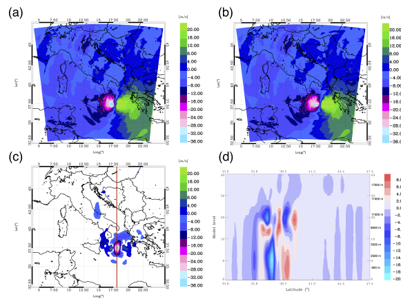
Figure 9. Analysis of wind components at 12 UTC on 17 September 2020 for member 10: a) background meridional wind component at about 2500 m a.s.l; b) analysis of the meridional wind component at about 2500 m a.s.l; c) difference between analysis and background fields of the meridional wind component (same level of panels a-b); d) cross-section of the difference between the analysis and the background of the zonal wind component along the red line of panel c). The y-axis of panel d) shows the vertical levels and labels on the right y-axis correspond to the approximate height of the levels.
