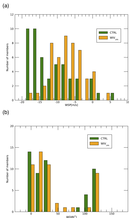
Figure 12. Distribution of the errors of the ensemble members for the surface winds at Kefalonia for CTRL and WIV 24h . Errors are computed compared to member 42 at the 06 UTC on 18 September for a) wind speed; b) wind direction. The histogram bins are 2.0 \text{ ms}^{-1} for the wind speed and 15^\circ for the direction.
