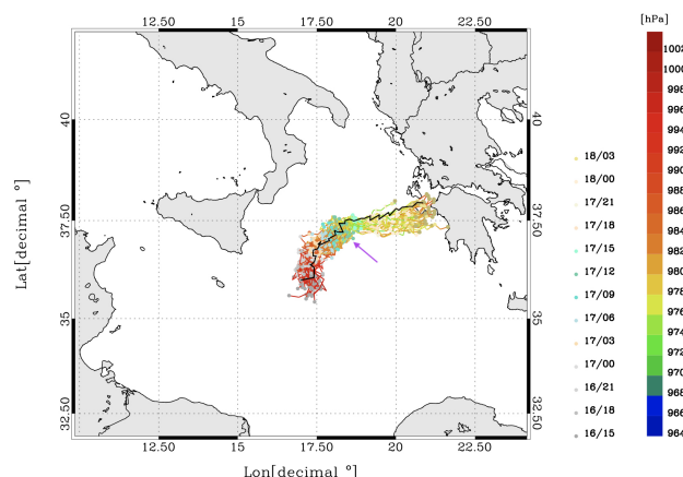
Figure 7. Trajectories followed by the members of the WRF ensemble WIV_{24h} . The trajectory in black is the representative member 42, while the violet arrow indicates the assimilation time.
