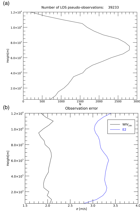
Figure 4. a) Vertical distribution of the number of WIVERN observations; b) Vertical average of the observations' error (black curve) and of the model error (blue curve). The model error is also used as observation error in the sensitivity experiment with inflated observation error.
