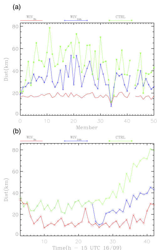
Figure 8. Average error of the ensembles CTRL , WIV 24h , and WIV 3h as function of a) the member; and, b) the time. In the panel b), diamonds are shown every 3h while the square is every 24h from the simulation start.
