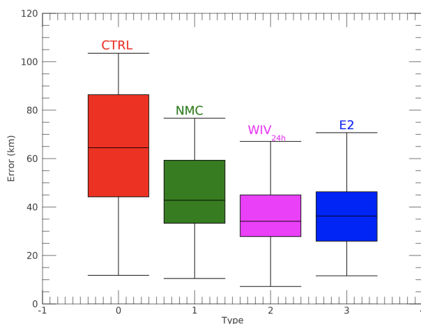
Figure 13. Trajectories error distribution, respect to the representative member 42, of the ensembles CTRL , NMC , WIV_{24h} and E2 . The boxes show the 25 th and the 75 th percentile, the black line inside the box is the median and the maximum and minimum values are the extremes of the error bar.
