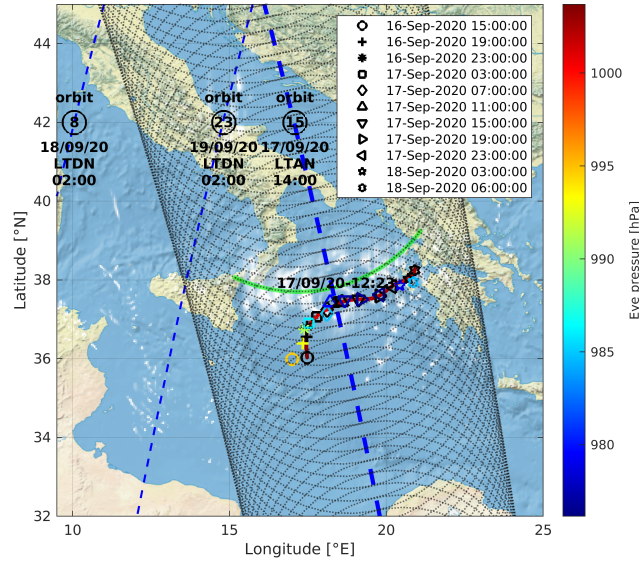
Figure 1. WIVERN track for the Medicanne Ianos. The a-posteriori best estimated trajectory is shown by the red-line, the reference trajectory is shown by symbols. The time range of the trajectories is indicated in the legend. The surface pressure along the track is shown by the color (both line and marks). The WIVERN sub-satellite point is represented by the blue dashed line, while the radar conical scan is shown by the gray dashed line, showing the 800 km wide swath. Times are indicated in local time (UTC+2h) ascending/descending node. The passages of WIVERN over the area would have occurred at 00 UTC on 18 and 19 September 2020 and at 12 UTC on 17 September 2020, however, only the 12 UTC observations would have sampled Ianos at about the center of the scene.
