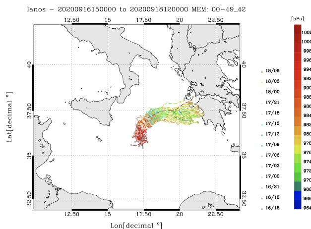
Figure 2. Trajectories followed by the ensemble members of the WRF control ensemble.
