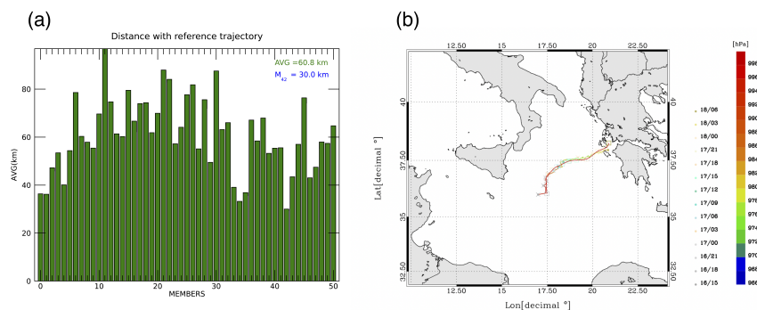
Figure 3. a) Histogram of the distances between the WRF ensemble members at the Ianos best estimated trajectory. The average distance is 60.8 km, while the minimum distance is achieved by the member 42 (30.0 km); b) trajectories of the best a-posteriori estimated trajectory of Ianos (red curve) and the representative member 42.
