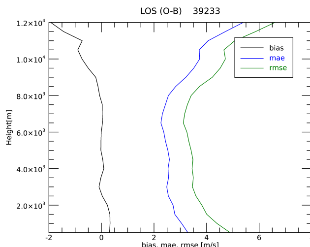
Figure 14. Observation minus background errors [m/s] for the winds along the line of sight as a function of the vertical levels.
