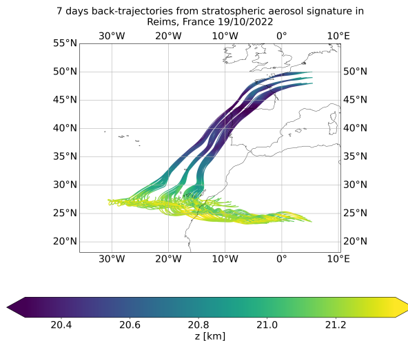
Figure 3. Simulation depicting the backward trajectories of 63 air parcels over 7 days with hourly outputs using CLAMS. The air parcels originate from a region defined as a box spanning 48^{\circ} – 50^{\circ} N and 3^{\circ} – 5^{\circ} E at 20.6 km altitude. Colors represent the corresponding altitude levels.
