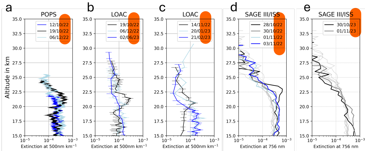
Figure 2. (a) POPS in situ aerosol partial extinction observations for the plume signal from Reims, France 19/10/2022 at 49°N and 4°E and comparison flights for background measurements on 06/12/2022 (Orleans, France, 47.8°N, 1.9°E) and 12/10/2022 (Reims); (b) Respective LOAC v1.5 observations, including background measurements on 02/06/2023 (Orleans, France, 47.8°N, 1.9°E); (c) LOAC observations of aerosol plumes of volcanic origin from MeteoModem, France 48.3°N, 2.6°E; (d) and (e) SAGE III/ISS aerosol extinction profiles (756 nm) within around 250 km of the in situ measurement locations. Panel (d) shows profiles from the same year as the in situ observations, while panel (e) presents profiles from one year later. Light grey lines in (d) and (e) indicate background profiles observed in October 2018 above central Europe.
