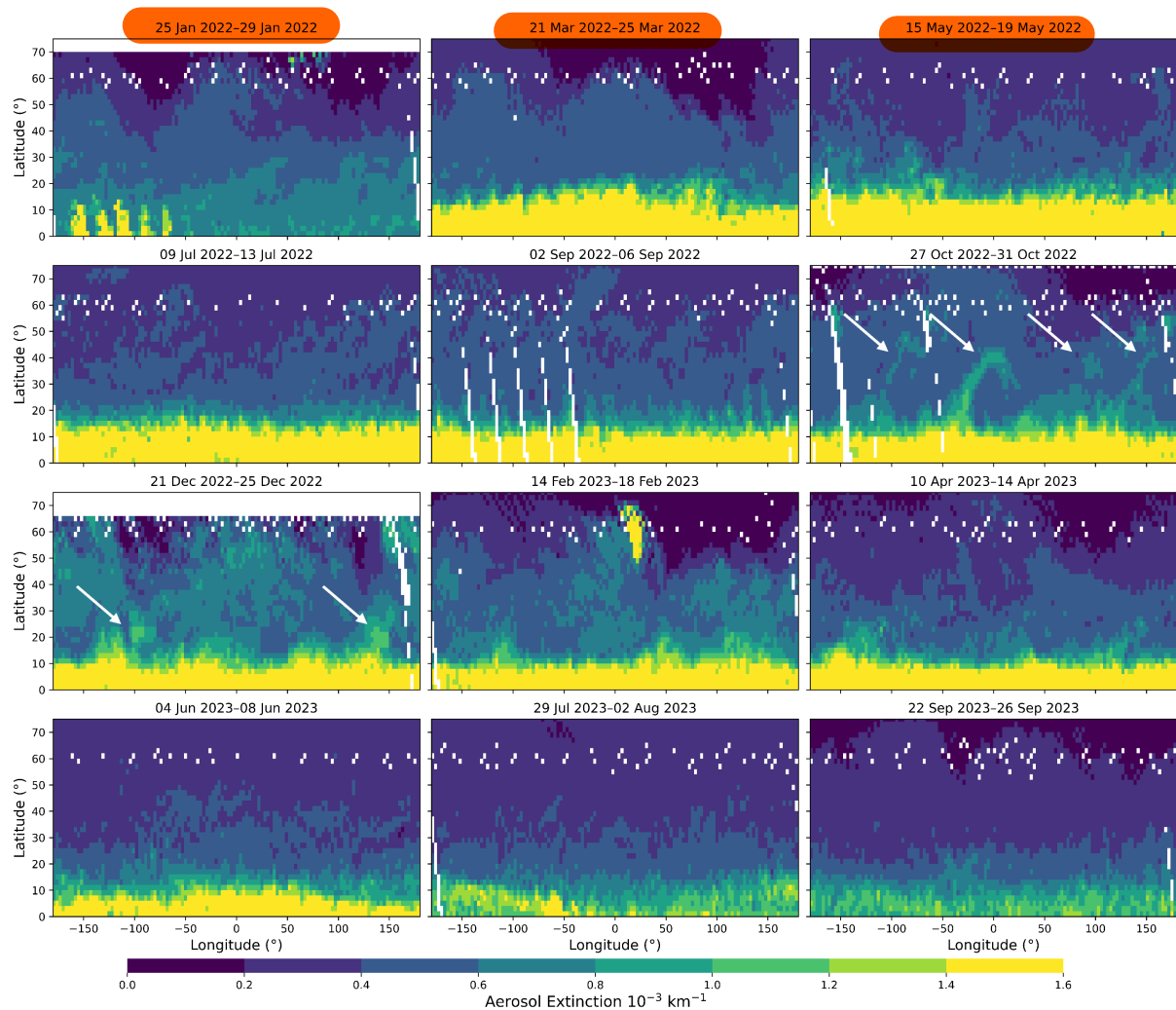
Figure 6. Five-day mean aerosol extinction at 675 nm from OMPS at 21–22 km altitude, binned to 2^\circ (latitude) \times 3^\circ (longitude) from January 2022 to January 2024. Each panel shows the period indicated in the title. The arrows point to clearly identifiable plume patches. The respective detailed transport is shown in the supplementary material video https://zenodo.org/records/15343728 .
