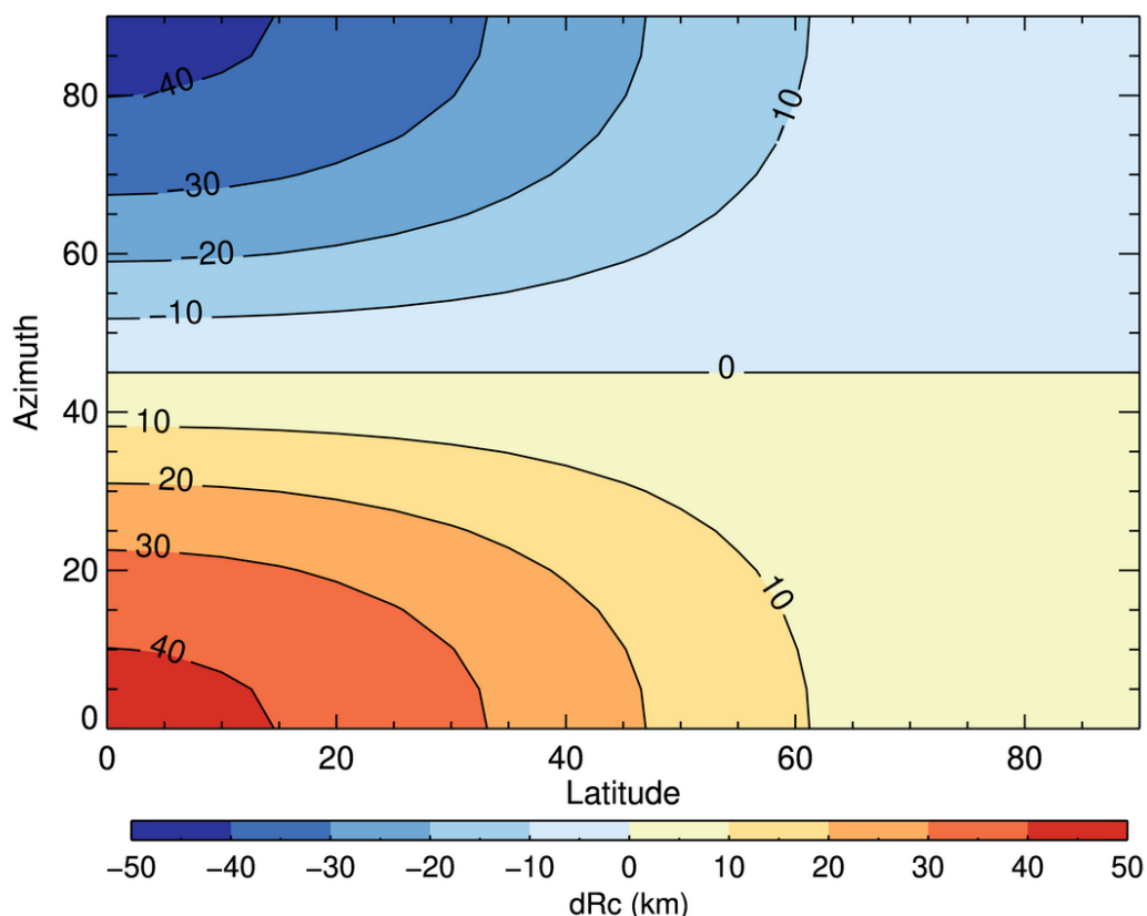
Fig. 18: Difference in radius of curvature ( dR_c in km) across minus along ray path as a function of latitude (x-axis) and occultation plane azimuth angles (y-axis).
