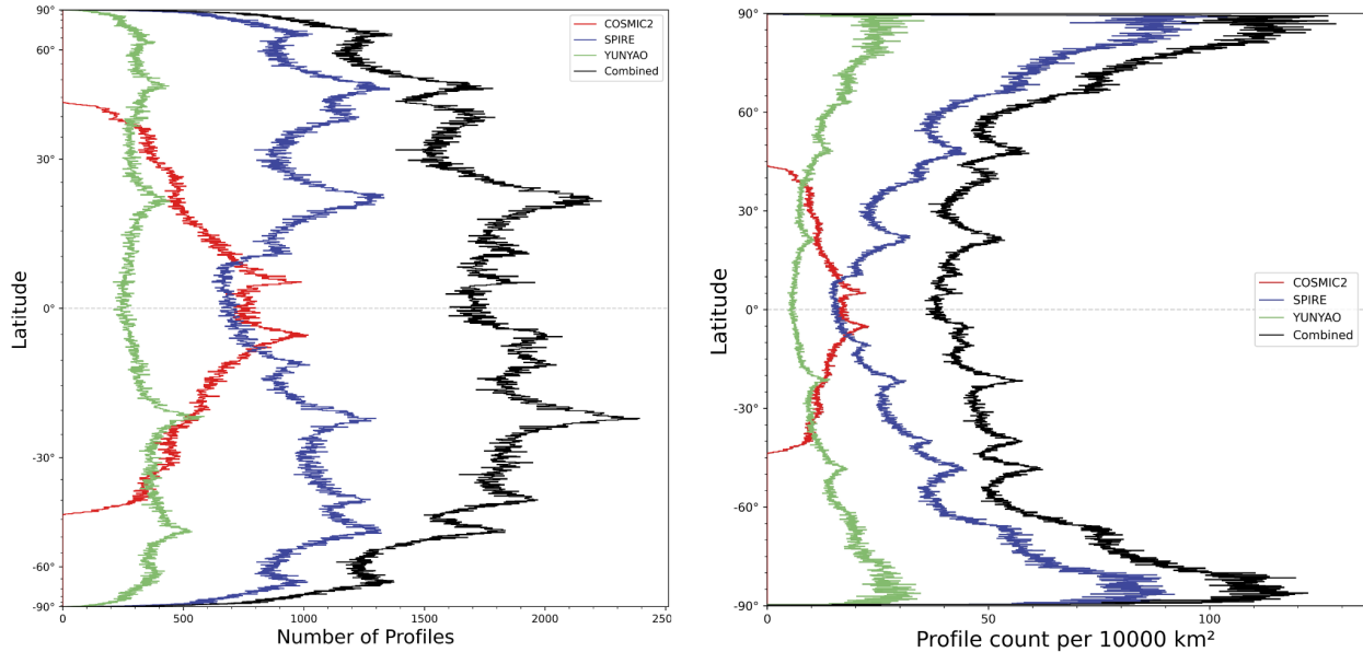
Fig. 1e: Number of profiles over the 3-month ROMEX period (x-axis) in 0.1° latitude bins for C2 (red), Spire (blue), Yunyao (green), and combined CSY (black). The panel on the left is count vs. \cos(\text{latitude}) . Panel on right is count per 10,000 square km vs. latitude.
