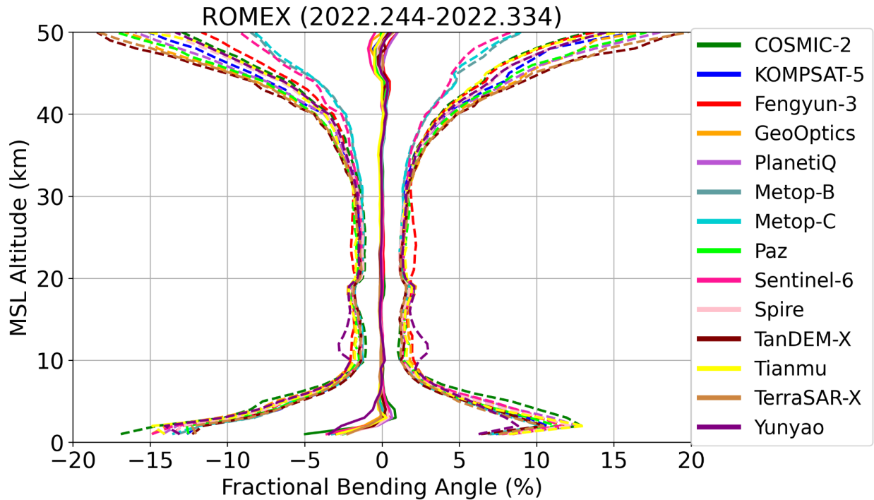
Fig. 5: Biases and standard deviations of differences from ECMWF analysis for all ROMEX missions. All latitudes are included. Figure prepared by Hannah Veitel.
