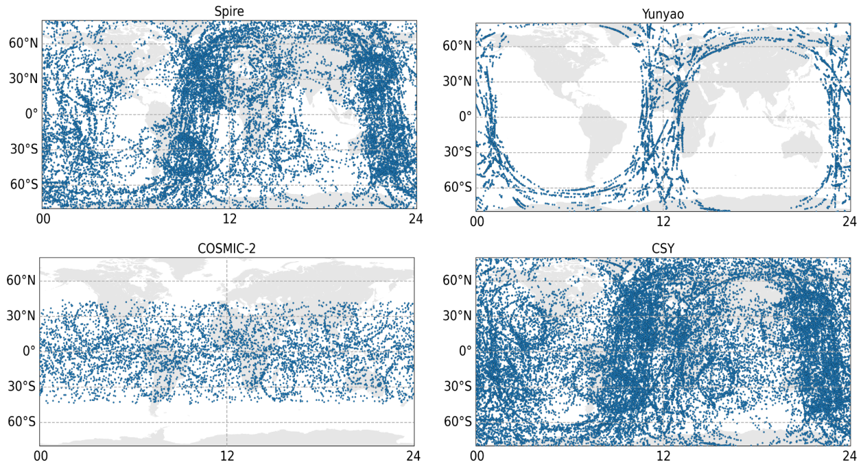
Fig. 1a: Local time coverage of Spire, Yunyao, COSMIC-2, and CSY (combined COSMIC-2, Spire and Yunyao) for 1 September 2022. The x-axes are local time in hours. These are UCAR-processed data that have passed the CDAAC (COSMIC Data
