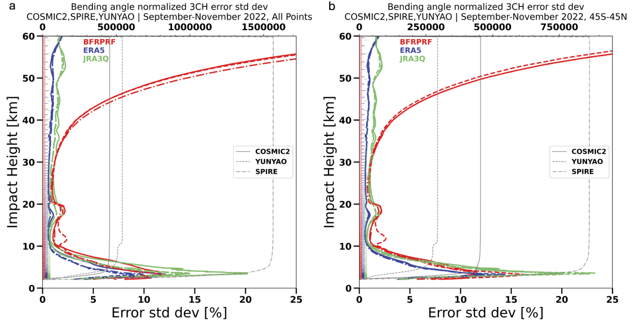
Fig. 8: 3CH BA uncertainties for COSMIC-2 (red solid), Spire (red dash-dotted), and Yunyao (red dashed), and the two corners of the 3CH method ERA5 (blue) and JRA-3Q (green). There are three estimates for the error variances of ERA5 and JRA-3Q, one for each RO mission; the differences are small and not visible in this plot. The dataset for all latitudes is shown in the left panel; the dataset for 45°NS is on the right. BFRPRF refers to the three RO missions. Above 30 km the Yunyao and C2 profiles are nearly indistinguishable in the left panel and in the right panel Spire and C2 are nearly indistinguishable, which illustrates the closeness of these three datasets at these levels.
