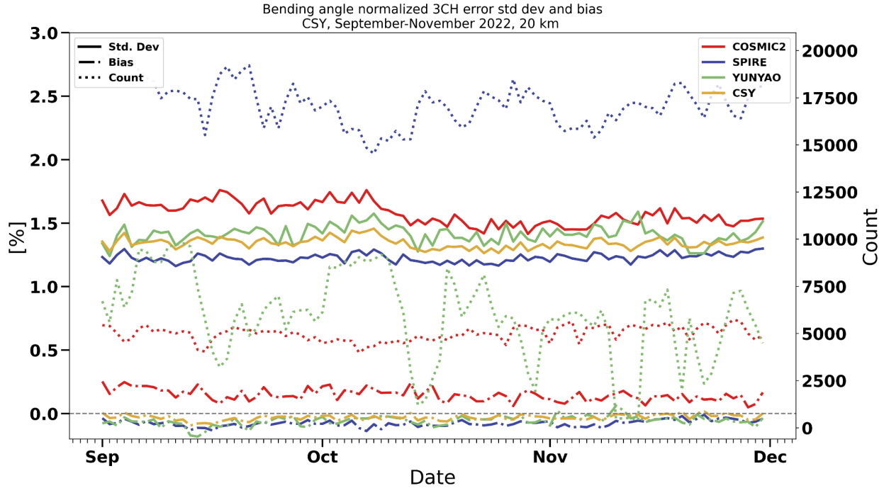
Fig. 2: Number of occultations per day (dotted lines) and error statistics (uncertainties in solid and biases with respect to ERA5 in dot-dashed) of BA for C2 (red), Spire (blue), Yunyao (green), and CSY (orange) at 20 km. The CSY daily counts are not shown. The uncertainties and biases are normalized by the sample mean of ERA5.
