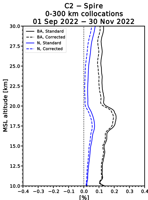
Fig. 19: Bias of C2 BA (black) and N (blue) relative to Spire for UCAR standard (solid) and sideways sliding-corrected data (dashed). C2 and Spire data for this comparison
