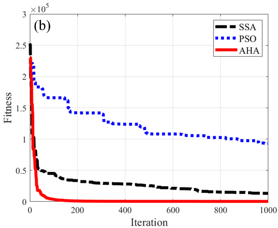
Figure 7. Convergence curves of the sparrow search algorithm (SSA), particle swarm optimization (PSO), and artificial hummingbird algorithm (AHA) applied to case study. (a) case study 1; (b) case study 2.
