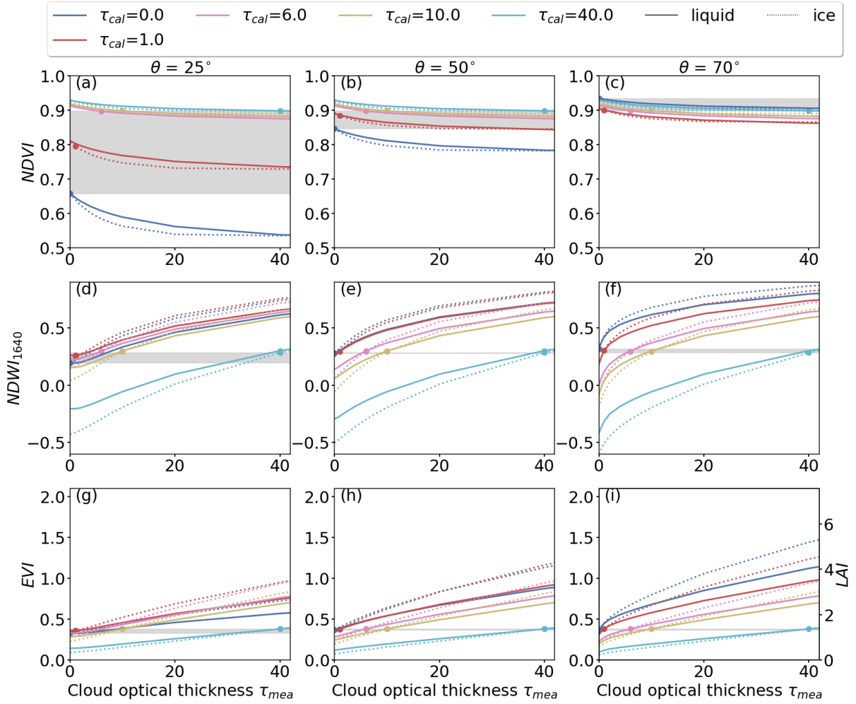
Figure A1. Same as Fig. 6 but for the erectophyll leaf angle distribution.
