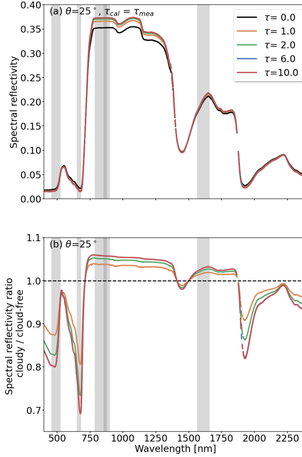
Figure 2. (a) Simulated spectral reflectivity -reflectance \rho(\lambda) caused by an ice cloud for a solar zenith angle \theta of 25°, and constant cloud optical thickness during calibration and the actual synthetic measurements ( \tau_{cal} = \tau_{mea} ). The simulations base on a spherical LAD. (b) Ratios of spectral reflectivity -reflectance with \tau_{cal} = \tau_{cal} > 0 with respect to the spectral reflectivity -reflectance under cloud-free conditions. Panels (a) and (b) share the same legend. The gray marked areas highlight the Sentinel-2 bands B2, B4, B8, B8a, and B11.
