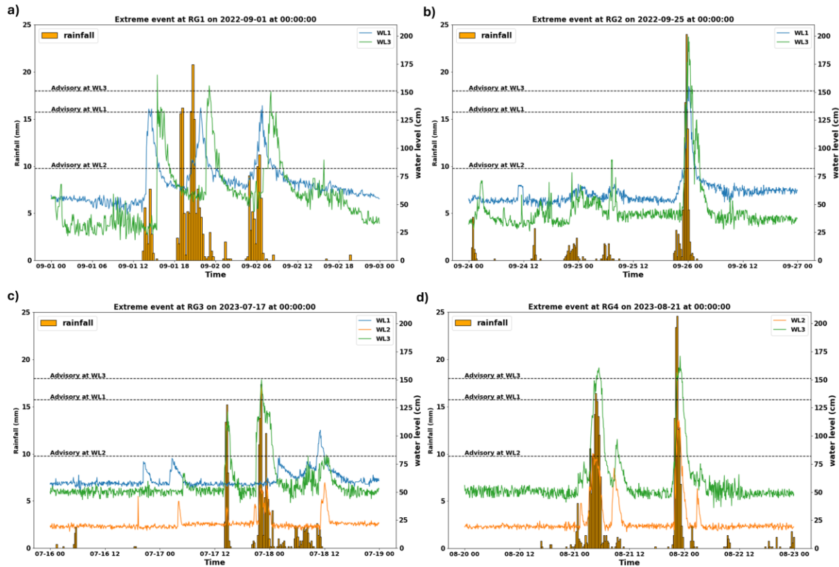
Figure 8: The response of water level sensors WL1, WL2, and WL3 to extreme rainfall events in the watershed, highlighting the variability in watershed dynamics. Advisory thresholds for water level alerts are indicated for each site (black dashed line). Panels a) to d) correspond to extreme rainfall events on different dates, showing the water level response and rainfall data from RG1 to RG4, respectively.
