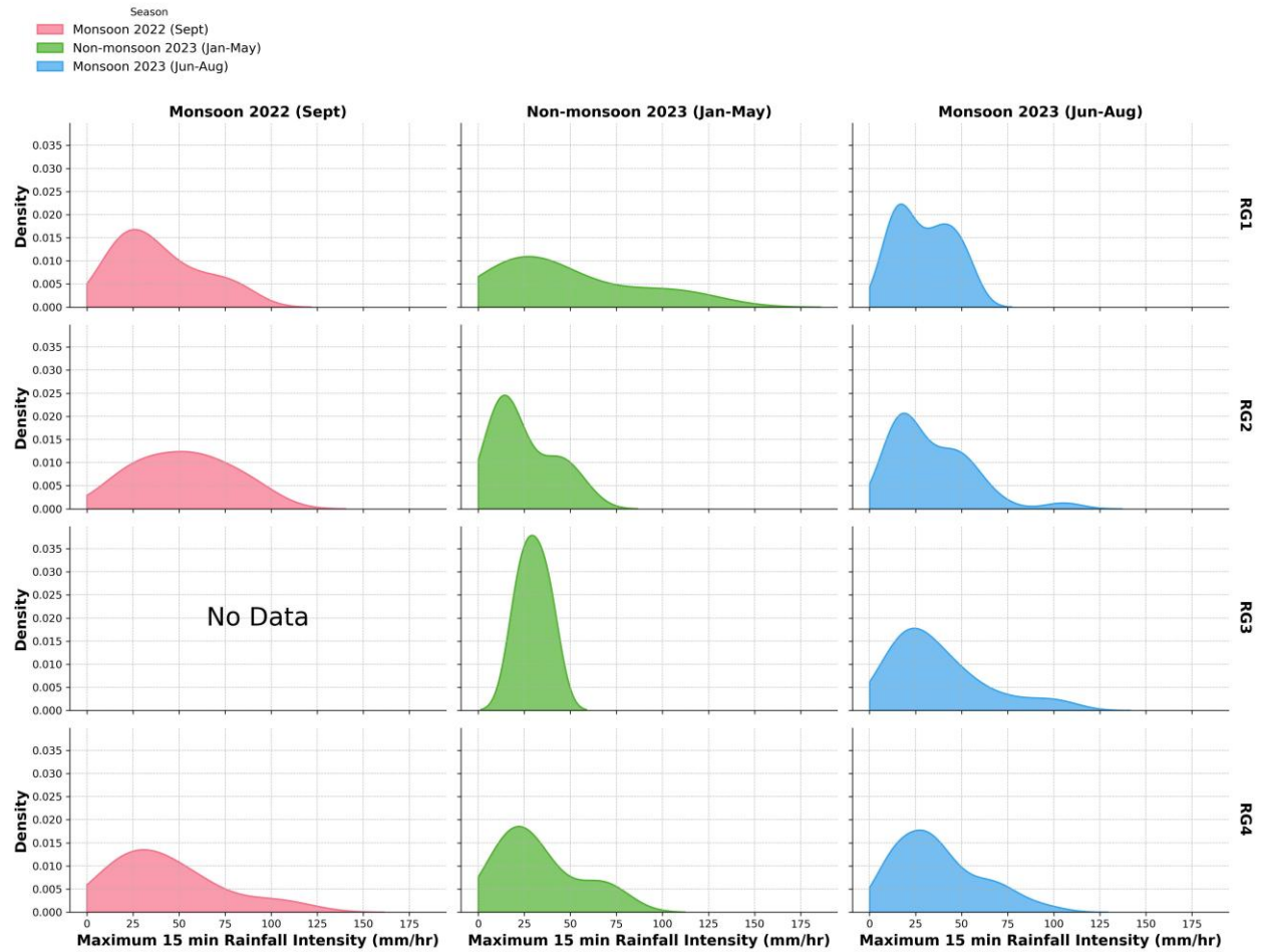
Figure 7: Density plots showing the distribution of maximum 15-minute rainfall intensities (mm/h) observed at various rain gauges across different seasons within the watershed. The plots highlight distinct seasonal patterns, with notable differences between monsoon and non-monsoon periods, and variations in intensity magnitudes across gauges and downstream locations.
