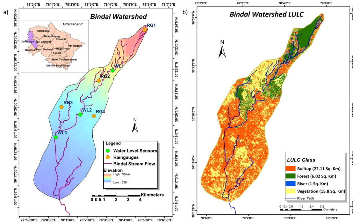
Figure 1: Bindal Watershed. a) Map of Bindal watershed with sensor locations, i.e., rain gauges: RG1, RG2, RG3, RG4, and river water level recorders: WL1, WL2, and WL3; The inset map illustrates the location of the watershed within the broader Dehradun district boundary (shaded purple) in Uttarakhand state to provide regional geographical context. b) Land Use/Land Cover (LULC) classification of the Bindal watershed highlights the dominance of built-up areas ( 22.11 \text{ km}^2 ) and vegetation ( 15.8 \text{ km}^2 ) across the 44.4 \text{ km}^2 Watershed.
