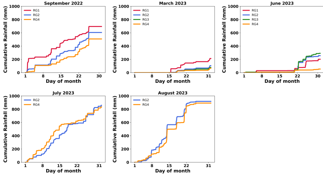
Figure 4: Cumulative plot of monthly observed rainfall across different rain gauges in the watershed (only months with more than 200 mm of cumulative rainfall are shown), illustrating spatial variability in rainfall. Higher elevations generally receive more rainfall than lower elevations. Additional plots for all months (September 2022–August 2023) are provided in the Supplementary Information (Figure S1).
