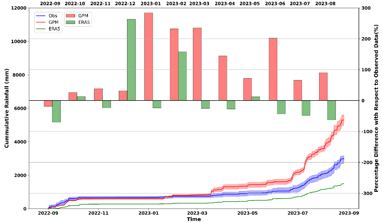
Figure 6 Comparison of cumulative rainfall and monthly percentage differences between observed gauge data (Obs), GPM, and ERA5 datasets from September 2022 to August 2023. The lower panel shows cumulative rainfall ($mm$), where the solid lines represent the spatial average and the shaded regions indicate the range between the minimum and maximum rainfall values across all pixels and gauges within the basin. The upper panel displays the monthly percentage difference of GPM (red bars) and ERA5 (green bars) relative to the observed data.
