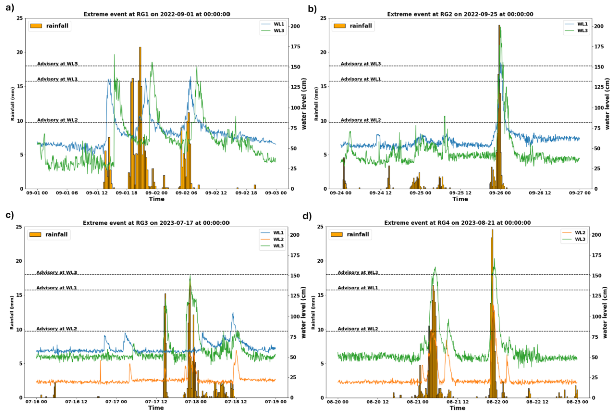
Figure 8 The response of water level sensors WL1, WL2, and WL3 to extreme rainfall events in the watershed, highlighting the variability in watershed dynamics. Advisory thresholds for water level alerts are indicated for each site (black dashed line). Panels a) to d) correspond to extreme rainfall events on different dates, showing the water level response and rainfall data from RG1 to RG4, respectively.
