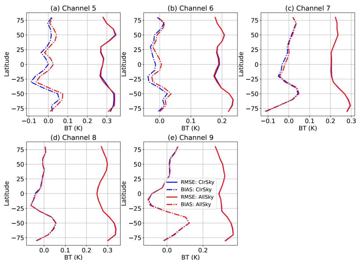
Figure 6. RMS (solid line) and mean (dashed line) of the observations minus ensemble mean background (i.e., OMB), binned by latitude, for bias-corrected clear-sky radiances from NOAA 15 AMSU-A: (a) channel 5, (b) channel 6, (c) channel 7, (d) channel 8, and (e) channel 9, for ClrSky (blue) and AllSky (red). Statistics are calculated globally every 6 hours from 0000 UTC 18 April to 1200 UTC 14 May 2018, using 10° latitude bins.
