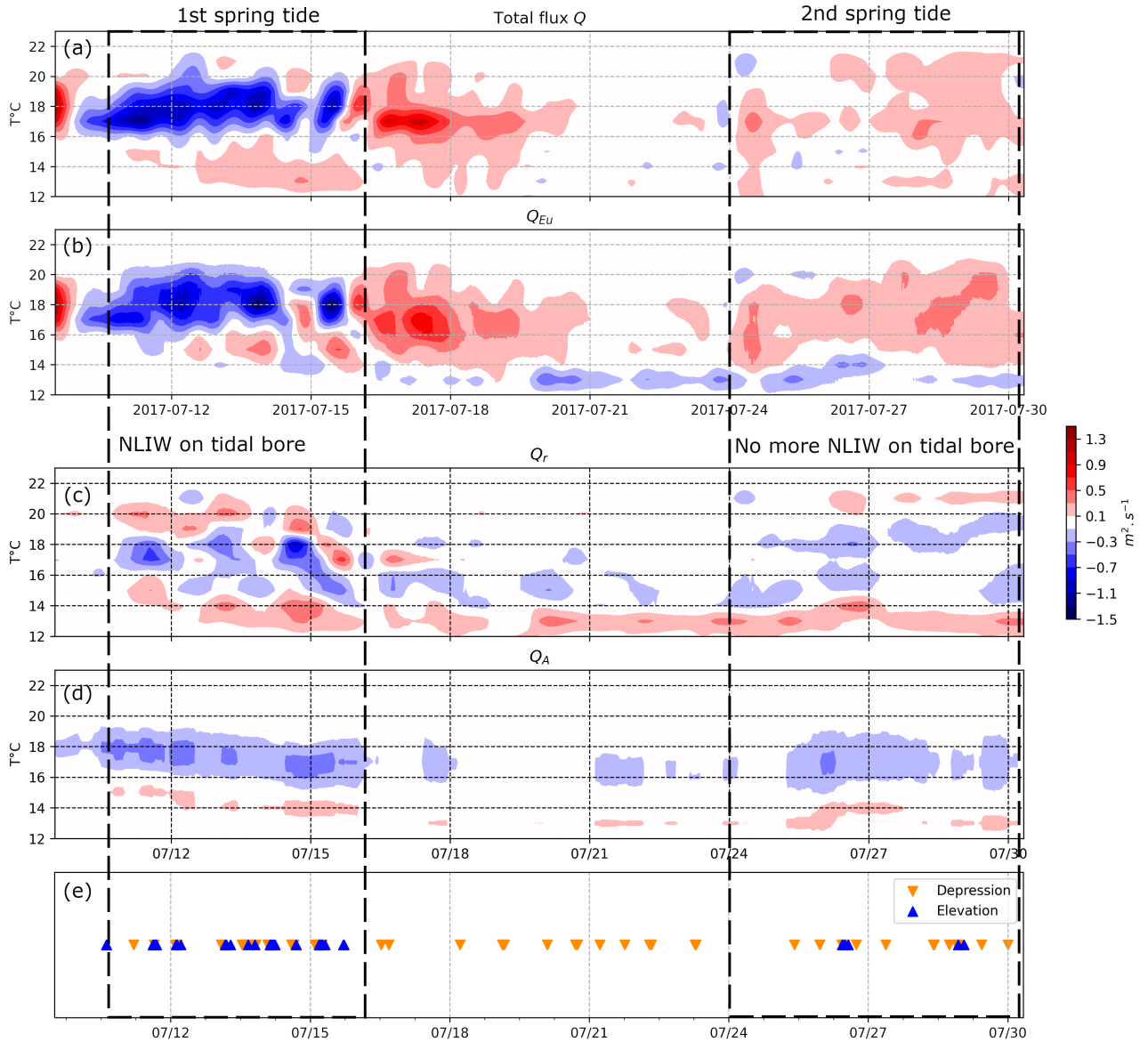
Figure 8. SE-BoB fluxes and NLIWs from July 09 to July 30. Colors indicate the direction of volume flux. Red is onshore volume flux and blue offshore. (a) Total net cross-shelf volume flux Q . (b) Subtidal volume flux Q_{Eu} . (c) Stokes drift volume flux Q_r (see definition in section 2.3). (d) Theoretical Stokes volume flux for a linear, M2, mode 1 internal tide Q_A as defined in section 2.3. (e) NLIWs, blue triangles correspond to mode 1 NLIWs of elevation, orange downward triangles show mode 1 NLIWs of depression.
