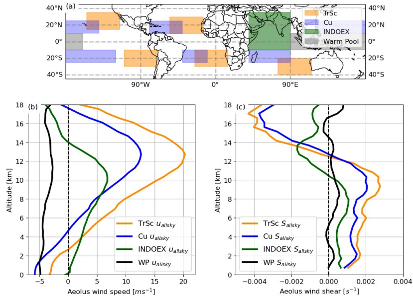
Figure 11: (a) map of the different regions considered. Average (b) wind speed profiles and (c) wind shear profiles retrieved in each region during the year 2020. The wind shear S_{\text{allsky}}(z) is computed at each altitude z using the u_{\text{allsky}}(z_1) observed 1 km below z and at u_{\text{allsky}}(z_2) observed 1 km above z , following Eq. 4.
