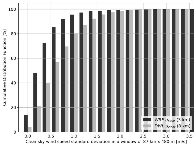
Figure B3: Same as Fig. 5 but all altitudes between the surface and 19 km are included for WRF (about 4000 independent segments of 87 km x 480 m).
