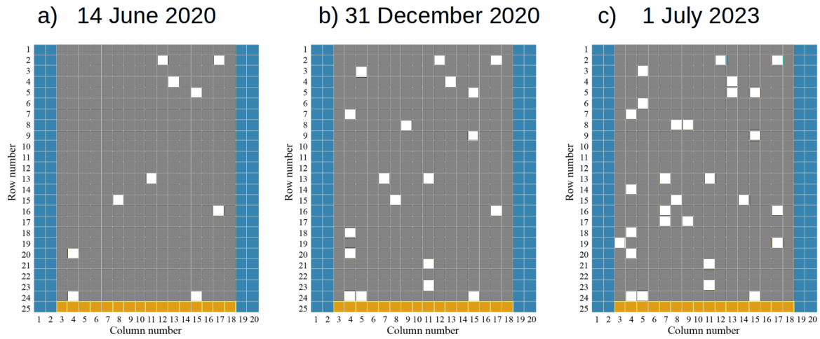
930 Figure A2. Hot pixel maps corresponding to (a) 14 June 2020 (compare with Weiler et al., 2021), (b) 31 December 2020 (end of our 935 study) and 1 July 2023 (end of Aeolus mission). Hot pixels are denoted in white, regular pixels in gray. Hot pixels are identified by comparing each detector pixel value against its immediate neighbors within the same Mie detector row: pixels exceeding all neighboring values are flagged and counted across all daily orbits. The resulting frequency maps are normalized by their maximum count and thresholded at 0.2, with pixels above this empirical threshold marked as "hot". For our study, we used the hot pixel map of 31 December 2020 (Fig. A2b) but follow-on study based on a longer period may use the most conservative hot pixel map of 1 July 2023 (Fig. A2c).
