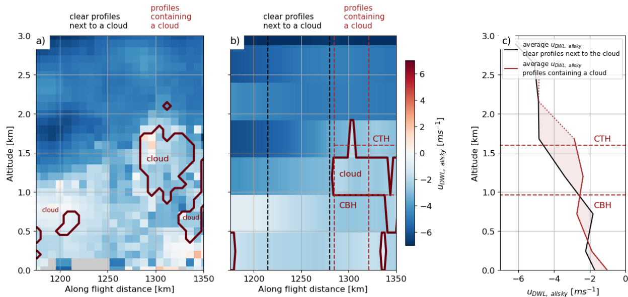
Figure 10: (a) Curtain of u_{DWL, allsky} acquired by the airborne DWL and projected along the laser pointing direction of Aeolus during the AVATAR-T campaign. (b) is the same u_{DWL, allsky} wind curtain coarsened at the resolution of our Aeolus dataset (3 km along flight direction, 480 m vertically). The cloud mask is also coarsened and clouds are represented with solid red contours. Vertical red dashed lines represent the horizontal extent of the profiles encompassing a cloud while vertical black dashed lines represent the horizontal extent of clear sky profiles next to the clouds. Horizontal red dashed lines mark the average Cloud Base Height (CBH) and Cloud Top Height (CTH) for the profiles encompassing a cloud. (c) Profiles of u_{DWL, allsky} encompassing the cloud (red curve) and in the clear sky surrounding the cloud (black curve).
