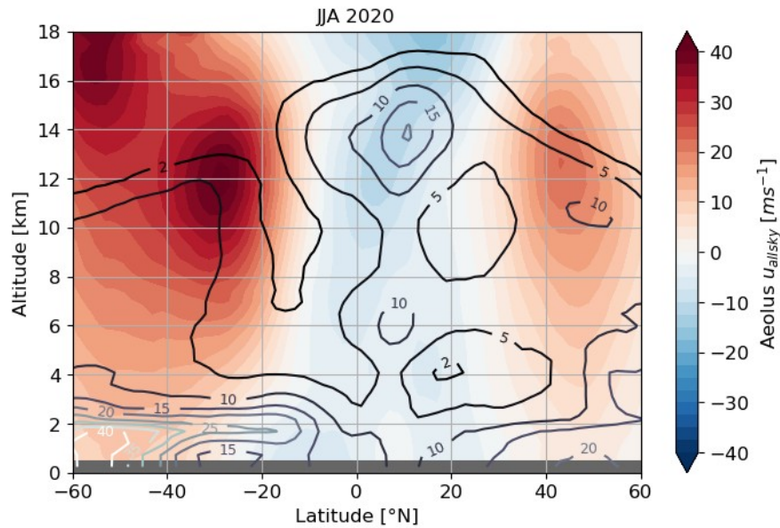
Figure 7: (a) Zonal average of all-sky wind speed profiles from June to August 2020. Contours represent the zonal average cloud fraction.
