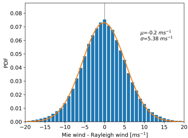
1030 Figure B2: Distribution of the differences between colocated, resampled, Mie winds retrieved in cloudy sky and Rayleigh winds that were substituted. Based on all bins during JJA 2020.
