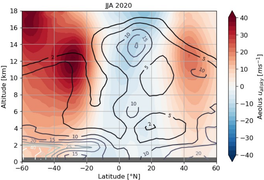
485 Figure 7: (a) Zonal average of all-sky wind speed profiles from June to August 2020. Contours represent the zonal average cloud fraction.
