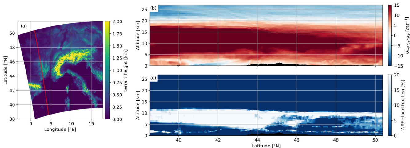
Figure B8: (a) terrain height of WRF simulation, the red curve corresponds to a theoretical orbit track of Aeolus. (b) Horizontal wind projected along Aeolus line-of-sight ( u_{WRF, \text{alsky}} ) at a horizontal resolution of 3 km and (c) the corresponding cloud fraction.
