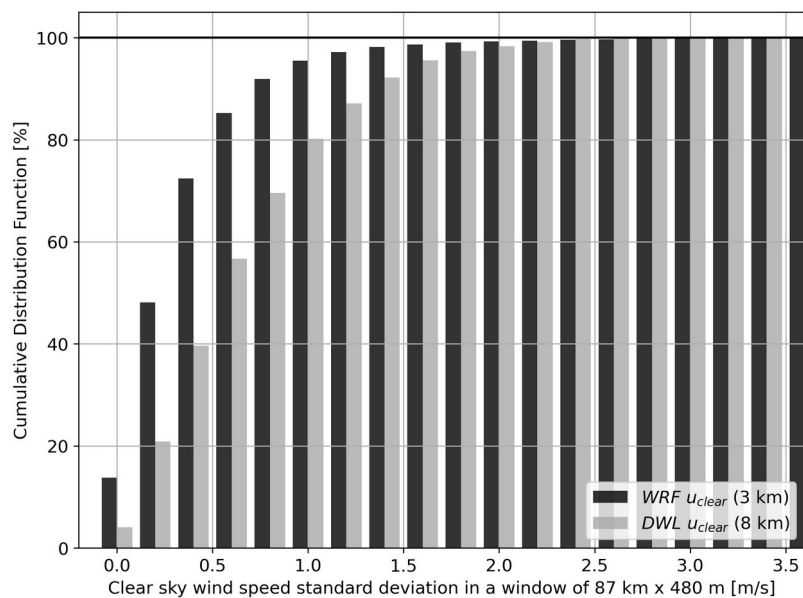
1050 Figure B3: Same as Fig. 5 but all altitudes between the surface and 19 km are included for WRF (about 4000 independent segments of 87 km x 480 m).
