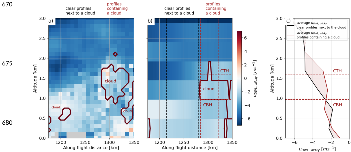
685 Figure 10: (a) Curtain of u_{DWL, allsky} acquired by the airborne DWL and projected along the laser pointing direction of Aeolus during the AVATAR-T campaign. (b) is the same u_{DWL, allsky} wind curtain coarsened at the resolution of our Aeolus dataset (3 km along flight direction, 480 m vertically). The cloud mask is also coarsened and clouds are represented with solid red contours. Vertical red dashed lines represent the horizontal extent of the profiles encompassing a cloud while vertical black dashed lines represent the horizontal extent of clear sky profiles next to the clouds. Horizontal red dashed lines mark the average Cloud Base Height (CBH) and Cloud Top Height (CTH) for the profiles encompassing a cloud. (c) Profiles of u_{DWL, allsky} encompassing the cloud (red curve) and in the clear sky surrounding the cloud (black curve).
