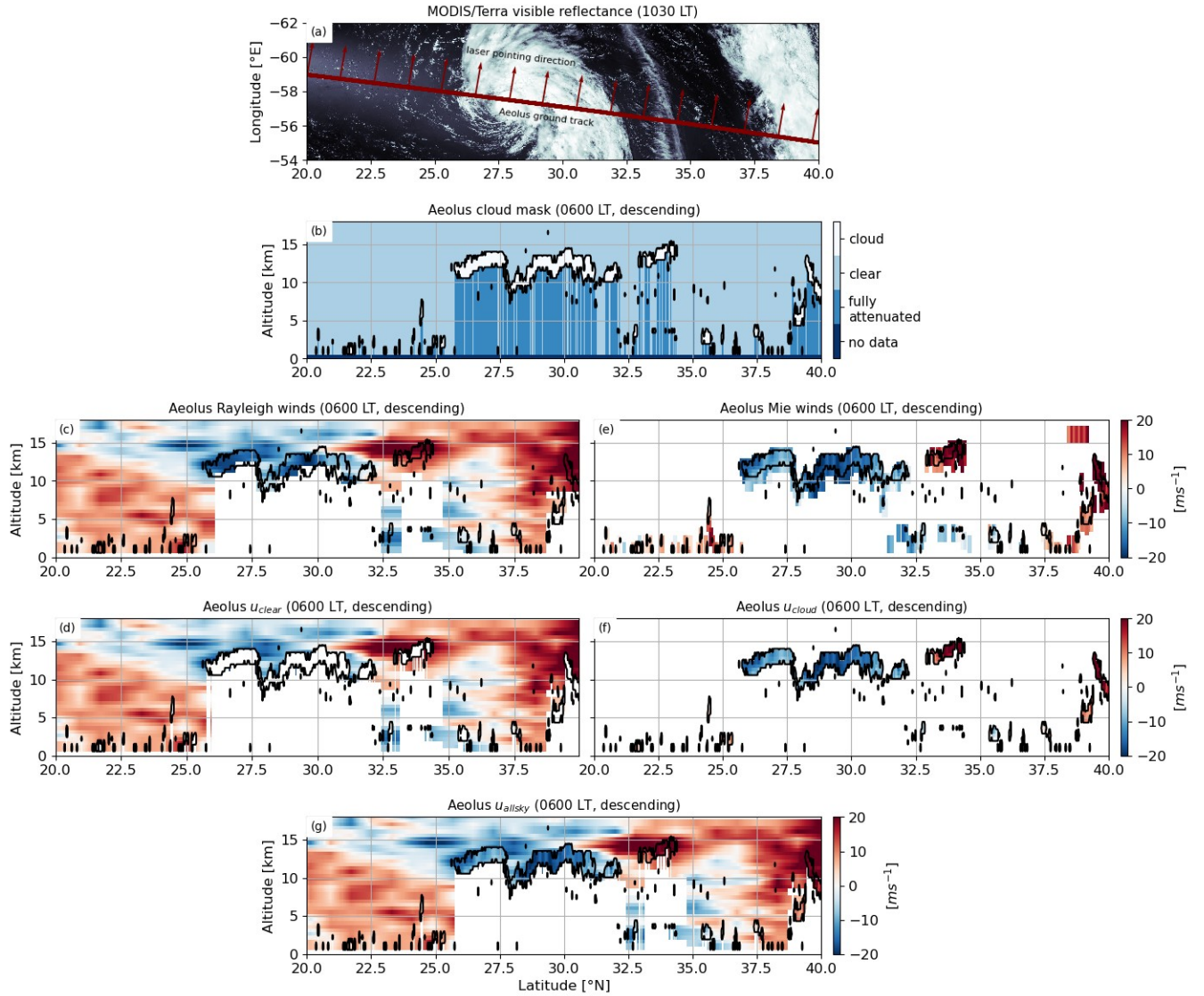
Figure 6: (a) Descending orbit segment crossing the tropical cyclone Paulette over the Atlantic ocean (2020-09-12T09–2020-09-12T11) plotted in red over a MODIS/Terra reflectance image. The red arrows represent the laser pointing direction. (b) Aeolus cloud mask. Aeolus (c) all Rayleigh winds and (d) Rayleigh winds only outside of the cloud mask, noted u_{clear} along the paper. Aeolus (e) all Mie winds, (f) Mie winds only within the cloud mask, noted u_{cloud} along the paper. (g) All-sky winds, noted u_{allsky} , result from the merging of u_{clear} and u_{cloud} . The winds are negative when blowing westward and positive when blowing eastward. For panels (b-g), the resolution of the re-sampled data is 3 km horizontally and 480 m vertically and the black contour is the cloud mask.
