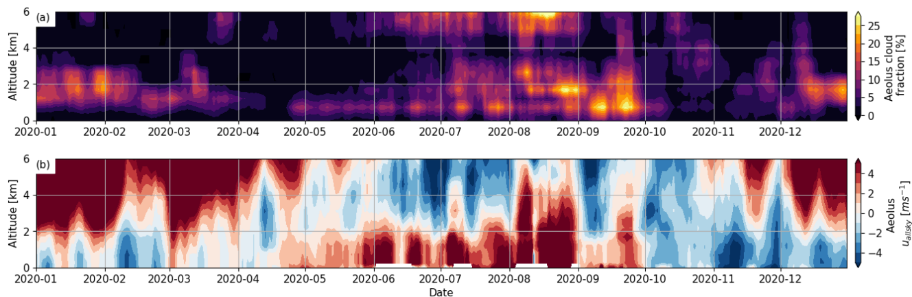
Figure B4 : Time series of (a) the average profiles of cloud fraction and (b) the average profiles of all-sky wind speed within (12°N-24°N, 55°E-75°E). A 7-day rolling mean is applied to see the typical direction of the wind and vertical cloud extent
