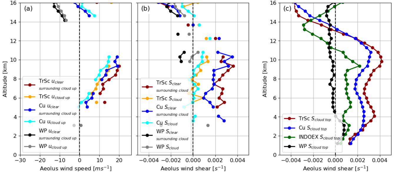
Figure 12: (a) average wind speed profiles retrieved within the uppermost cloudy layer u_{\text{cloud up}}(z) and average of the closest clear sky wind speed u_{\text{clear surrounding cloud up}}(z) observed over each region. Only values where u_{\text{cloud up}}(z) and u_{\text{clear surrounding cloud up}}(z) are significantly different (two sided T-test with p\text{-value} < 0.05 ) are plotted. (b) Average wind shear profiles within the cloud S_{\text{cloud}}(z) , and in the surrounding clear sky S_{\text{clear surrounding cloud}}(z) are computed at each altitude z using the the wind speed observed at z_1 located 1 km below z and at the wind speed observed at z_2 located 1 km above z . Note that for (a) and (b), only a sample of the data is used as each cloud should be at least 2 km thick vertically, and the horizontal distance between S_{\text{cloud}}(z) and S_{\text{clear surrounding cloud}}(z) must be < 100 km and only values where S_{\text{cloud up}}(z) and S_{\text{clear surrounding cloud up}}(z) are significantly different (two sided T-test with p\text{-value} < 0.05 ) are plotted. (c) Average cloud top wind shear S_{\text{cloud top}}(z) profiles retrieved in each region during the year 2020 using all data collected by Aeolus over each region, contrarily to (a) and (b) that only use a sample of the data.
