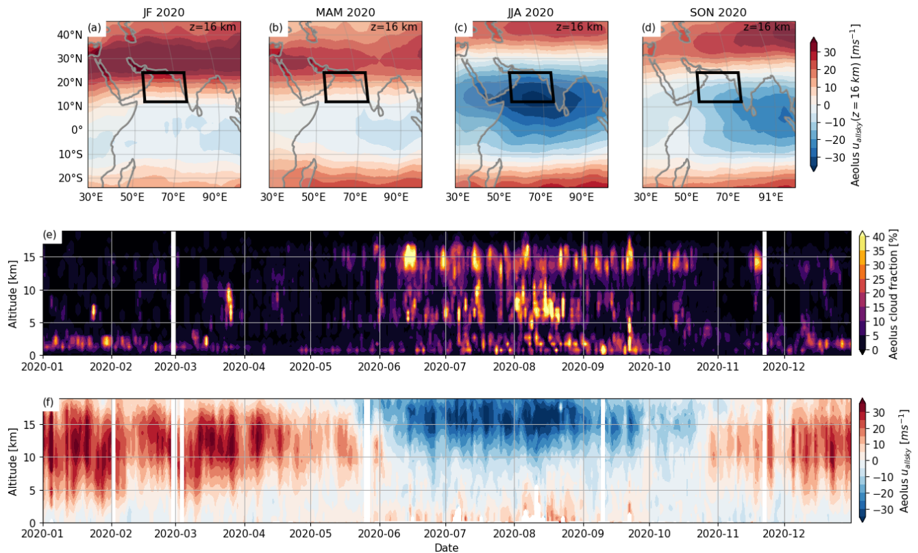
Figure 9: (a) map of the averaged all-sky wind speed u_{allsky}(z=16 \text{ km}) during the months of January and February 2020; (b, c and d) are the same for respectively March-May, June-August and September-November 2020. The rectangle (12°N-24°N, 55°E-75°E) represents a domain selected as it is under the influence of the Tropical Easterly Jet during summer. Time series at a daily resolution of (e) the average profiles of cloud fraction within the domain and (f) the average profiles of all-sky wind speed within the domain.
