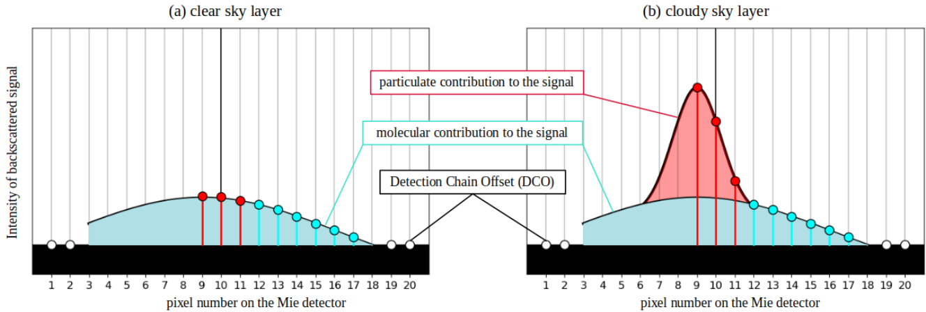
930 Figure A1. Schematics of the signal received on the detector of the Mie channel (a) in the case of a clear sky layer and (b) in the case of a cloudy layer. Note that these are not at scale and in the case of a cloudy scene, the particulate backscattered signal peak is much larger compared to the molecular backscattered spectrum.
