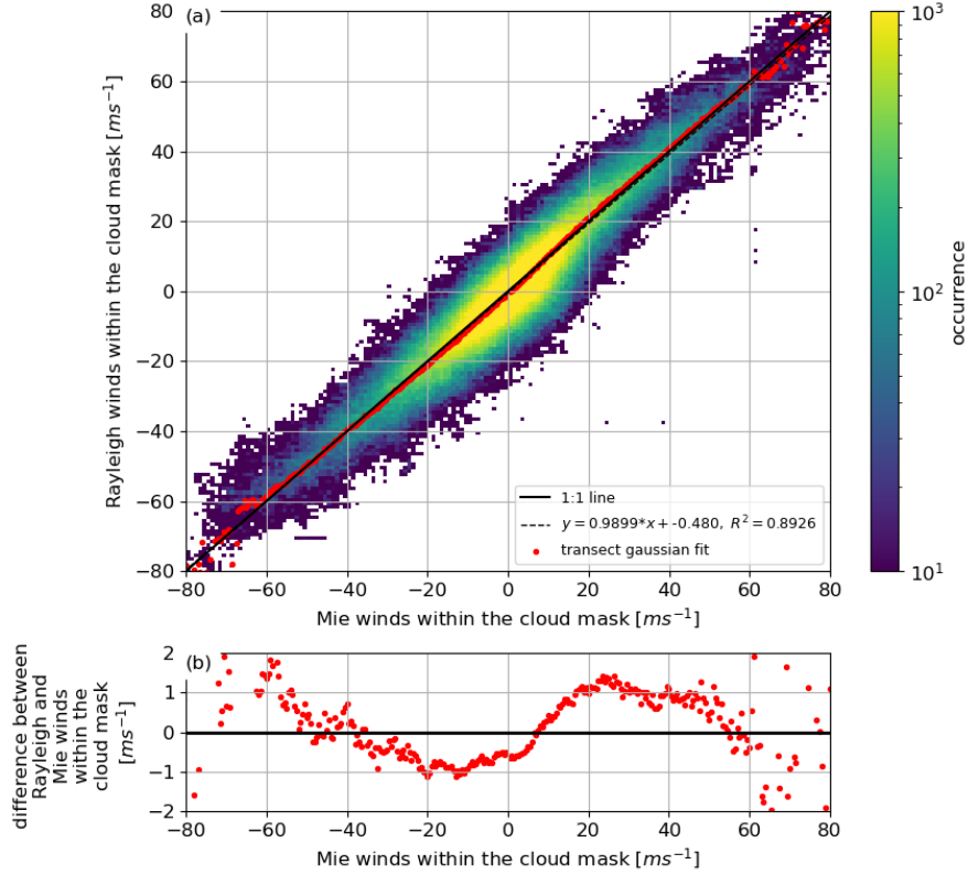
Figure 4: (a) 2D-PDF of pairs of colocated Mie winds and the Rayleigh winds when they both coexist within the cloud mask. The black dotted line represents the best linear regression. The 1:1 line is represented as a solid black line. For each point along this 1:1 line, a Gaussian was fitted to all data points lying along a perpendicular transect. Where the data spread and statistics allow a satisfactory fit, the maximum of the Gaussian is plotted as a red filled circle each 0.5 \text{ ms}^{-1} . (b) Maximum of the Gaussian of the differences between Rayleigh and Mie winds within the cloud mask as a function of the Mie winds within the cloud mask. A sample of 50 orbit files of the year 2020 are analysed with a total of 10^6 bins of 3 \text{ km} \times 480 \text{ m} where both Rayleigh and Mie winds coexist within the cloud mask.
