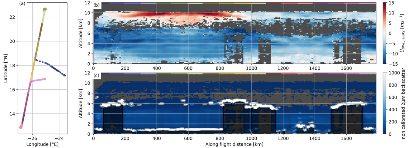
Figure B7: (a) position of airborne LIDAR profiles during AVATAR-T Flight (2021-09-08, same as Fig. 10) over Cape Verde (b) horizontal wind projected along Aeolus line-of-sight ( u_{DWL, allsky} ) at a horizontal resolution of 8 km and vertical resolution of 100 m. and (c) uncalibrated 2\mu m backscatter with clouds contoured (grey) and the sub-cloud layers shaded (black). We estimated that uncalibrated 2\mu m backscatter exceeding 500 is associated with clouds.
