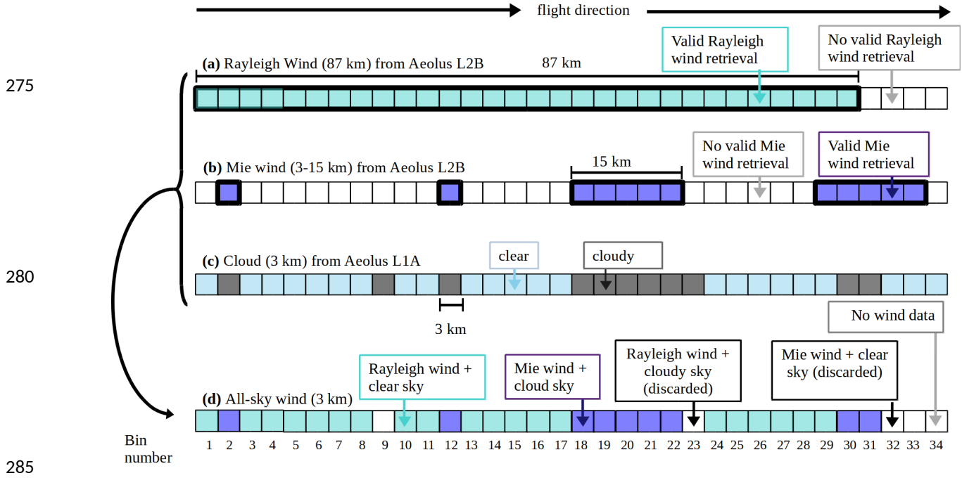
Figure 3: Building the all-sky wind along an orbit segment at one altitude level by selecting the adequate wind from Aeolus L2B based on the cloud detection. Each square represents a bin of 3 km x 480 m. (a) Blue bins contain valid wind from Aeolus L2B Rayleigh channel (87 km resolution along orbit track). (b) Purple bins contain valid wind from Aeolus L2B Mie channel (3 to 15 km resolution along orbit track). (c) Cloud detection made from Aeolus L1A (3 km resolution along orbit track). (d) Aeolus all-sky wind at 3 km along orbit track resolution, built by compositing lines (a) to (c). Blue bins contain a valid clear sky wind, purple bins contain a valid cloudy sky wind and white bins contain no wind data.
