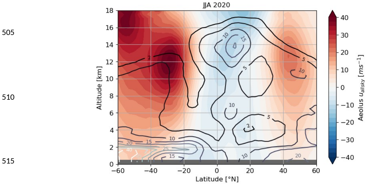
520 Figure 7: (a) Zonal average of all-sky wind speed profiles from June to August 2020. Contours represent the zonal average cloud fraction.
