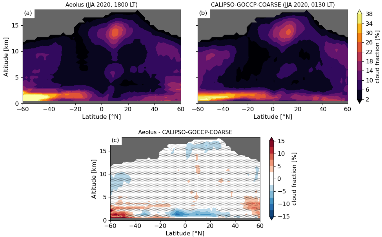
230 Figure 2: Zonal average cloud fraction profiles for (a) Aeolus at 1800 LT and (b) CALIPSO-GOCCP-COARSE at 0130 LT corrected for the diurnal cycle (c) is the absolute difference of cloud fraction between Aeolus and CALIPSO-GOCCP-COARSE. Non-significant differences (two sided T-test with p-values > 0.05) are dotted. The lowest bin encompasses the surface and is discarded in this study (opaque gray bar). Cloud fractions < 1% are masked in gray.
