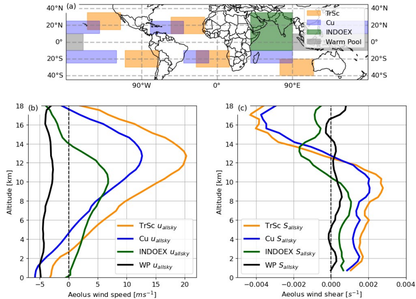
Figure 11: (a) map of the different regions considered. Average (b) wind speed profiles and (c) wind shear profiles retrieved in each region during the year 2020. The wind shear S_{\text{Aeolus}}(z) is computed at each altitude z using the u_{\text{Aeolus}}(z_1) observed 1 km below z and at u_{\text{Aeolus}}(z_2) observed 1 km above z , following Eq. 4.
