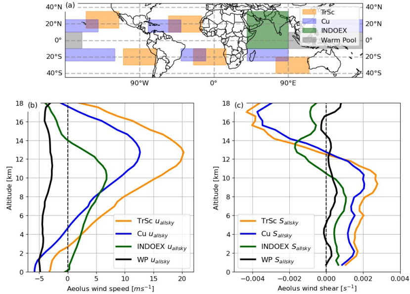
Figure 11: (a) map of the different regions considered. Average (b) wind speed profiles and (c) wind shear profiles retrieved in each region during the year 2020. The wind shear S_{allsky}(z) is computed at each altitude z using the u_{allsky}(z_1) observed 1 km below z and at u_{allsky}(z_2) observed 1 km above z , following Eq. 4.
