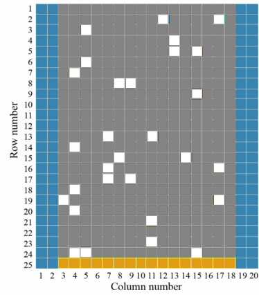
Figure A2. Hot pixel maps corresponding to (a) 14 June 2020 (compare with Weiler et al., 2021), (b) 31 December 2020 (end of our study) and 1 July 2023 (end of Aeolus mission). Hot pixels are denoted in white, regular pixels in gray. Hot pixels are identified by comparing each detector pixel value against its immediate neighbors within the same Mie detector row: pixels exceeding all neighboring values are flagged and counted across all daily orbits. The resulting frequency maps are normalized by their maximum count and thresholded at 0.2, with pixels above this empirical threshold marked as "hot".
