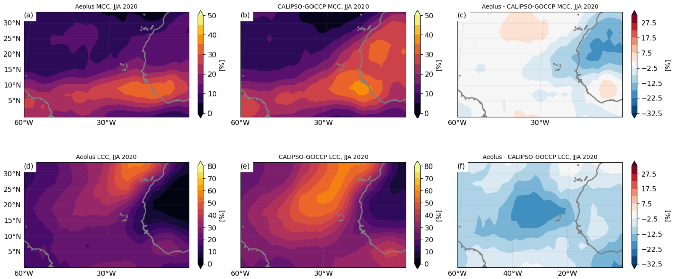
1025 Figure A4. Maps of mid-level (4-8 km) cloud cover (a) Aeolus dataset (b) CALIPSO-GOCCP and (c) the difference Aeolus – CALIPSO-GOCCP for the year 2020. (d), (e) and (f) are the same but for low level clouds (0-4 km).
