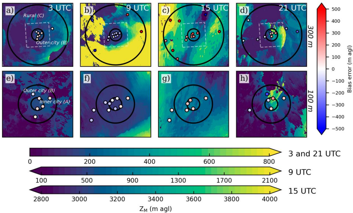
350 Figure 8. As Figure 7, but for 4 August 2022.
