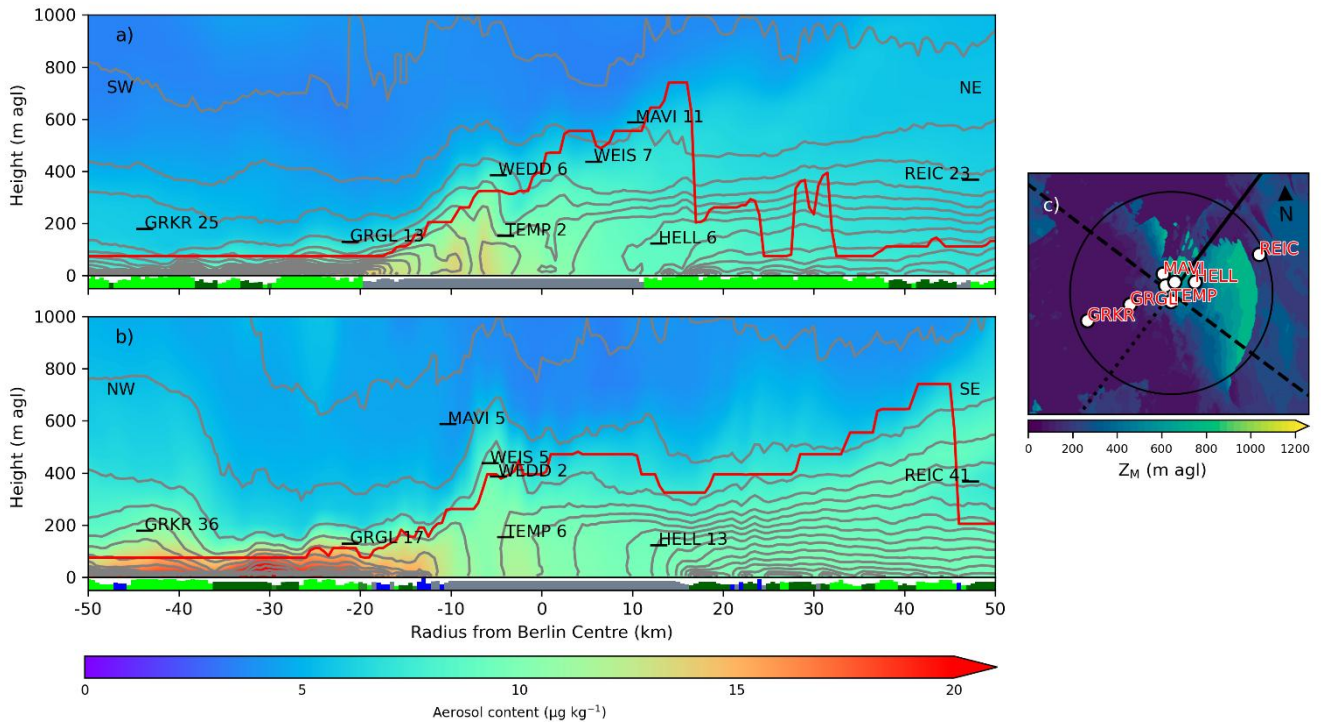
410 Figure 12. As Figure 11 but at 21:00 UTC.
