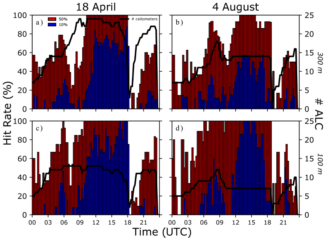
295 Figure 6. Model performance assessed using hit rate (Appendix A2) within 50 % (red) and 10 % (blue) of observed values by model resolution (a-b) 300 m, (c-d) 100 m, for (a, c) 18 April and (b, d) 4 August 2022. Number of ALCs giving data (black line) decreases near sunset because of ALC algorithm (Section 2.2).
