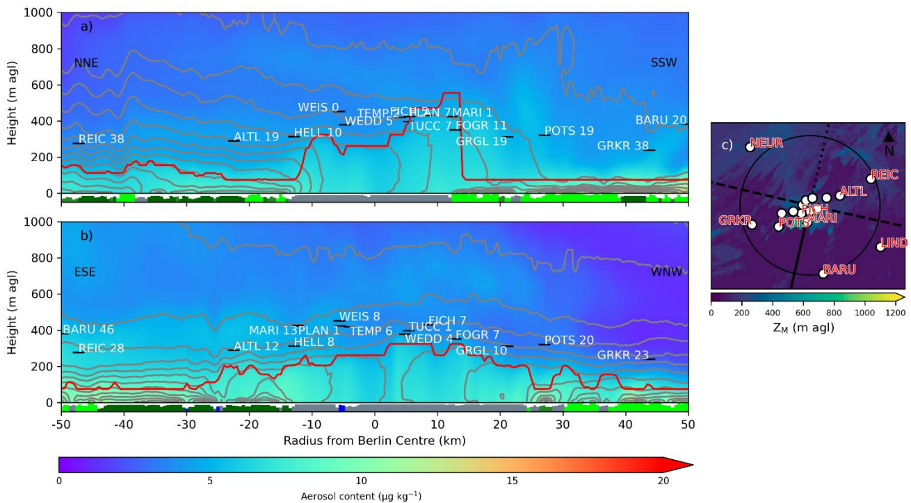
405 Figure 10. As Figure 9 but at 21:00 UTC.
