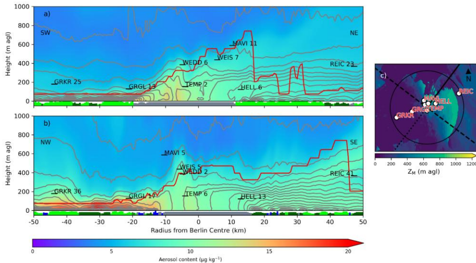
Figure 12. As Figure 11 but at 21:00 UTC.
