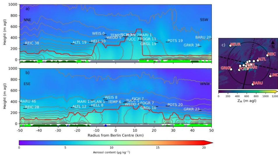
Figure 10. As Figure 9 but at 21:00 UTC.
