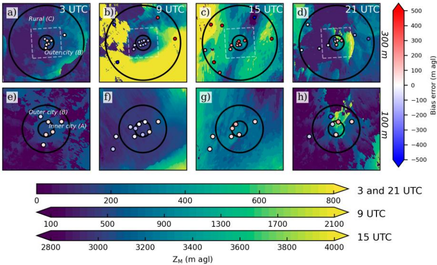
Figure 8. As Figure 7, but for 4 August 2022.
