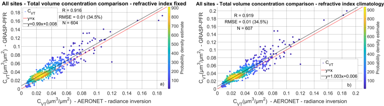
Figure 3: Scatter plot of C_{VT} for the GRASP-AOD from PFR data and AERONET inversions from almucantar scans retrievals from all four locations for a fixed value of refractive index (a) and the use of refractive index climatologies (b). The plots include the correlation factor (R), the root mean square error (RMSE) and the number of observations (N). The colour bar shows the density of the points. We also include the linear fit between the datasets and the y=x line.
