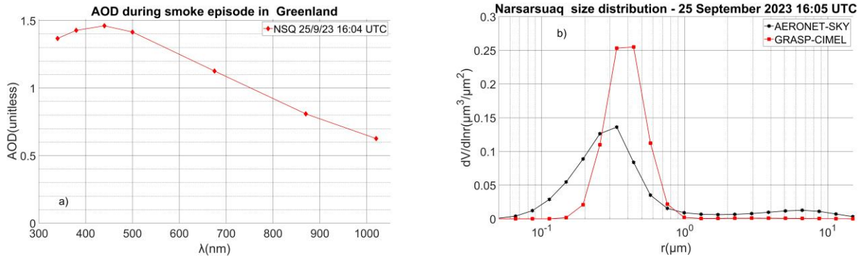
575 Figure 12: (a) CIMEL AOD per wavelength at Narsarsuaq during the record-breaking Canadian wildfires. (b) GRASP-CIMEL size distribution retrievals (red lines) and the closest AERONET size distributions (black lines) at Narsarsuaq (b) during the record-breaking Canadian wildfires.
