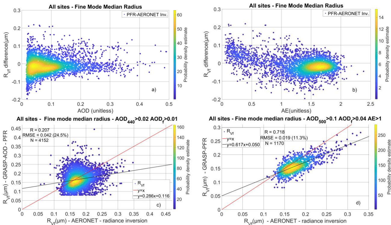
Figure 5: The R_{\text{Vr}} difference between GRASP-AOD from PFR data and AERONET inversions from almucantar scans in relation to AOD (a) and AE (b). Also, scatter plots for R_{\text{Vr}} from GRASP-AOD from PFR data and AERONET inversions (c and d) under different thresholds of AOD and AE in data screening. In panel d) we have increased the AOD, AOD_{\text{f}} and AE thresholds, which improved the comparison. All graphs correspond to all four locations.
