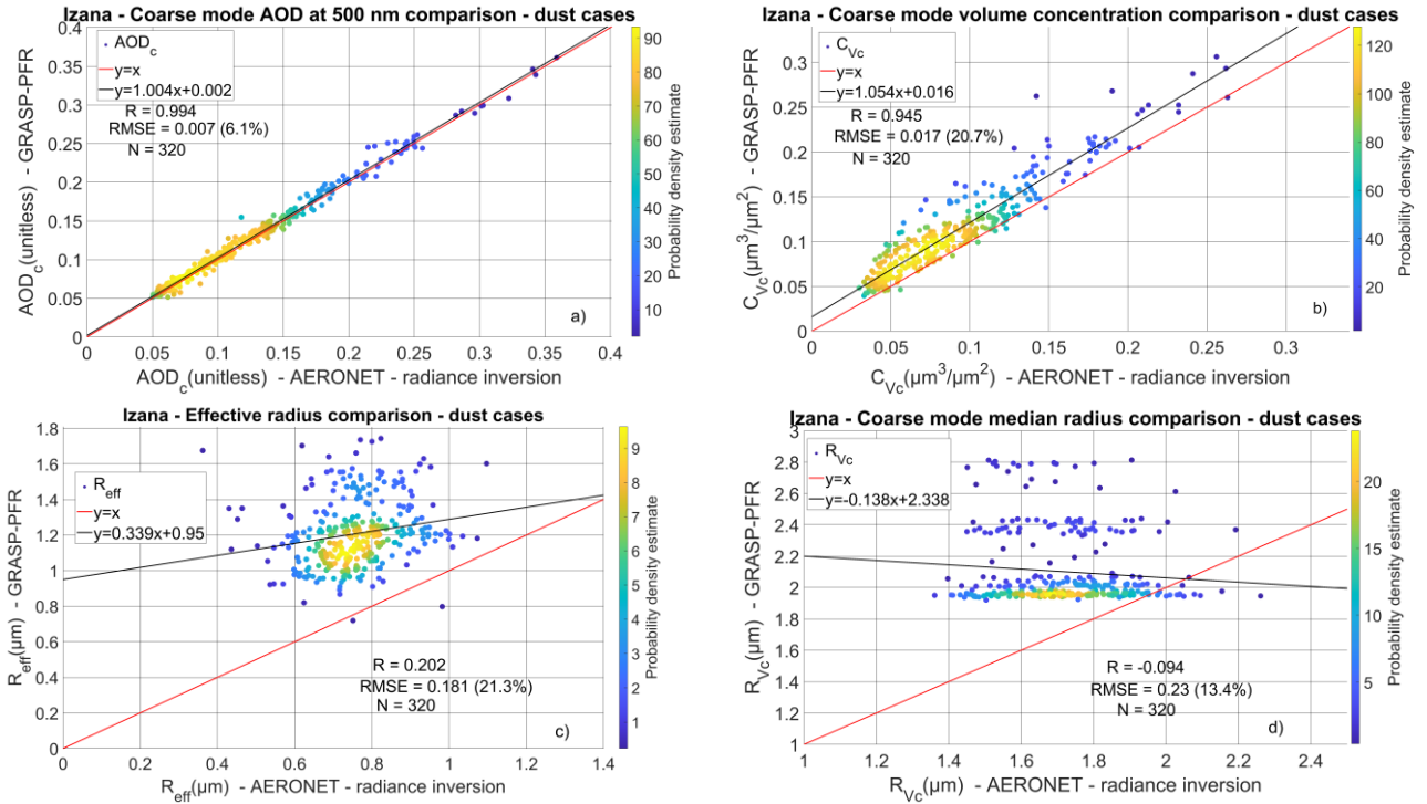
Figure 8: Scatter plot of AOD c (a), C Vc (b), R eff (c) and R Vc (d) for the GRASP-AOD from PFR data and AERONET inversions from almucantar scans retrievals in Izaña corresponding to AE<0.5, AOD c >0.05 and FMF<0.35 (which leads to large dust proportion in the overall aerosols).
