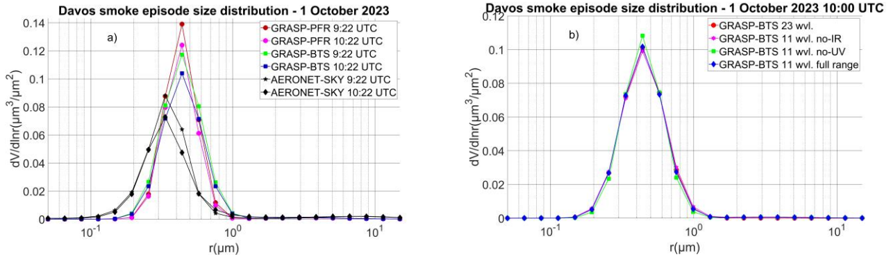
570 Figure 11: The SDs of AERONET (black lines) and GRASP retrievals (coloured lines) from PFR and BTS for two different common measurements (a) and the BTS retrievals for different wavelength selections (b).
