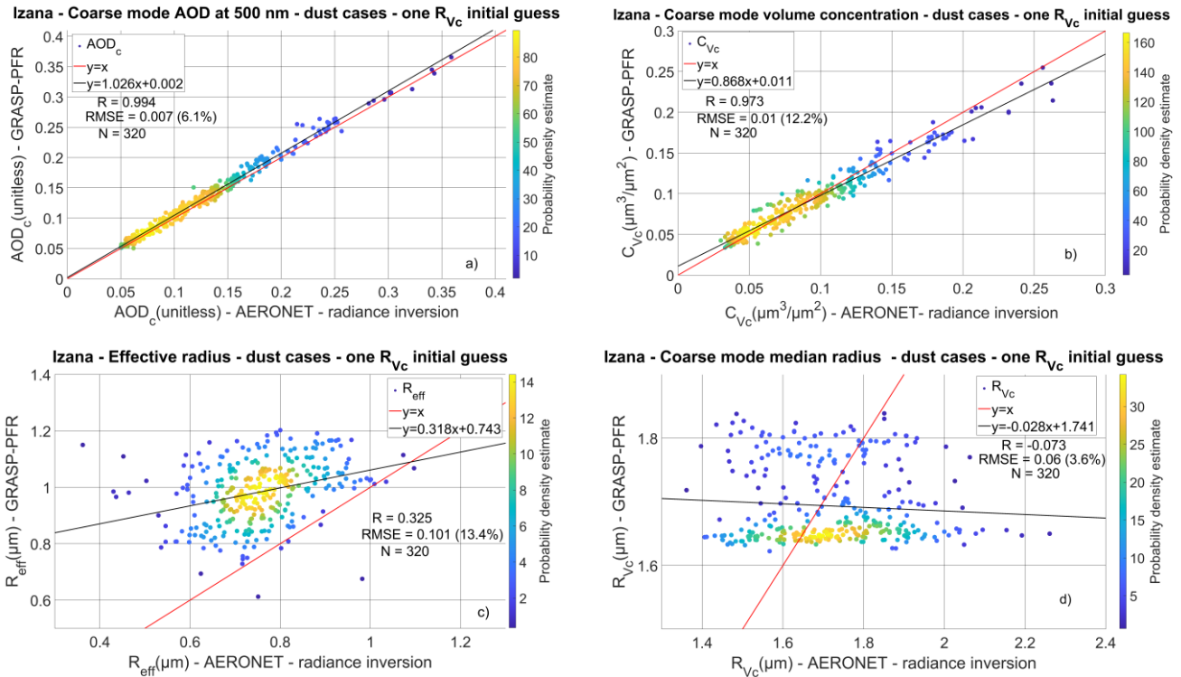
Figure 9: Scatter plot of AOD c (a), C_{Vc} (b), R_{eff} (c) and R_{Vc} (d) for the GRASP-AOD from PFR data and AERONET inversions from almucantar scans retrievals in Izaña corresponding to AE<0.5, AOD c >0.05 and FMF<0.35 and GRASP runs under one initial guess of R_{Vc} .
