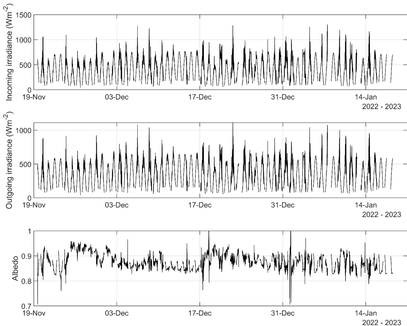
260 Figure 6: Incoming (top panel) and outgoing (middle panel) shortwave irradiance measured by the Eppley radiation station. Albedo (bottom panel) is calculated as the ratio of incoming to outgoing irradiance. Data corresponding to solar zenith angles greater than 80° have been excluded to minimize potential biases due to low sun angles. Albedo values > 1.0 created by broken cloud conditions on 18 Dec and 1 Jan are also filtered out as well as respective irradiance values.
