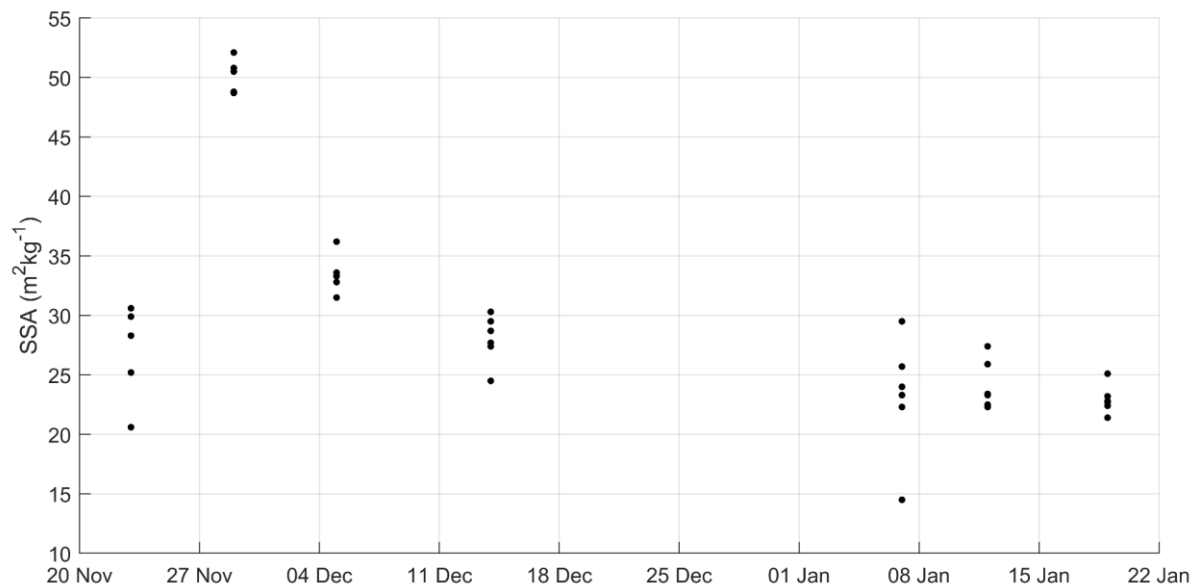
365 Figure 11: SSA measured at the snow surface at the AWS5 site.
