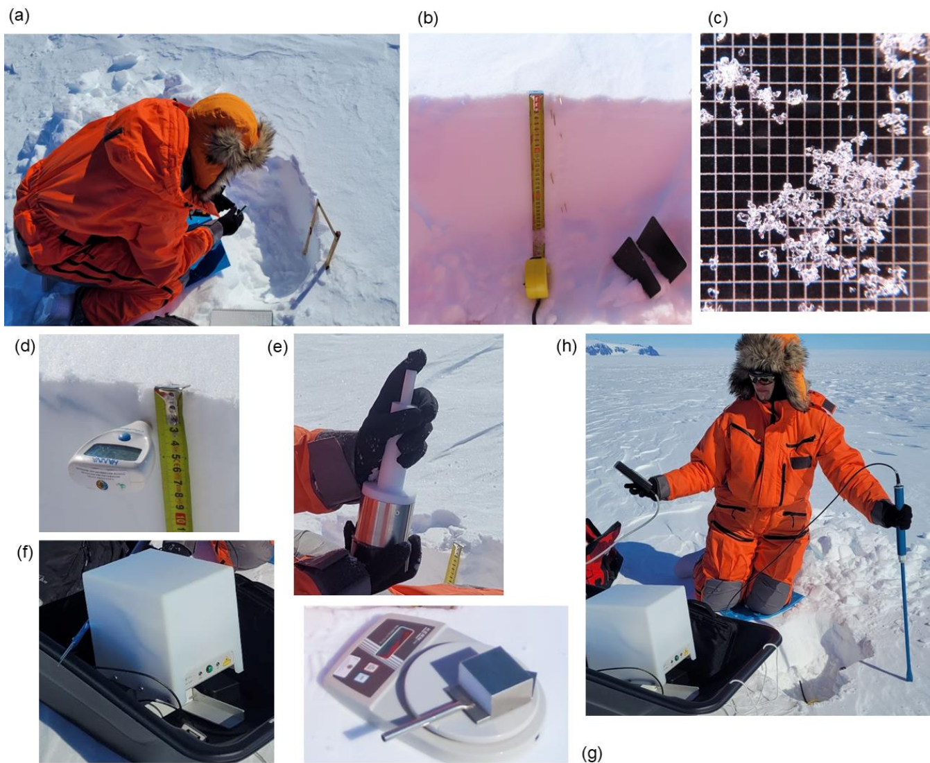
355 Figure 9: a) Overview of snow pit work, b) example of profile photo, c) example of grain macrophoto, d) temperature measurement, e) snow sampling for IceCube SSA measurement, f) IceCube instrument, g) density measurement, h) SnowFork measurement from the surface.
