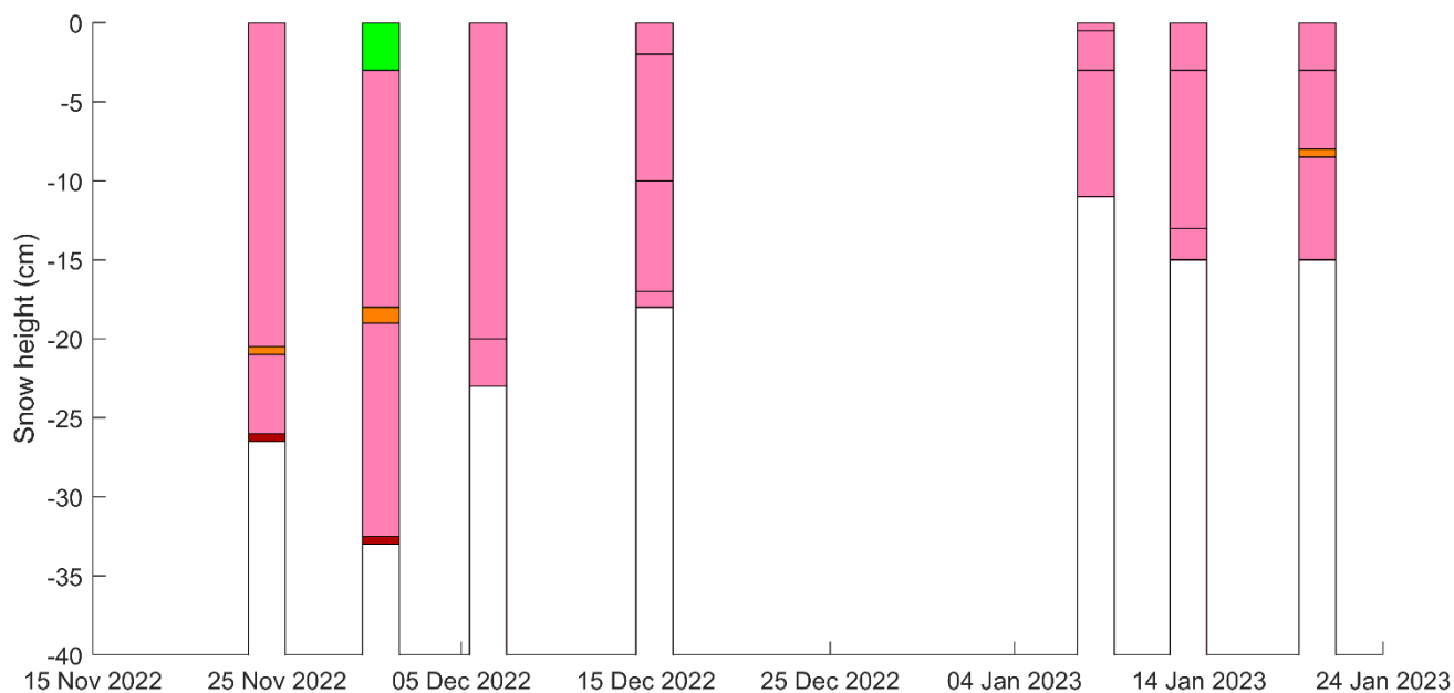
360 Figure 10: Stratigraphy for the topmost snowpack. Following grain types were observed: rounded grains (pink), crust or ice layer (red), crust and rounded grains (orange) and precipitation particles (green). Snow depth 0 cm is the surface. Time period in x-axel for each layer structure is two days.
