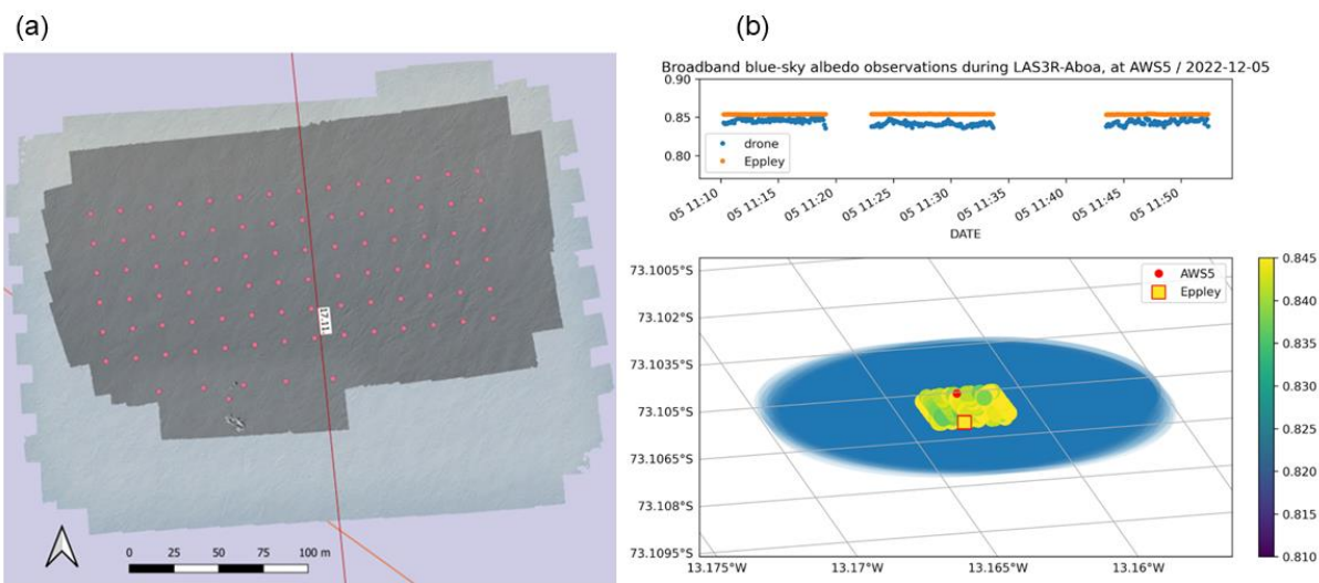
260 Figure 7: a) Example of hyperspectral camera spectral radiance data in channel 501 nm on 23 Nov 2022. b) Example of CM11 data on 5 Dec 2022. Top panel presents broadband blue-sky albedo from the drone and Eppley in UTC time. In the lower panel, spatial variability of CM11 albedo is shown and the blue area presents the field of view of the CM11 instrument at the flight altitude.
