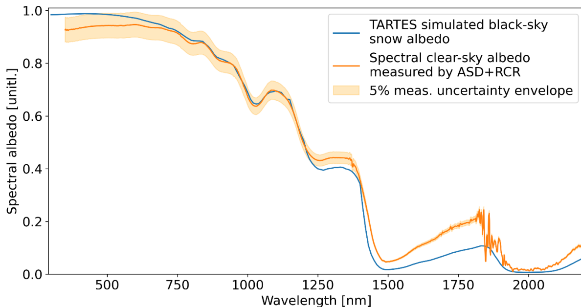
265 Figure 8: Spectral albedo measured with ASD spectroradiometer using an alternation of RCR foreoptic pointing up- and downward on Jan 5, 2023, a clear-sky day and simulated black-sky snow albedo with TARTES model with inputs consistent with observed conditions.
