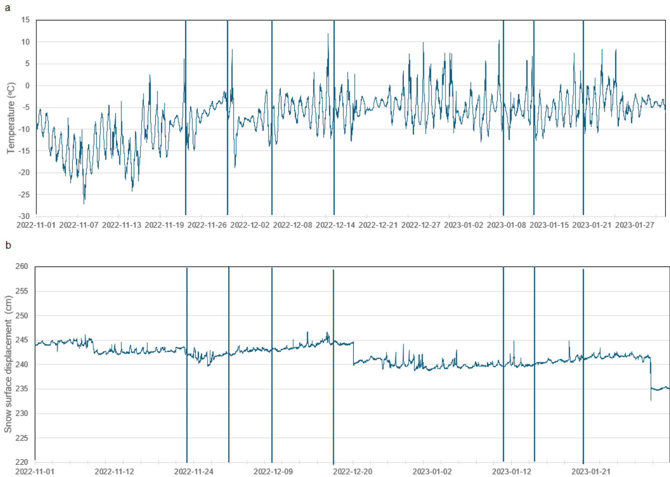
Figure 15: a) Air temperature and b) sensor distance from snow surface during the season 2022-23. Measurement days are marked with vertical lines.
