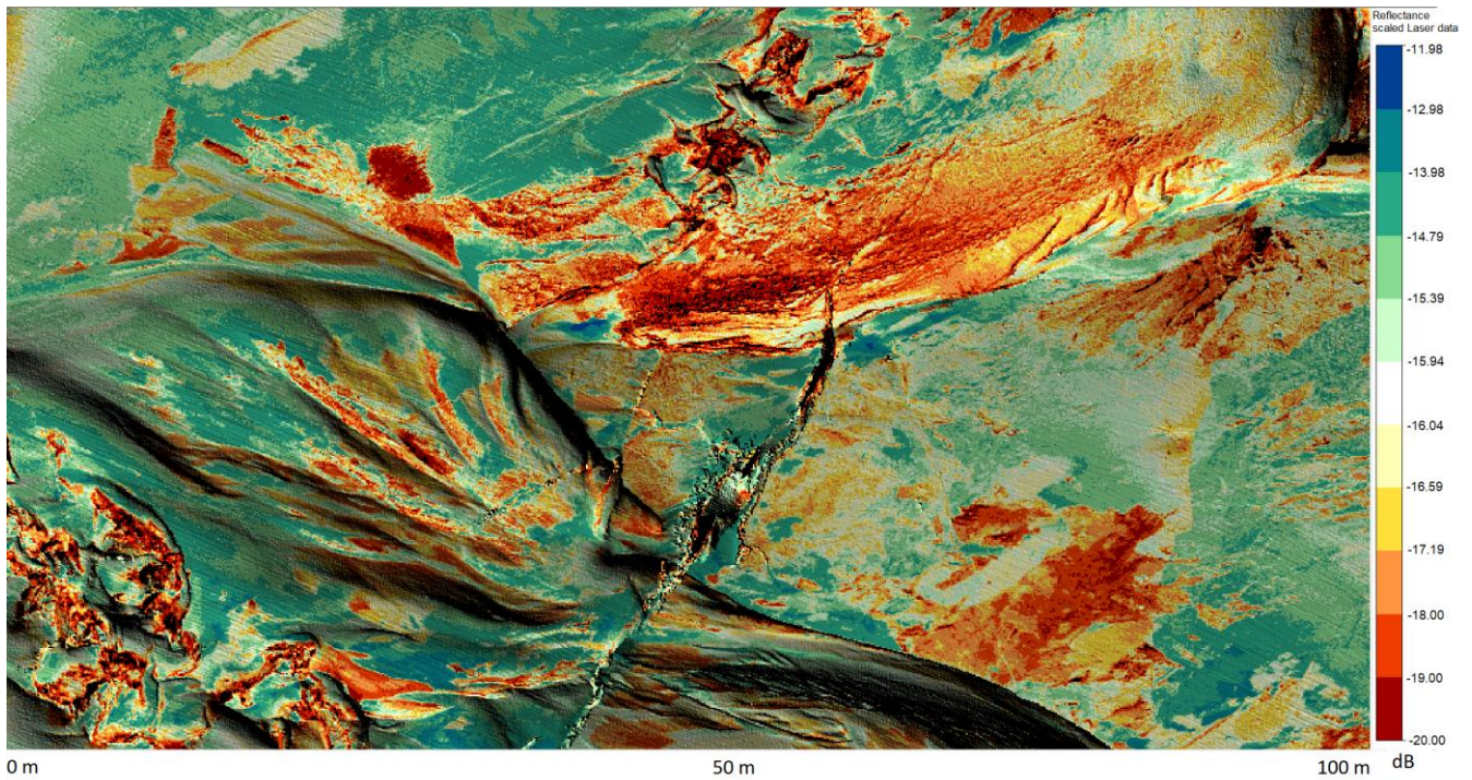
190 Figure 4: An example of the laser scanning data at the Riiser-Larsen shelf-ice shows the rugged transition zone with sea ice and wind erosion patterns. Colouring indicates the reflectivity of the surface at 1550 nm. Image width approximately 100 m, pixel size 10 cm.
